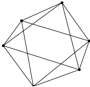
Figure 11.2.1. A graph.
