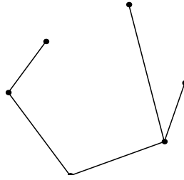
Figure 11.2.2. A tree.
