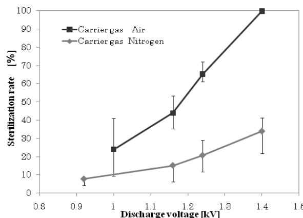
Figure 11: Comparison of sterilization rate of B. subtilis with air and nitrogen plasma.
