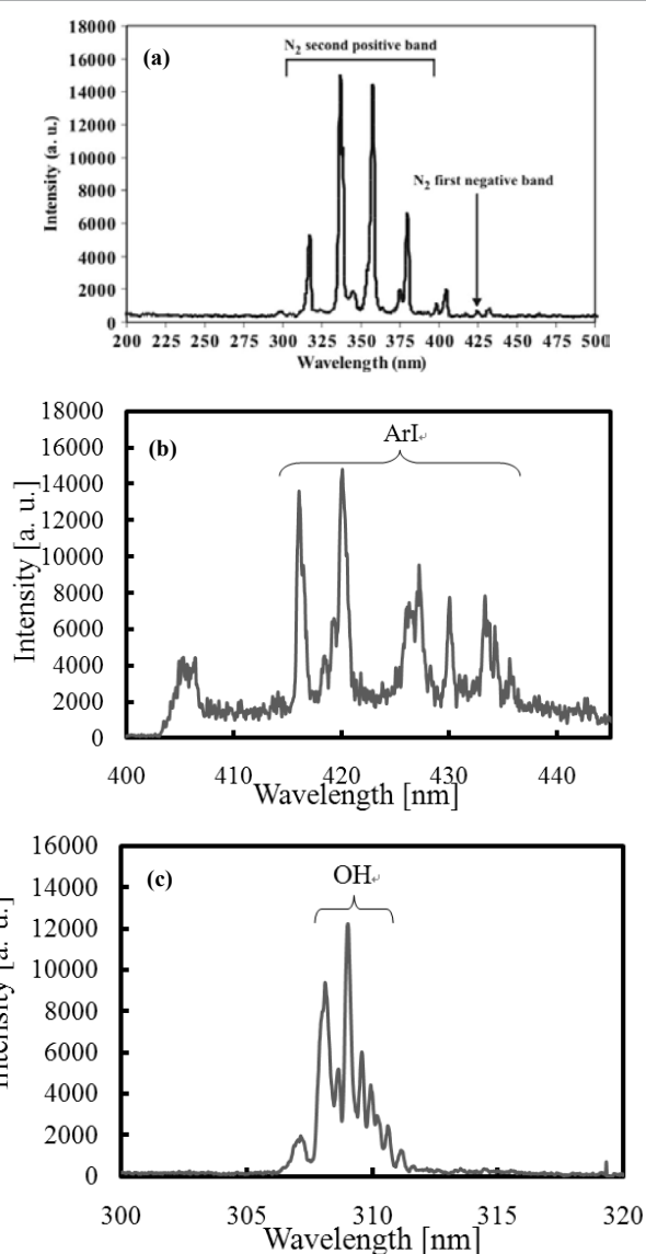
Figure 14: Emission spectrum of microplasma: N 2 second positive band system and N 2 first negative band system from discharge in nitrogen (a) excited Ar atoms (b) and excited OH radical.
