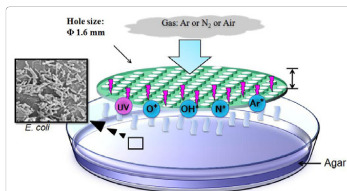
Figure 2: Schematic image of microplasma electrodes for sterilization and disinfection of surface colonized bacteria.
