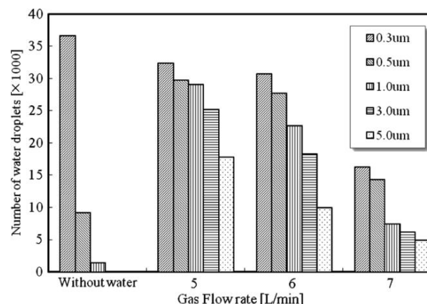
Figure 7: Size distribution of water particles generated in by the nebulizer at gas flow rates of 5, 6, and 7 L/min.
