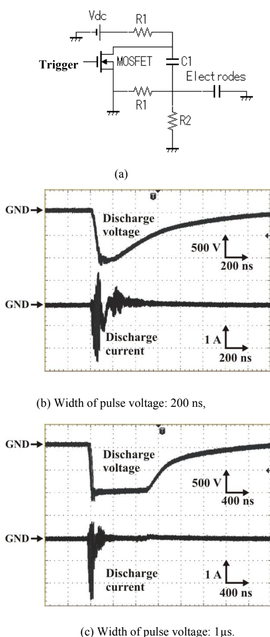
Figure 6: An example of a pulse circuit with the MOSFET switch (a); discharge voltage and corresponding discharge current by a pulse power circuit (b) and (c).
