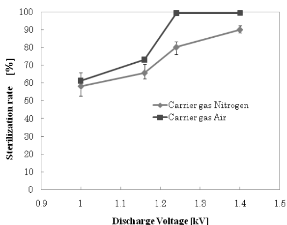
Figure 10: Comparison of sterilization rate of E. coli with air and nitrogen plasma.
