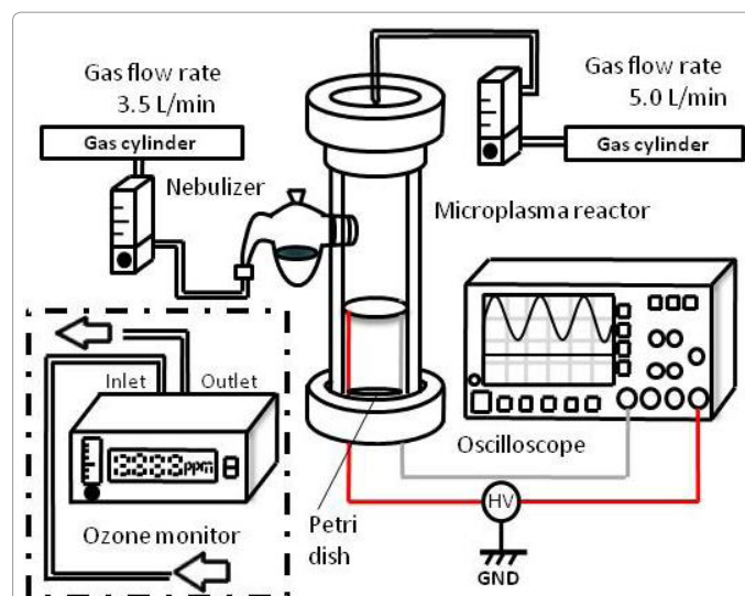
Figure 3: An experimental setup for sterilization and disinfection of airborne bacteria.
