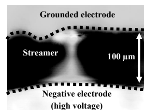
(c). Vd= 1.4 kV, shutter opening 30 sec., gap distance was set at 100 \mu\text{m} , and streamer diameter was about 20 \mu\text{m} , Gas composition was 1% \text{N}_2 , and 99% Ar.
