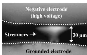
(b). Vd= 1 kV, shutter opening 30 sec., gap distance was set at 30 \mu\text{m} , and streamer diameter was about 10 \mu\text{m} , Gas composition was 1% \text{N}_2 , and 99% Ar.
