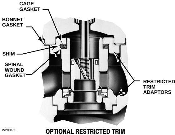
Figure 3-31. Adapter Method for Providing Reduced Flow Capacity
