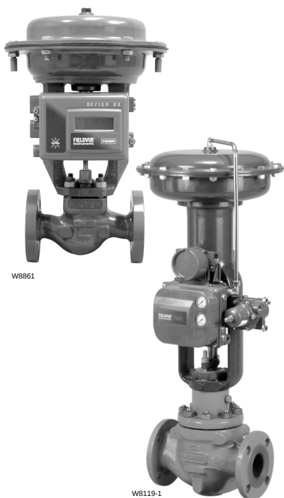
Figure 4-1. Modern Control Valves Utilizing Digital Valve Controllers
