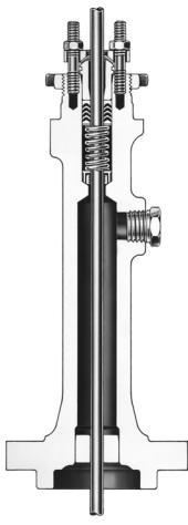
Figure 1-5. Extension Bonnet
