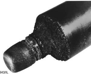
Figure 5-7. Typical Appearance of Cavitation Damage
