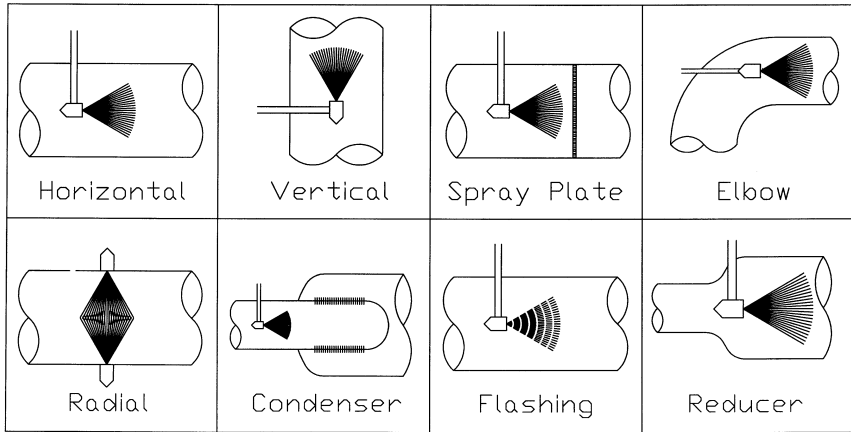
Figure 7-1. Desuperheater Installations
