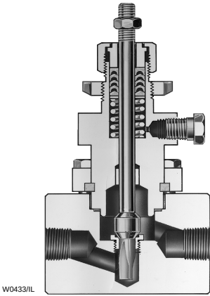
Figure 3-3. Bar Stock Valve Bodies
