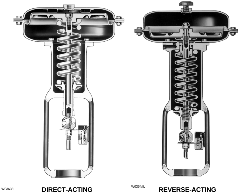
Figure 3-32. Diaphragm Actuators
