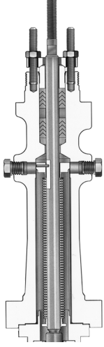
Figure 1-6. Bellows Seal Bonnet
