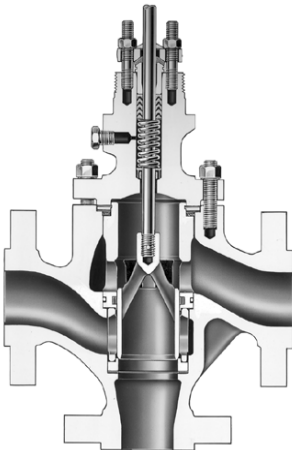
Figure 1-11. Three-Way Valve with Balanced Valve Plug
