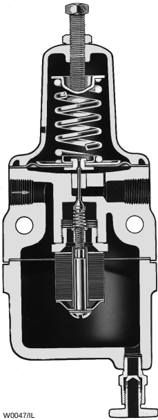
Figure 4-9. Supply Pressure Regulator with Filter and Moisture Trap
