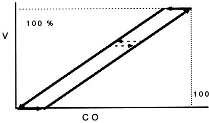
Figure 1-1. Process Dead Band
