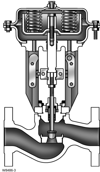
Figure 3-33. Field-Reversible Multi-Spring Actuator
