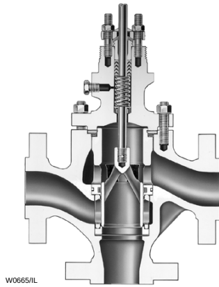
Figure 3-8. Three Way Valve with Balanced Valve Plug
