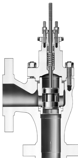
Figure 3-2. Flanged Angle-Style Control Valve Body
