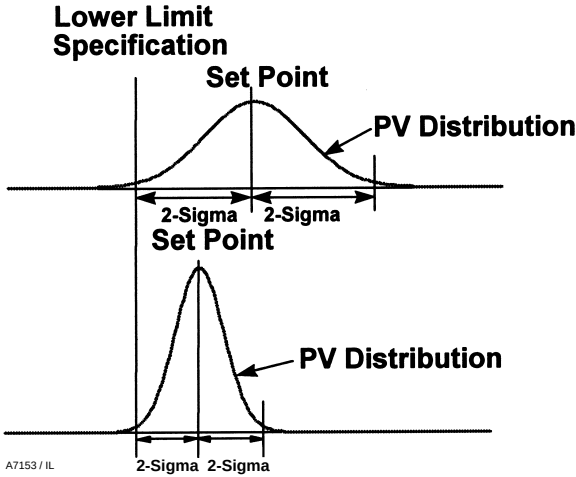
Figure 2-1. Process Variability
