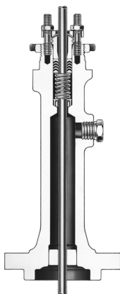
Figure 3-16. Extension Bonnet
