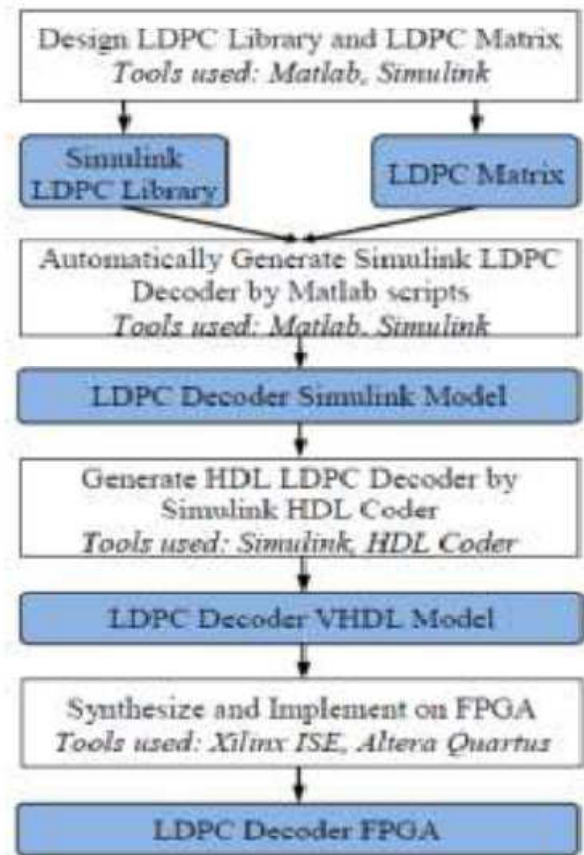
Fig 1. Automated LDPC design flow
