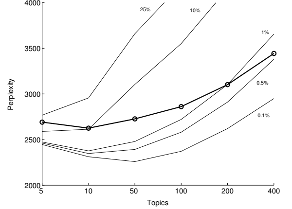
Figure 5: Perplexity of the 102 single-authored test documents from the NIPS collection, conditioned both on the correct author and authors ranked by perplexity using the model, as described in the text.
