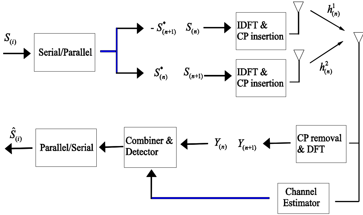
Fig 1: STBC-OFDM Block Diagram
