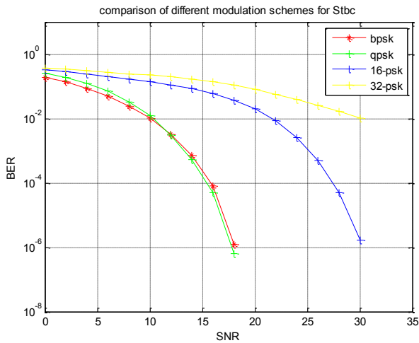
Fig 2: Performance comparison of 2*2 STBC-OFDM with M-PSK Modulation
