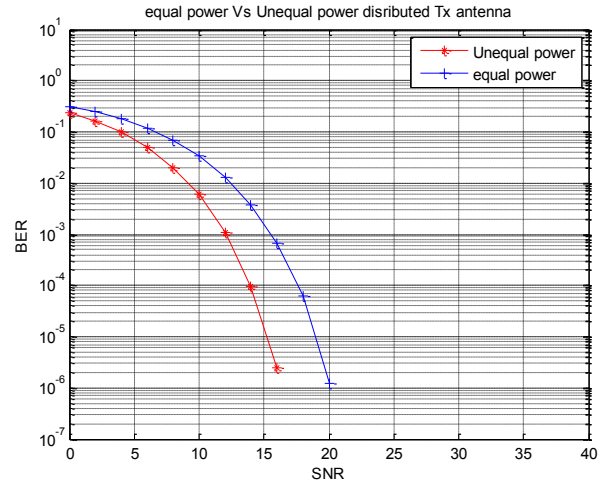
Fig 3: Performance comparison of 2*2 STBC-OFDM with equal and unequal power distributions
