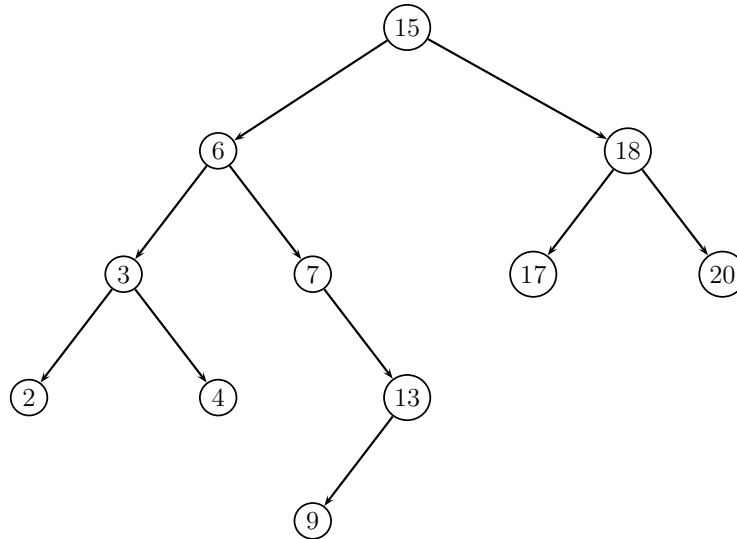
Fig. 4.32 A binary search tree
