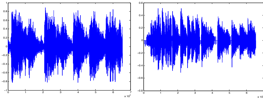
Fig. 3.28 The signal “handel” and its Haar transform
