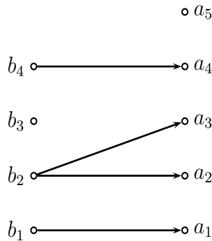
Fig. 3.11 The inverse, G^{-1} , of the graph of Figure 3.3
