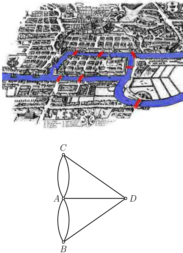
Fig. 8.11 The seven bridges of Königsberg and a graph modeling the Königsberg bridge problem
