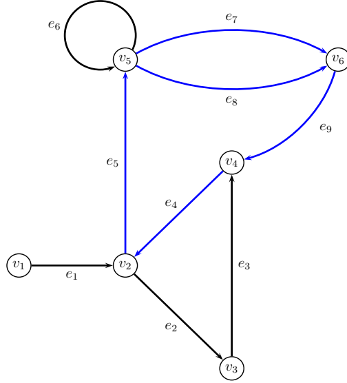
Fig. 4.8 A path in a directed graph G_1
