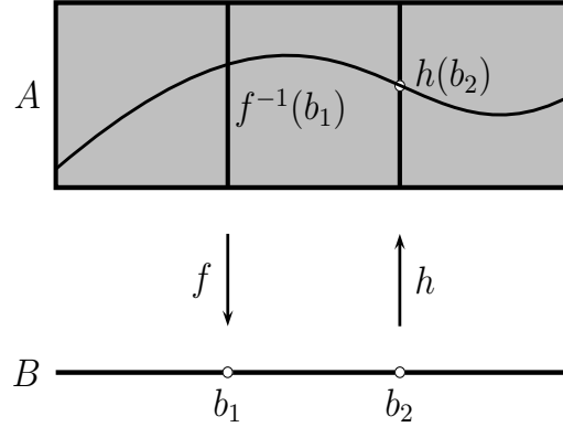
Fig. 3.16 A section h of a surjective function f .
