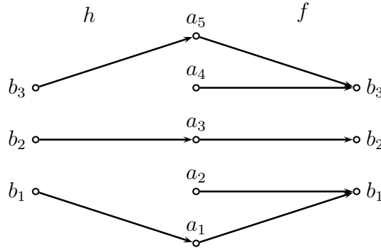
Fig. 3.9 A function f with a right inverse h .
