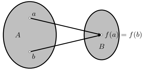
Fig. 3.12 A noninjective function
