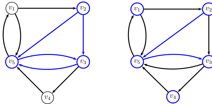
Fig. 4.16 An induced subgraph and a partial graph
