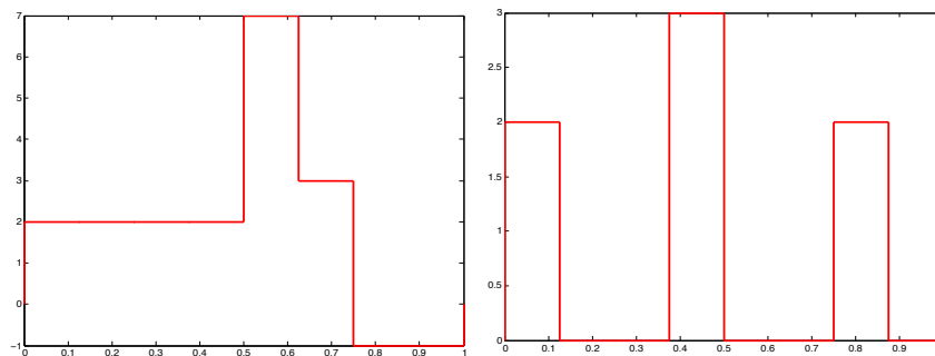
Fig. 3.26 A signal and its Haar transform
