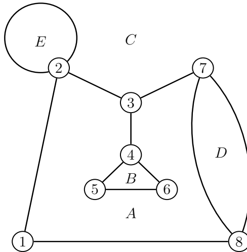
Fig. 8.34 A planar graph and its faces
