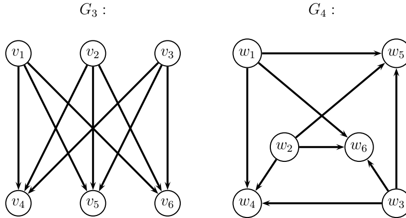
Fig. 4.7 Two isomorphic graphs, G_3 and G_4
