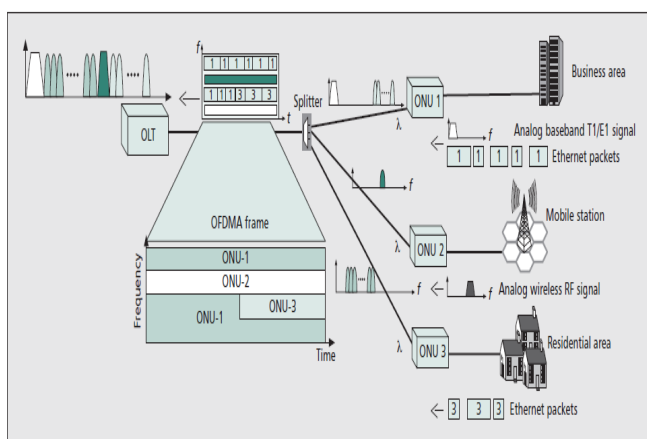
Figure 5: OFDMA PON architecture for delivery of heterogeneous services.
