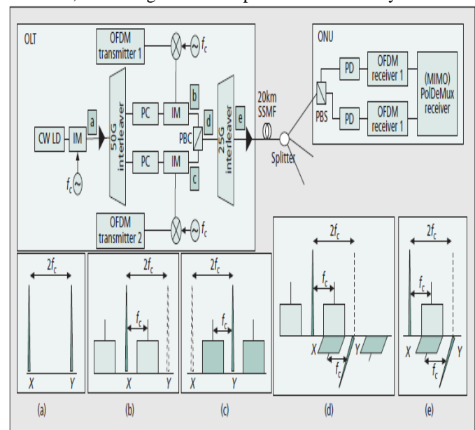
Figure 6: Proposed POLMUX-DD architecture (top) and frequency domain description of POLMUX-OFDM signal generation (bottom).
