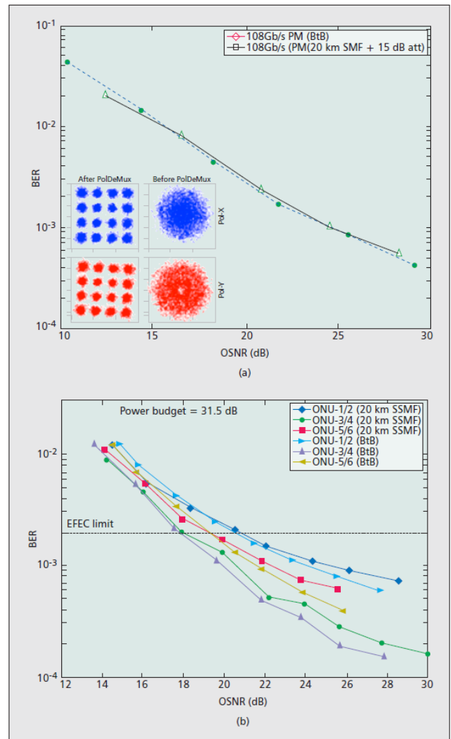
Figure 8: a) Experimental BER results for 108 Gb/s downstream OFDMA-PON; b) experimental BER results for 108 Gb/s upstream OFDMA-PON.
