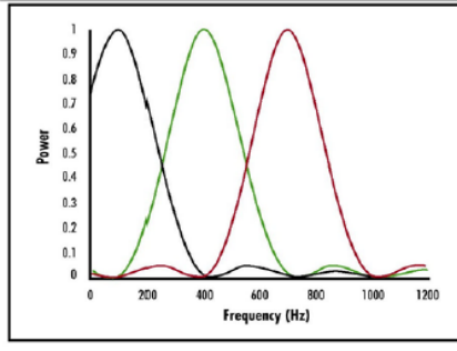
Figure 1: Orthogonality of Sub-carriers
