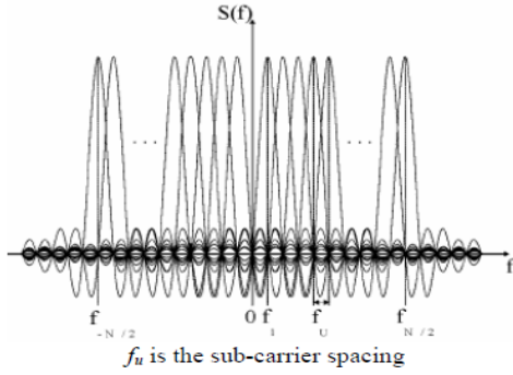
Figure 2: OFDM sub carriers in the frequency domain
