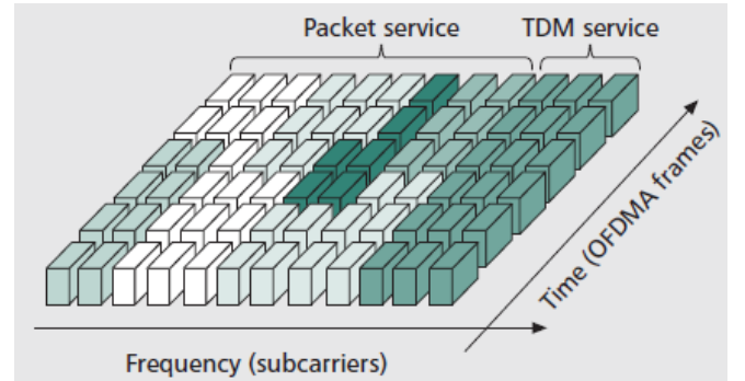
Figure 4: Frequency and Time domain partitioning of an OFDMA frame
