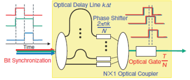
Figure 3: Optical Circuit for Discrete Fourier Transform
