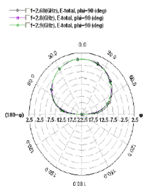
Fig. 5(b): Elevation pattern gain display of final patch antenna in lower frequency band
