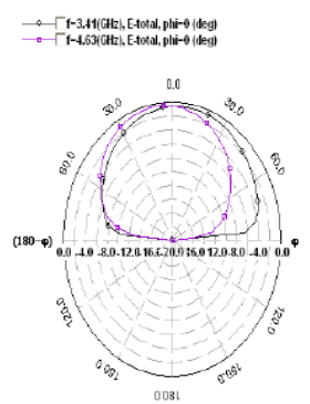
Fig. 5(c): Elevation pattern gain display of final patch antenna median frequency band
