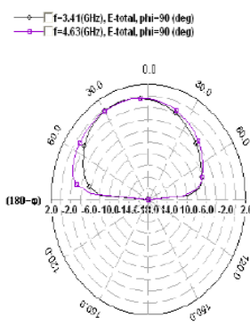
Fig. 5(d): Elevation pattern gain display of final patch antenna median frequency band
