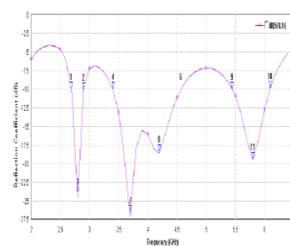
Fig. 2(a): Simulated variation in reflection coefficient of antenna with frequency
