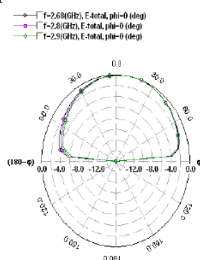
Fig. 5(a): Elevation pattern gain display of final patch antenna in lower frequency band
