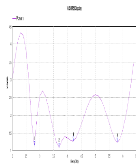
Fig 3(a) simulated variations in VSWR with frequency
