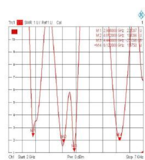
Fig3(b) Measured Variations in VSWR with frequency
