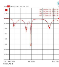
Fig. 2(b): measured variation in reflection coefficient of antenna with frequency
