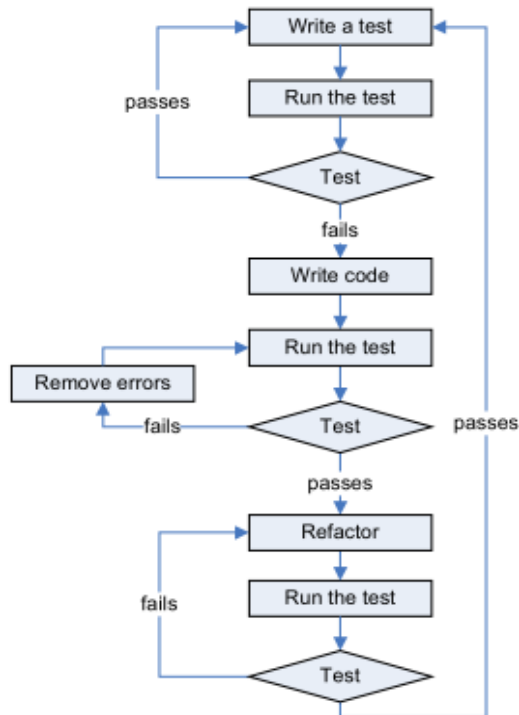
Figure 2: TDD Flowchart
