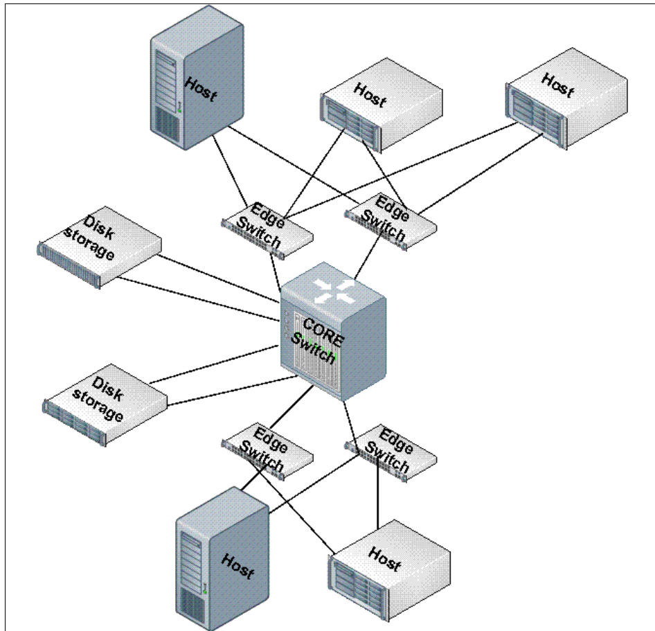
Figure 5-9 Core-edge topology
