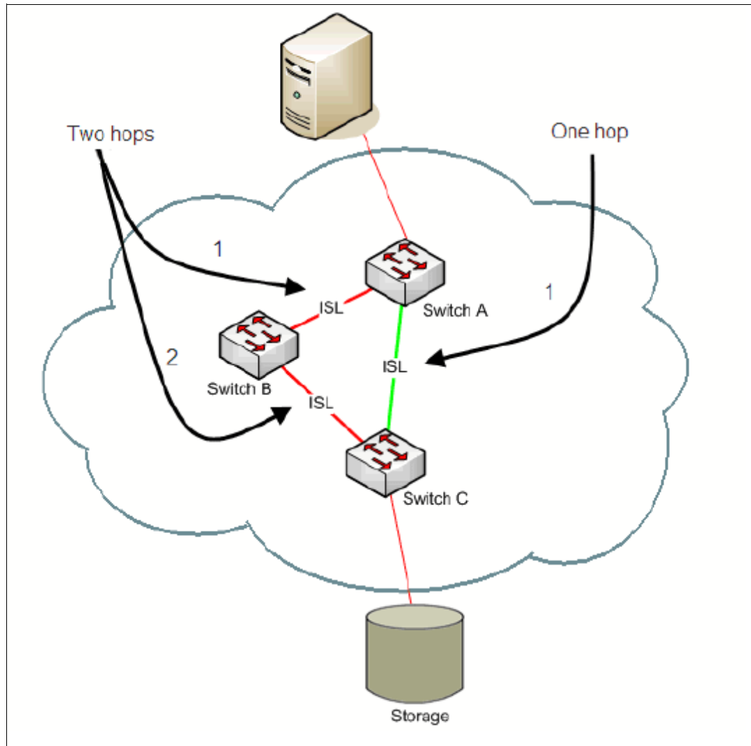
Figure 7-18 Hops example
