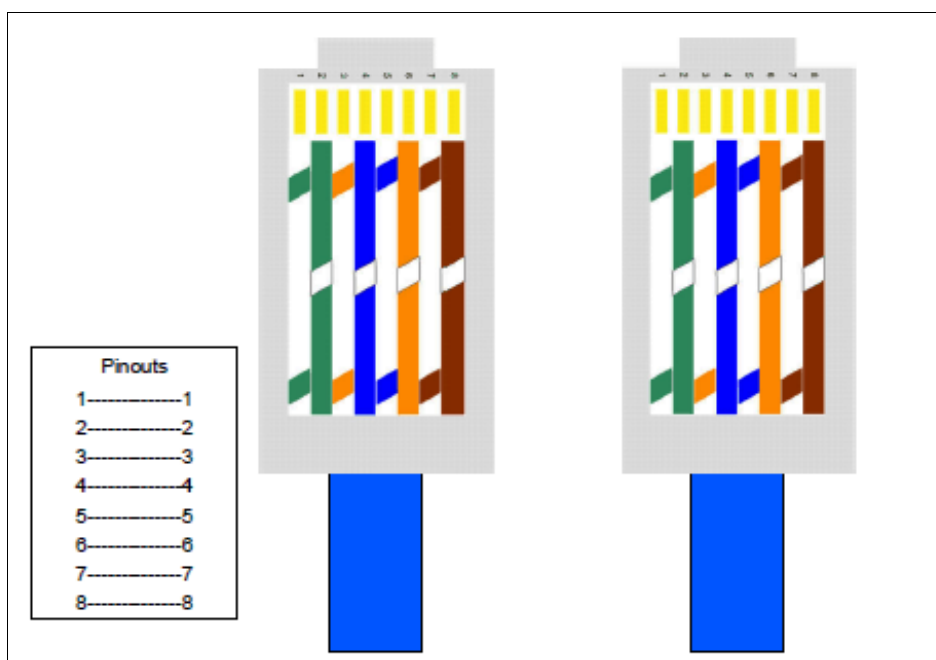
Figure 7-10 Straight-through Ethernet cable
