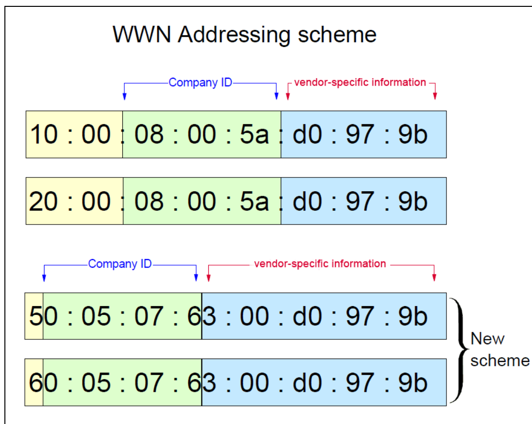
Figure 5-15 Worldwide name (WWN) addressing scheme
