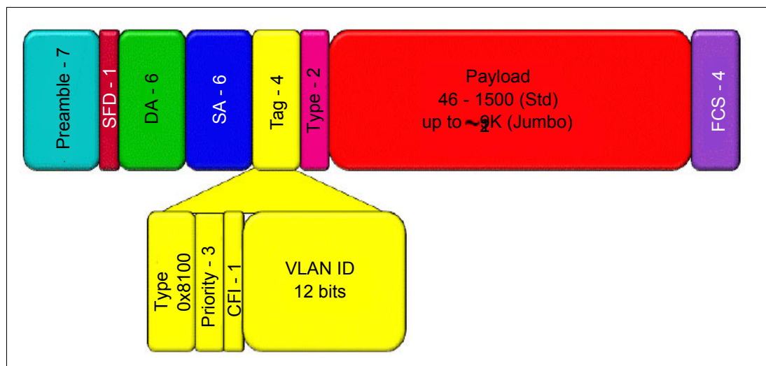
Figure 4-7 IEEE 802.1p/q tagged Ethernet frame
