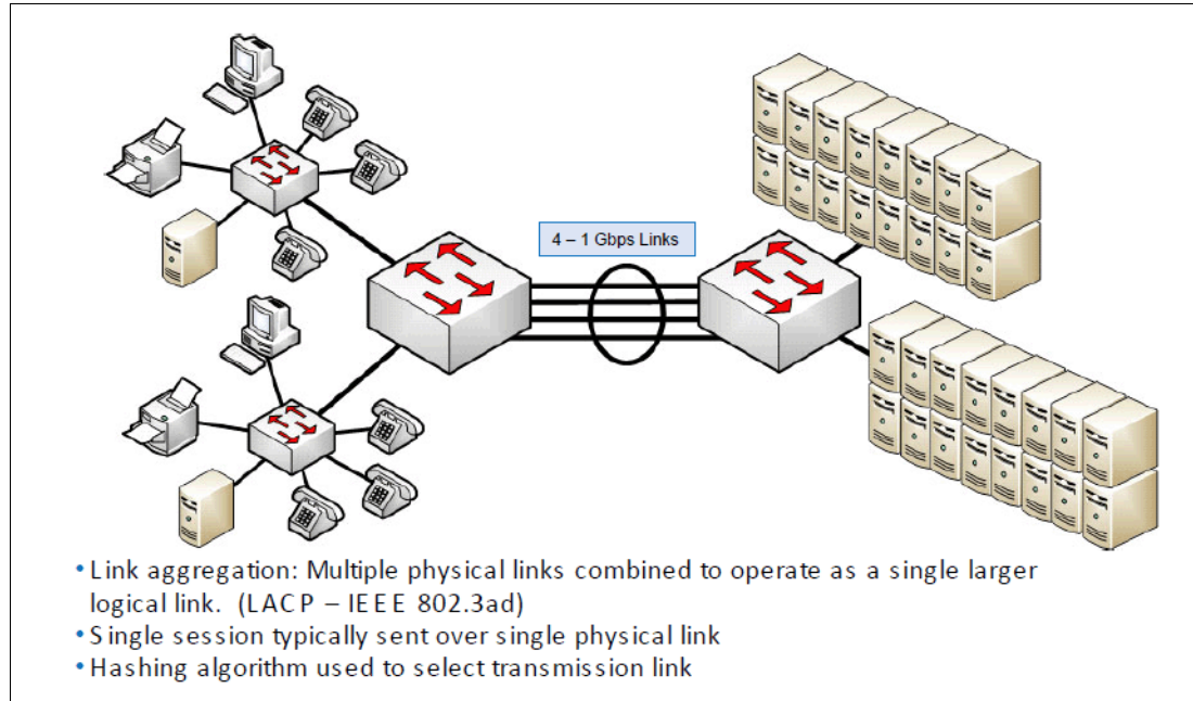
Figure 4-9 Link aggregation
