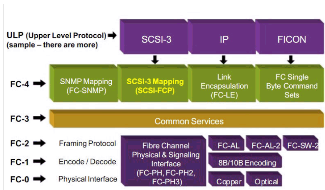
Figure 2-4 Fibre Channel model overview
