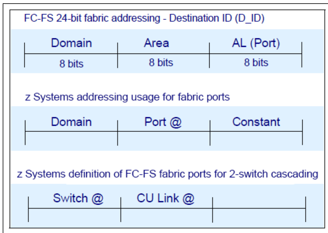
Figure 5-25 FICON addressing for cascaded directors
