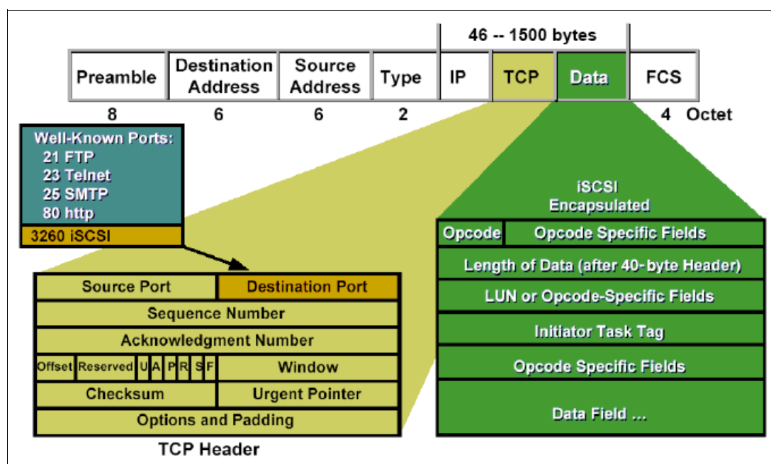
Figure 4-12 iSCSI packet format
