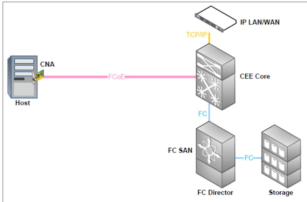
Figure 10-8 Fabric convergence
