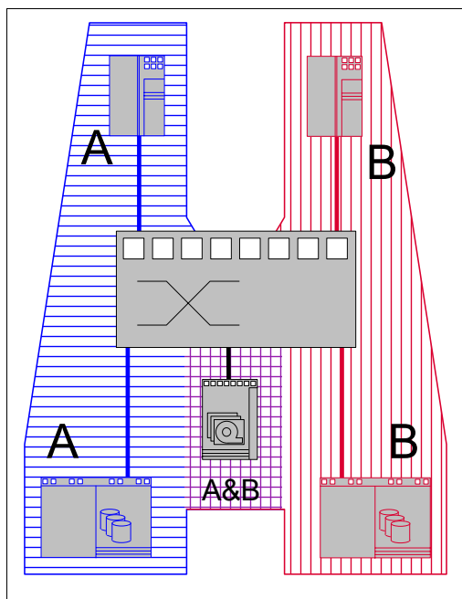
Figure 5-31 Zoning example
