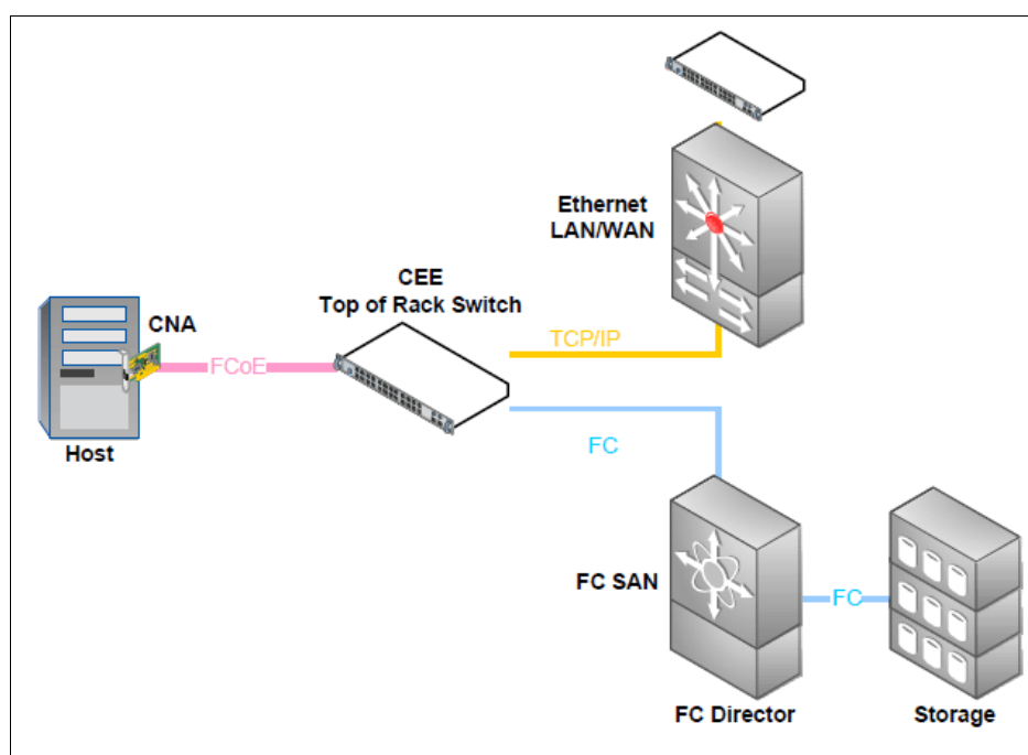
Figure 10-7 Access layer convergence
