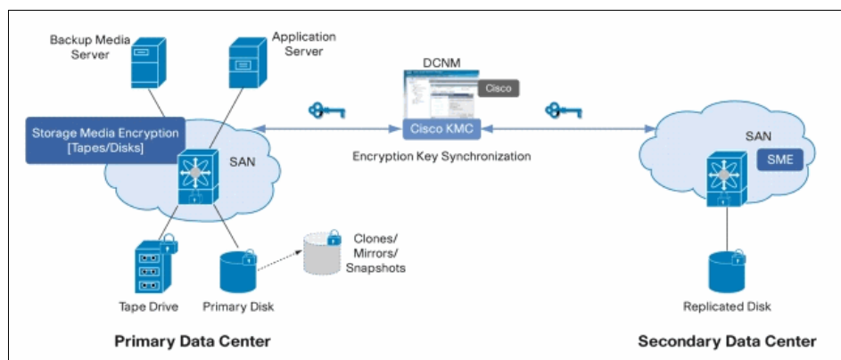
Figure 9-6 SME architecture
