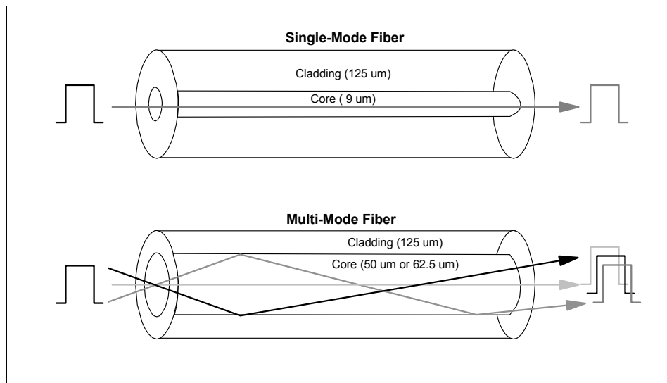
Figure 3-7 Cable types
