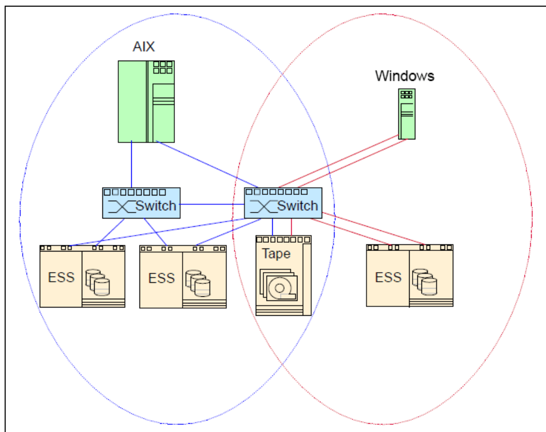
Figure 5-30 Zoning
