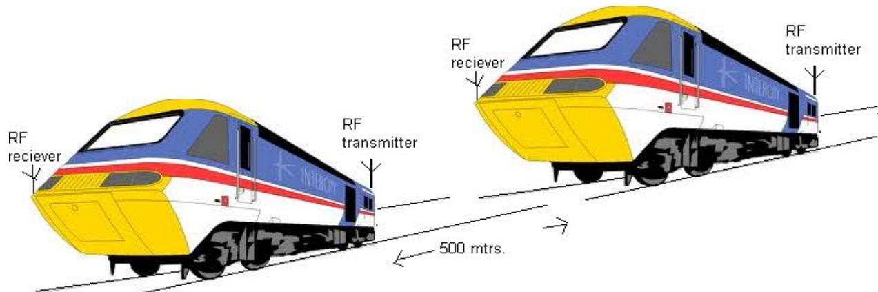
Fig. 1.2 Train Setup
