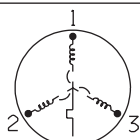
MOTOR WINDING CONNECTION 2-94 052-1199-00
