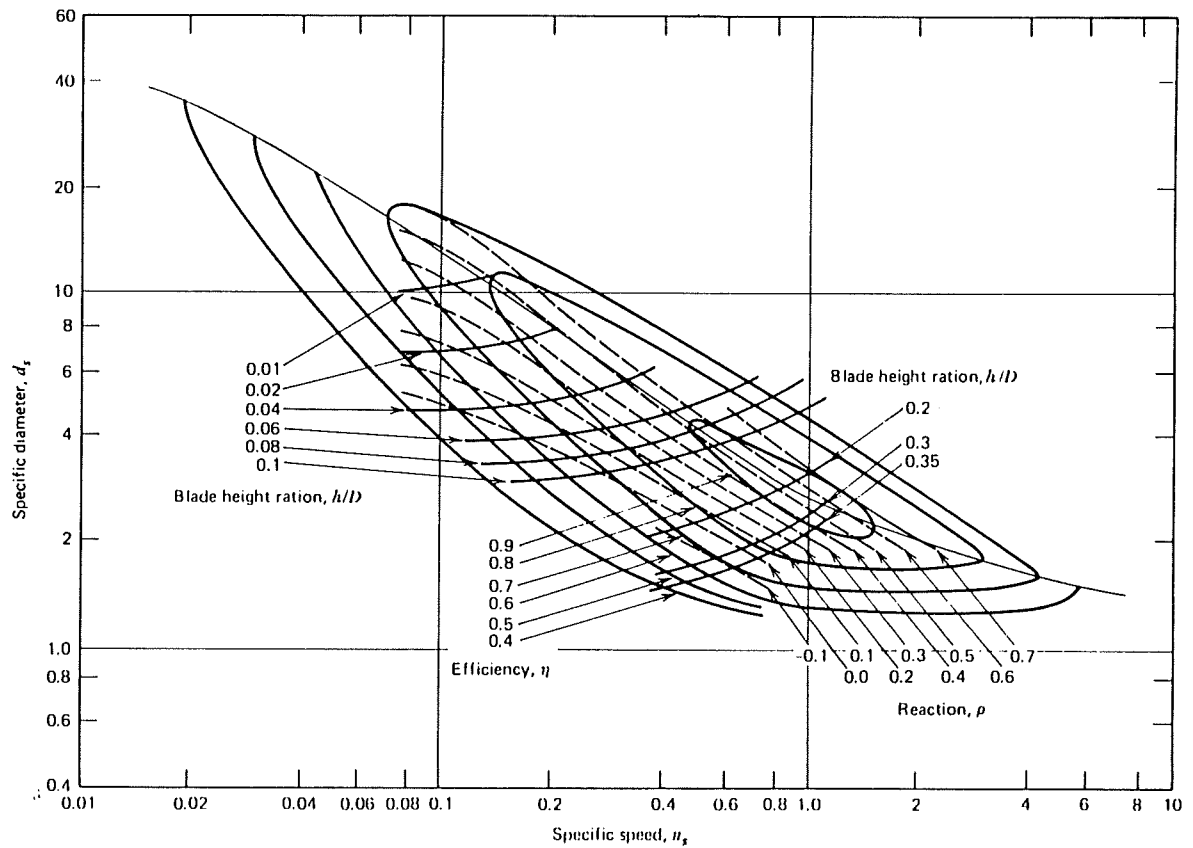
n_s, D_s diagram for turbines calculated for minimum loss coefficients
