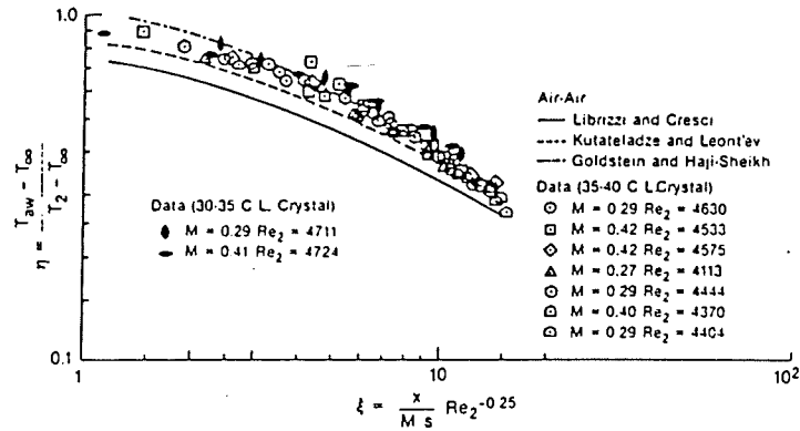
Film cooling effectiveness for air-air.
