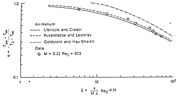
Film cooling effectiveness for air-helium.
