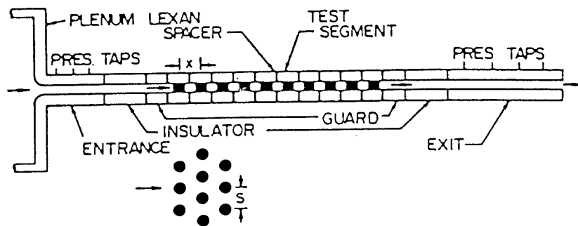
Test section arrangement
