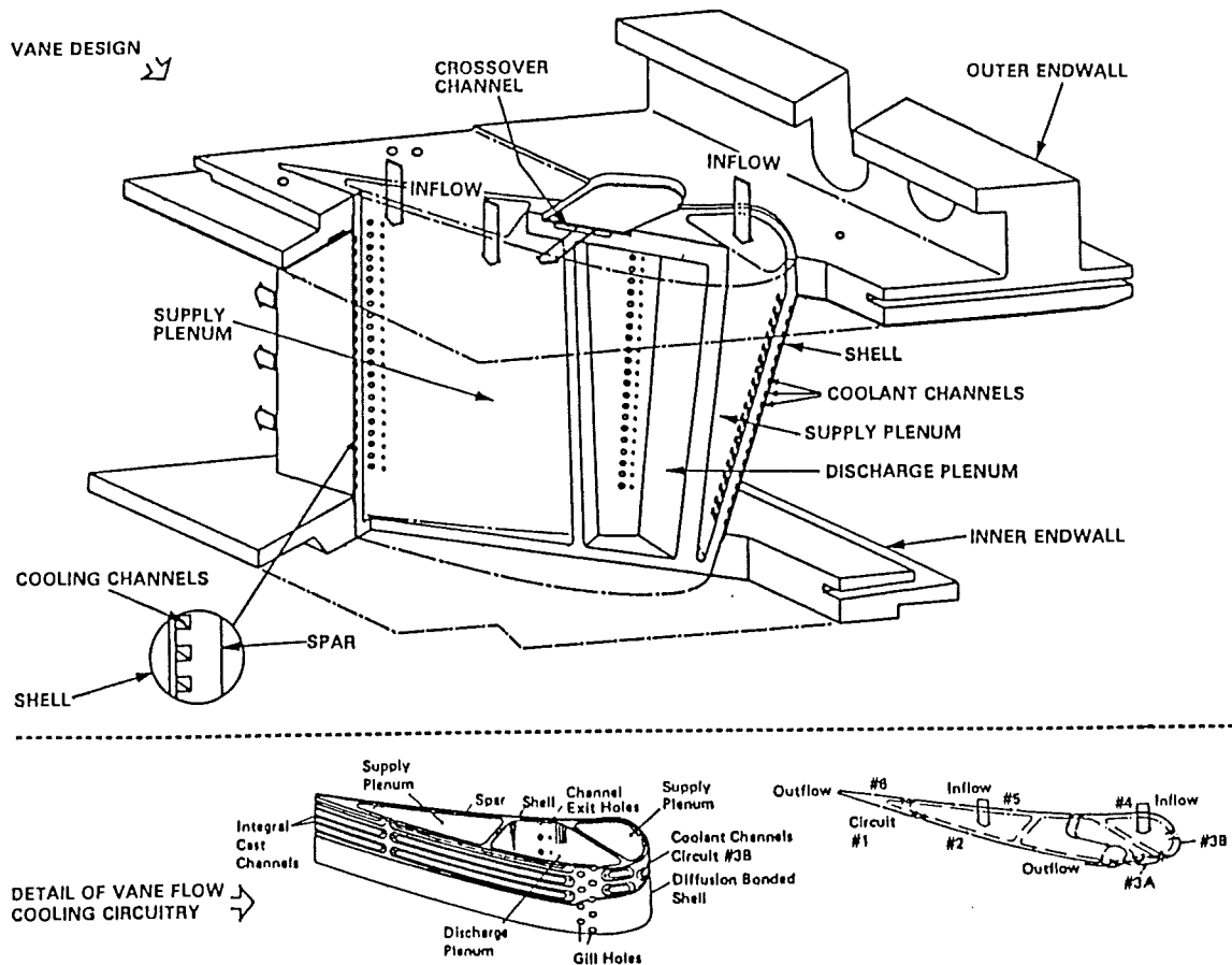
CONCEPTUAL DESIGN OF THE SHELL-SPAR ADVANCED COOLED VANE
