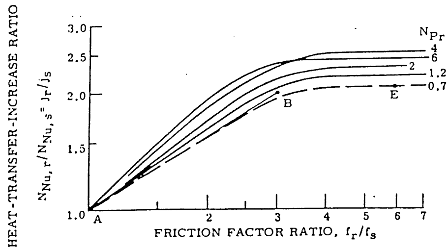
HEAT-TRANSFER EFFECT OF SAND-GRAIN ROUGHNESS AS AFFECTED BY PRANDTL NUMBER, FOR REYNOLDS NUMBERS FROM 10,000 TO 200,000 (AND PERHAPS MORE)
