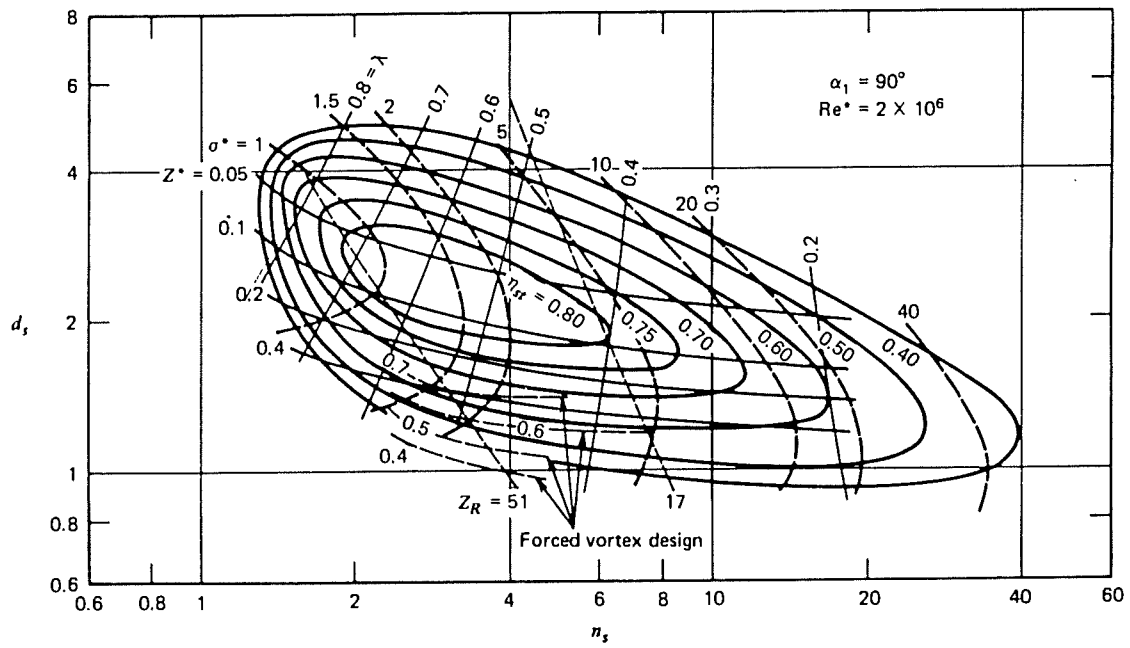
Calculated n_s d_s diagram for single-stage axial machines.
