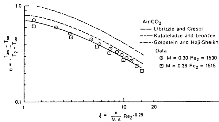
Film cooling effectiveness for air-carbon dioxide ( CO_2 ).
