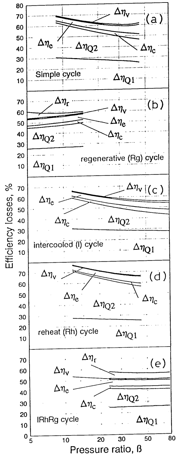
Fig. 10.7 Efficiency losses (as defined in Par. 10.3.1) of simple gas cycles with T_{IT}=1250^{\circ}\text{C} as a function of pressure ratio \beta . The difference between unity and the sum of all losses represents \eta_{II} . The upper value of \beta of non-regenerative cycles is set by the limit on maximum compressor outlet temperature (see Tab. 10.1); for regenerative cycles, the limit is set by the need to maintain a minimum \Delta T across the regenerator.
