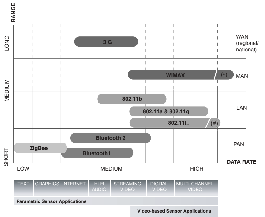
Figure 4.5 Graphical comparison of available protocols.
