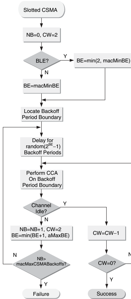
Figure 5.19 Slotted CSMA algorithm.
