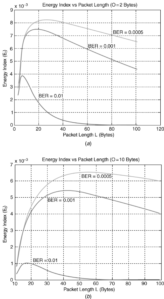
Figure 11.7 Energy index versus packet length: (a) packet overhead ( O ) is 2 bytes; (b) O is 10 bytes.
