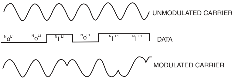
Figure 4A.1 PSK.
