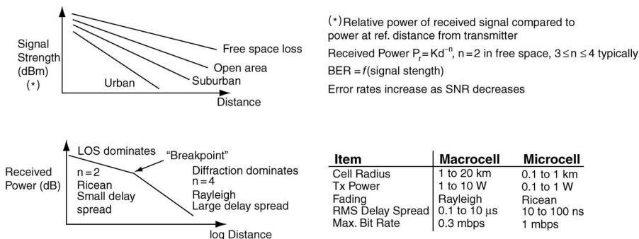
Figure 4.2 Outdoor radio propagation. (Based in part on [4.2].)
