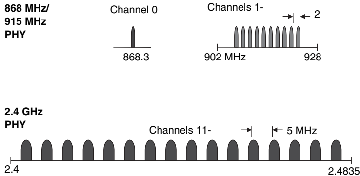
Figure 5.13 IEEE 802.15.4 PHY-layer operating frequency bands.
