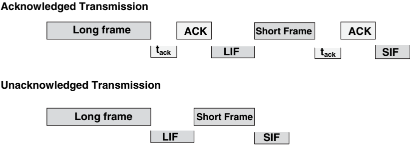
Figure 5.18 Interframe spacing.
