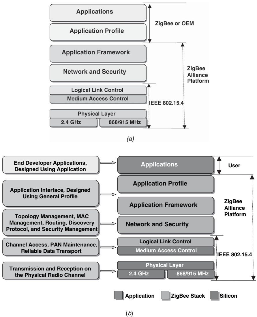
Figure 5.12 (a) IEEE 802.15.4 and ZigBee reference model; (b) ZigBee stack reference model.
