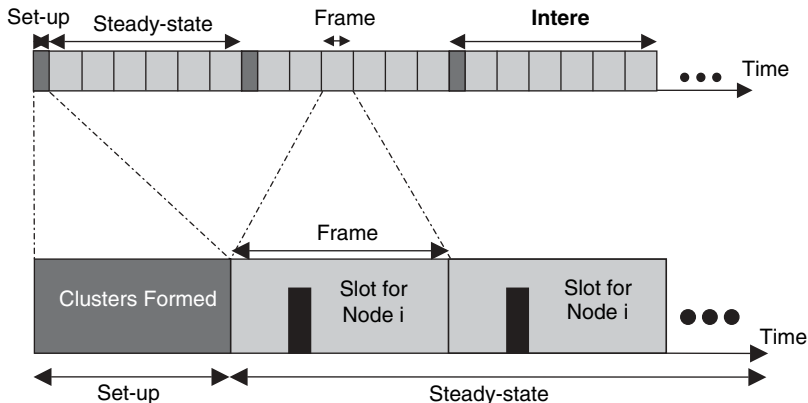
Figure 6.10 LEACH phases [6.18].
