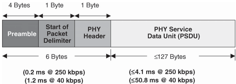
Figure 5.14 IEEE 802.15.4 PHY-layer packet structure.
