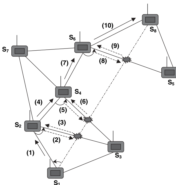
Figure 6.18 Perimeter traversal on a planar graph.
