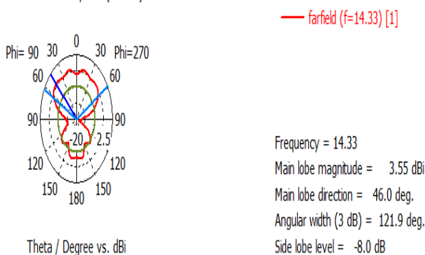
Figure. 8: Polar plot of far field pattern of proposed antenna at frequency 14.33GHz
