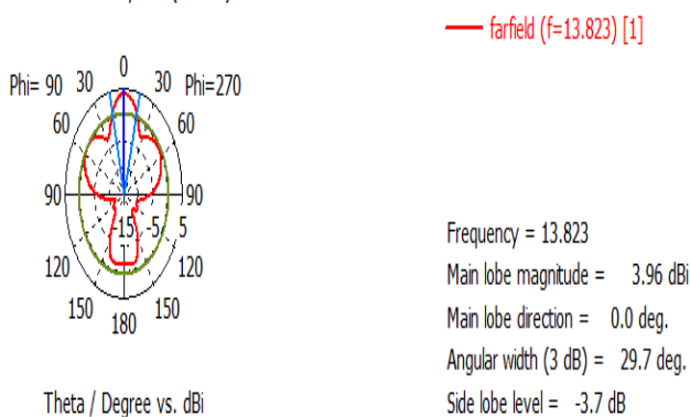
Figure. 9: Polar plot of far field pattern of proposed antenna at frequency 13.823GHz
