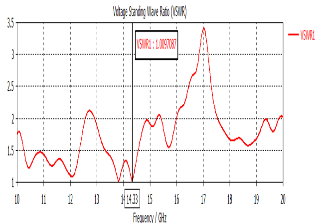
Figure. 4: VSWR of proposed fork antenna frequency 14.33GHz
