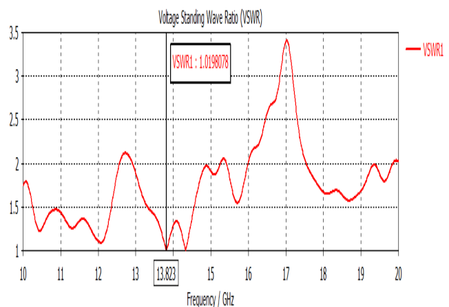
Figure. 5: VSWR of proposed fork antenna frequency 13.823GHz
