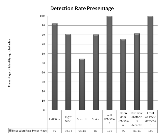
Fig. 11. Obstacle identification analysis.
