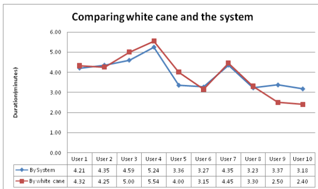
Fig. 13. Comparative analysis.
