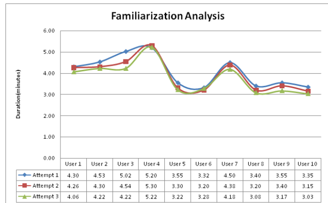
Fig. 10. Familiarization analysis.
