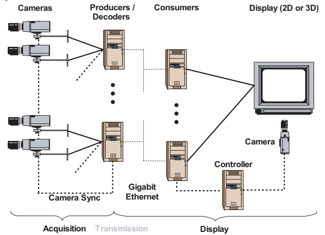
Figure 3: Modified implementation for compression, transmission, and decoding in our prototype system.
