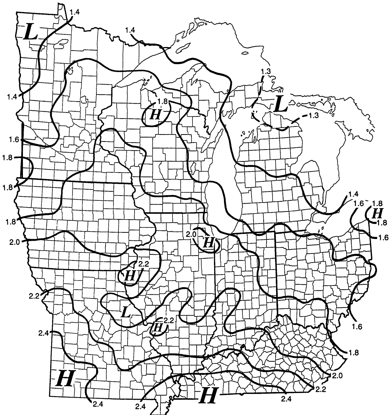
Figure 3. Spatial distribution of 3-hour rainfall (inches)
