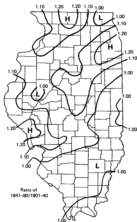
Figure 15. Ratio for two 40-year periods (1941-1980 and 1901-1940) for 2-year, 24-hour storms
