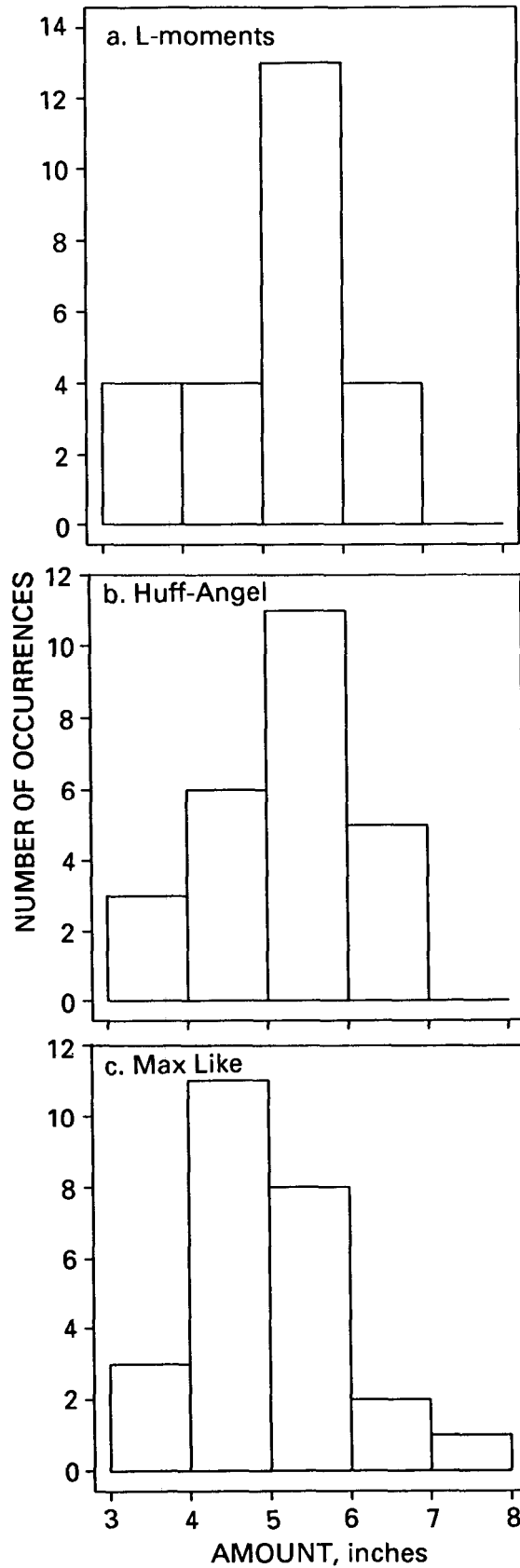
Figure 10. Histogram comparisons for 1-day rainfall in Minnesota
