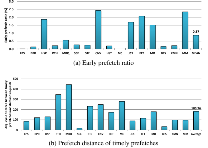
Figure 14: Early prefetch ratio and average prefetch distance of timely prefetches
