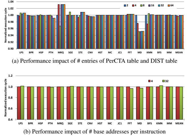
Figure 15: Performance variation w.r.t. # entries of PerCTA table and DIST table and # base addresses per load instruction
