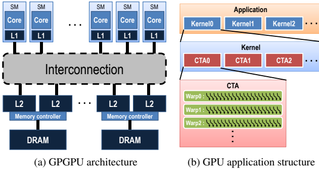
Figure 1: GPGPU hardware and software architecture
