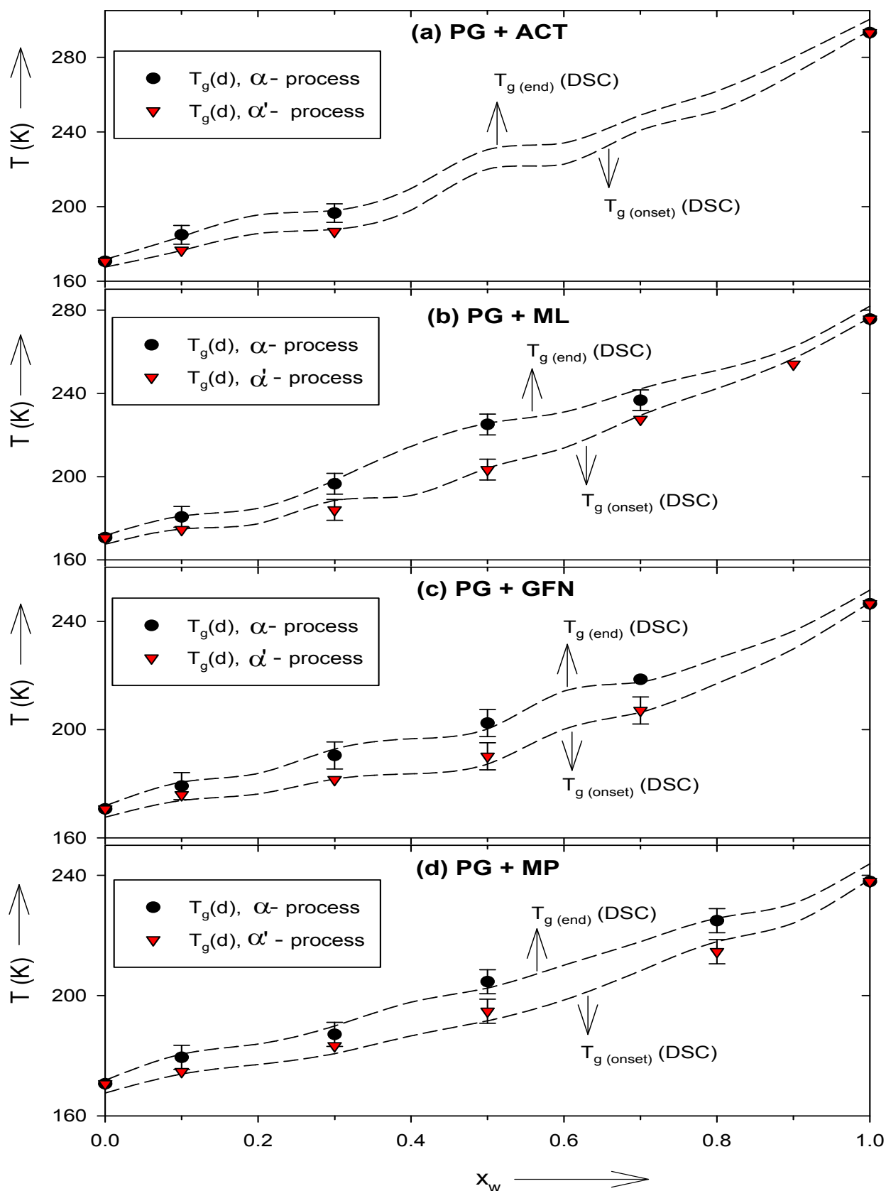
Figure 11: The variation of T_g (d) of \alpha - and \alpha' -processes, with weight fraction ( x_w ) of drug samples, is shown, where, T_g (d) is the temperature at which f_m = 10^{-3} Hz. The dotted lines correspond to T_g (onset) (DSC) and T_g (end) (DSC) for supercooled binary liquid mixtures.
