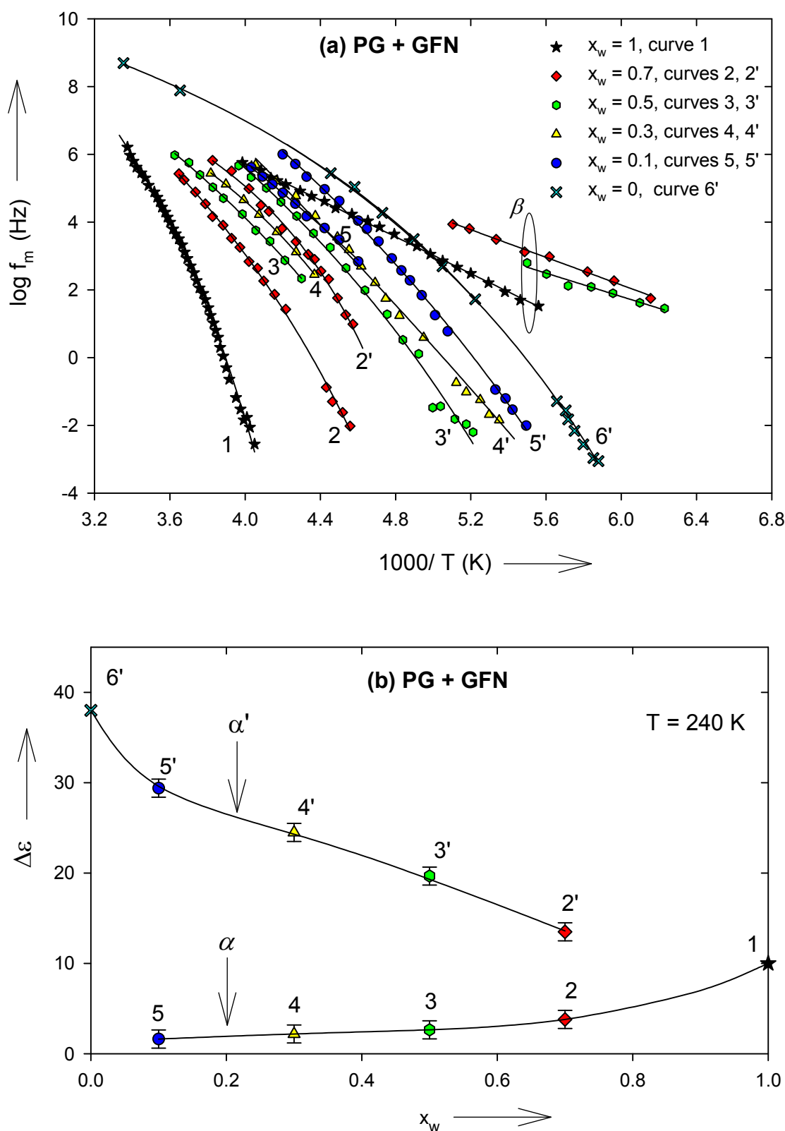
Figure 9: PG + GFN binary mixture (a) Arrhenius diagram depicting the \alpha - (curves 1 - 5), \alpha' - (curves 2' - 6') and \beta - processes, where x_w = 0 corresponds to neat PG [33] and x_w = 1 corresponds to neat GFN [16]. The thick line along the \alpha - and \alpha' - processes corresponds to Eq. (3) (for f_m < 10^4 Hz), and that along the \beta - process corresponds to Eq. (4), for the parameters given in Table 3. (b) Variation of dielectric strength ( \Delta\epsilon ) of \alpha - and \alpha' - processes with x_w , at the temperature shown in the figure.
