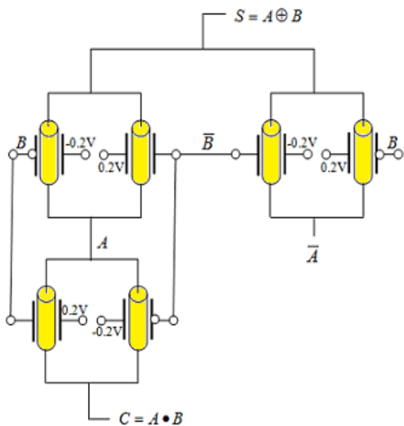
Fig. 11. Half-adder using CNTFET-TG.
