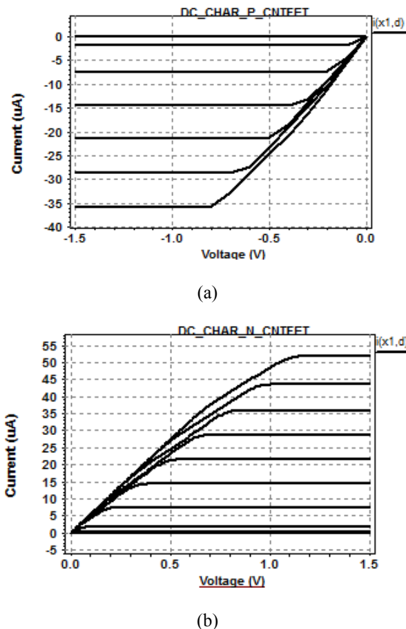
Fig. 4. (a) I_D - V_{DS} characteristics of p-type CNTFET. (b) I_D - V_{DS} characteristics of n-type CNTFET. Parameters: d = 1.5 \text{ nm} , R_{SD} = 75 \text{ k}\Omega , T = 300\text{K} .
