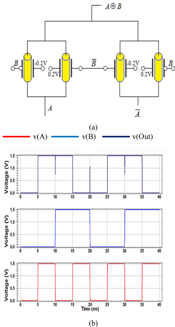
Fig. 10. (a) TG XOR using CNTFET, (b) transient characteristics of CNTFET TG XOR.
