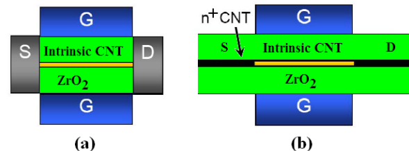
Fig. 1. Different types of CNTFETs: (a) Schottky barrier (SB) CNTFET (b) MOSFET-like CNTFET.
