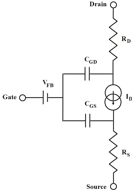
Fig. 2. Schematic of SPICE compatible CNTFET model, where C_{GS} is gate to source capacitance, C_{GD} is gate to drain capacitance, R_D is drain resistance, R_S is source resistance, V_{FB} is flat-band voltage, and I_D is drain current.
