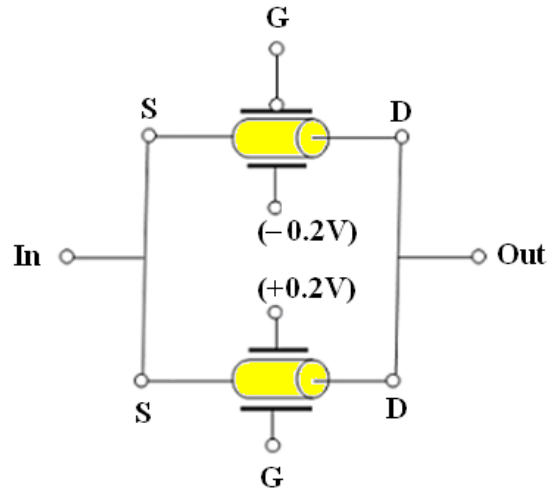
Fig. 9. Transmission-gate using CNTFET.
