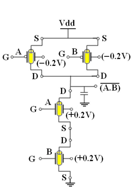
Fig. 6. Two input NAND gate using CNTFET.
