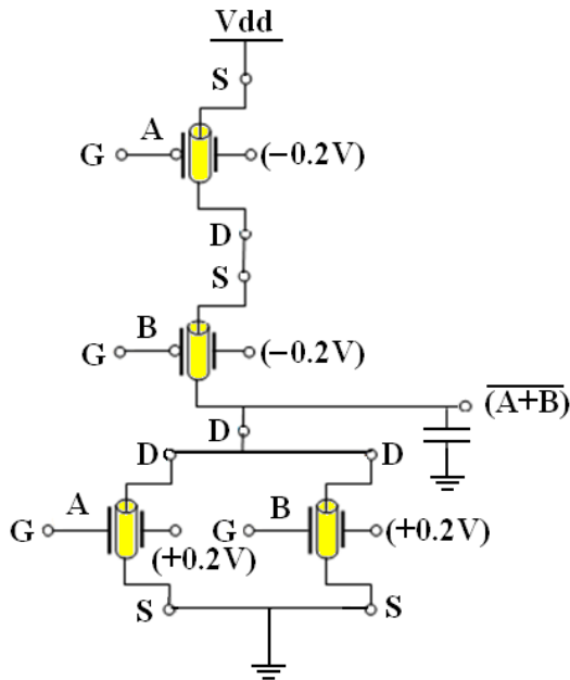
Fig. 7. Two input NOR gate using CNTFET.
