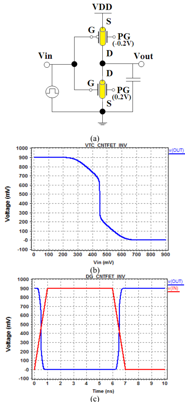
Fig. 5. CNTFET inverter (a) schematic, (b) voltage transfer characteristic, (c) and transient characteristics.
