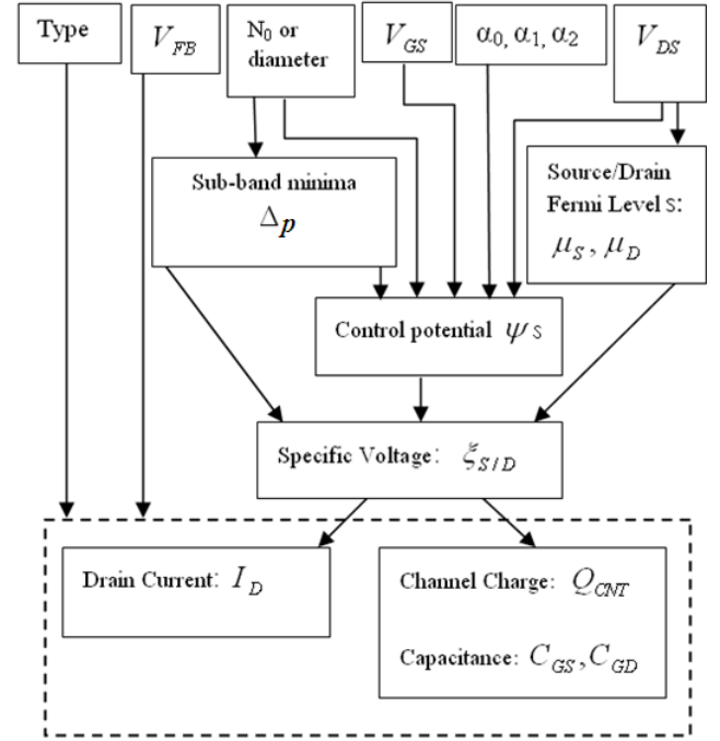
Fig. 3. Structure of CNTFET compact model.
