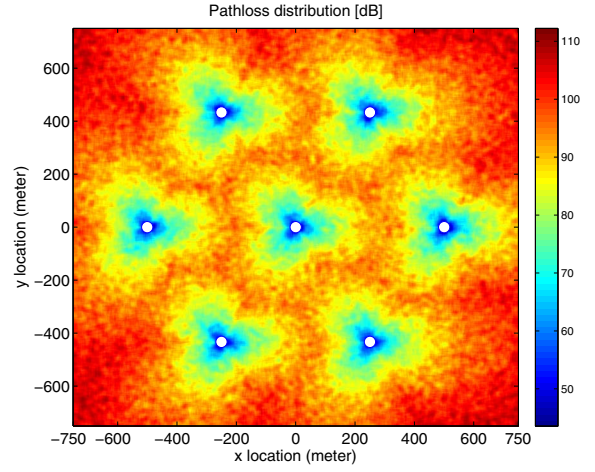
Fig. 6. Simulation region (of size 1500 \times 1500 \text{ m}^2 ) showing pathloss (dB) that includes antenna gain, distant dependent macroscale pathloss, and lognormal shadow fading pathloss.
