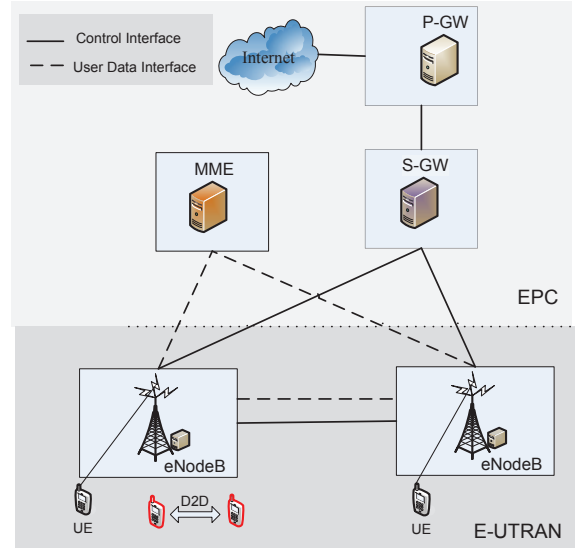
Fig. 1. System level overview of LTE architecture.
