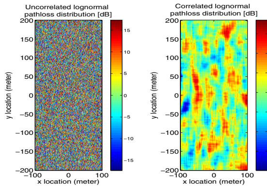
Fig. 5. Uncorrelated and space-correlated lognormal shadow fading pathloss map (in dB).
