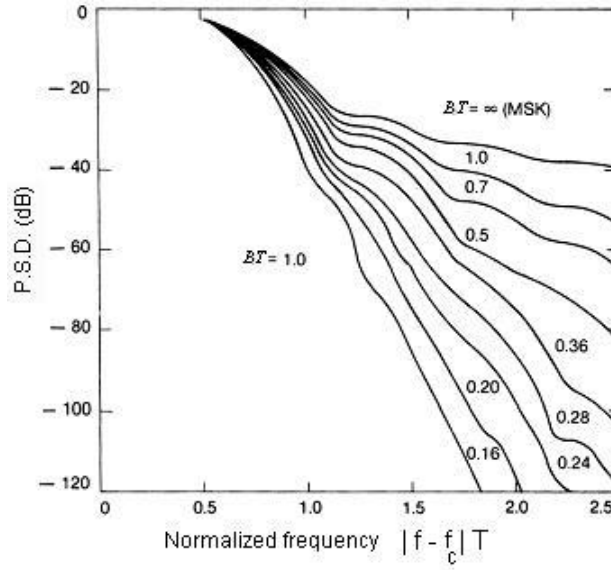
Figure 6.12: Spectrum of GMSK scheme.
