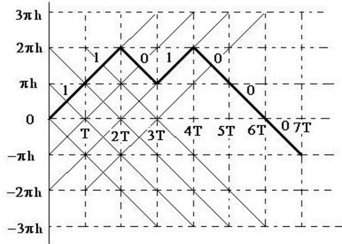
Figure 6.8: Phase tree of 1101000 CPFSK sequence.
