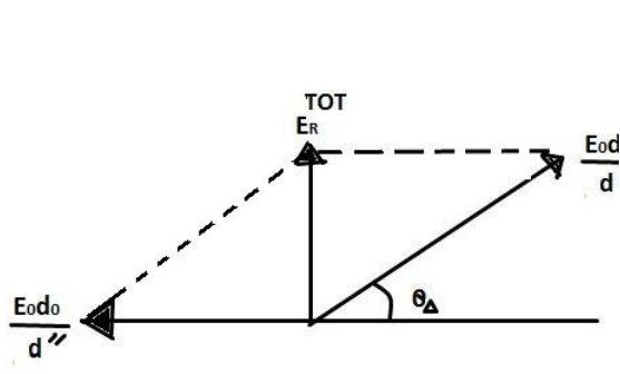
Figure 4.3: Phasor diagram of electric fields.
