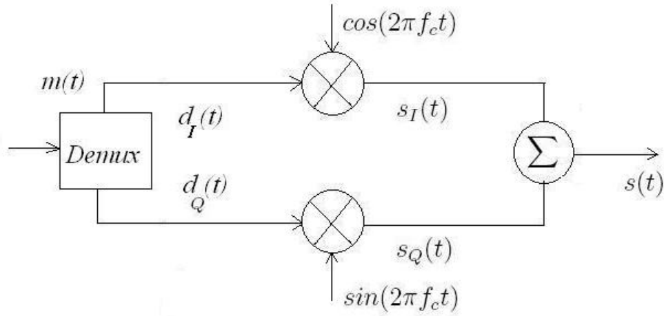
Figure 6.3: QPSK transmitter.
