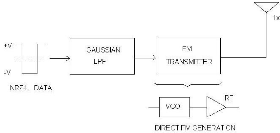
Figure 6.10: GMSK generation scheme.
