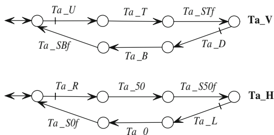
Fig. 8 Plant model of elevating rotary table
