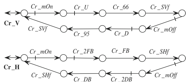
Fig. 4 Plant model of crane
