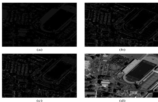
Fig 6. Difference between (d) the original high-resolution satellite image and (a) the proposed enhanced image, (b) the standard bicubic interpolation, and (c) the WZP- and CS-based image resolution enhancement technique.
