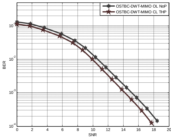
Fig.8.BER performance of WiMAX Closed loop with THP OSTBC-MIMO DWT OFDM in AWGN & Multipath stationary Pedestrian B channel.
