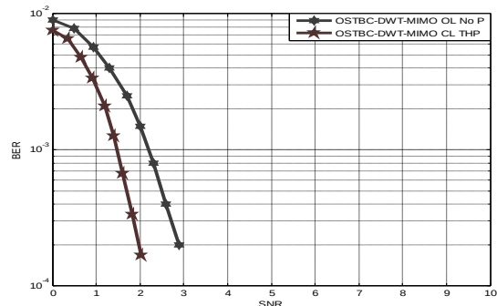
Fig .3. BER performance of WIMAX with THP OSTBC-MIMO DWT OFDM in AWGN channel model.
