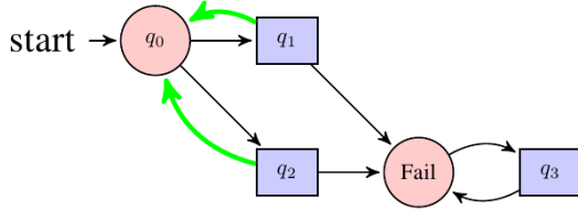
Fig. 2. An example of a game graph and a winning strategy for player 2 (red edges)
