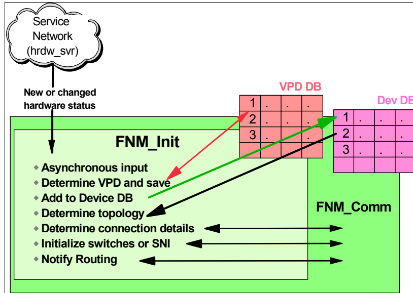
Figure 2-37 FNM_Init logical description
