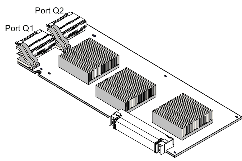
Figure 2-13 p655 two-port GX card
