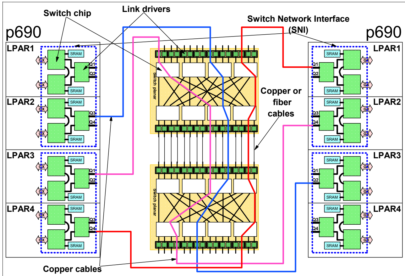
Figure 1-9 Switch hardware diagram
