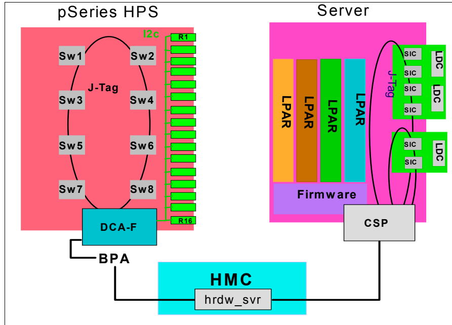
Figure 2-34 JTAG access to HPS components
