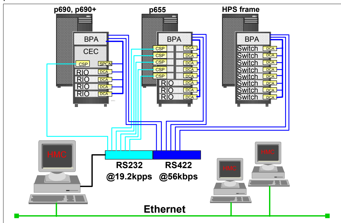
Figure 2-22 General HPS cabling example
