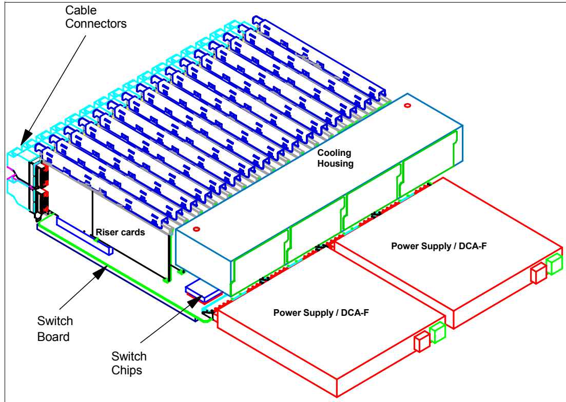
Figure 2-6 pSeries High Performance Switch diagram
