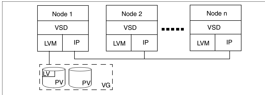
Figure 3-15 Logical view of the VSD subsystem
