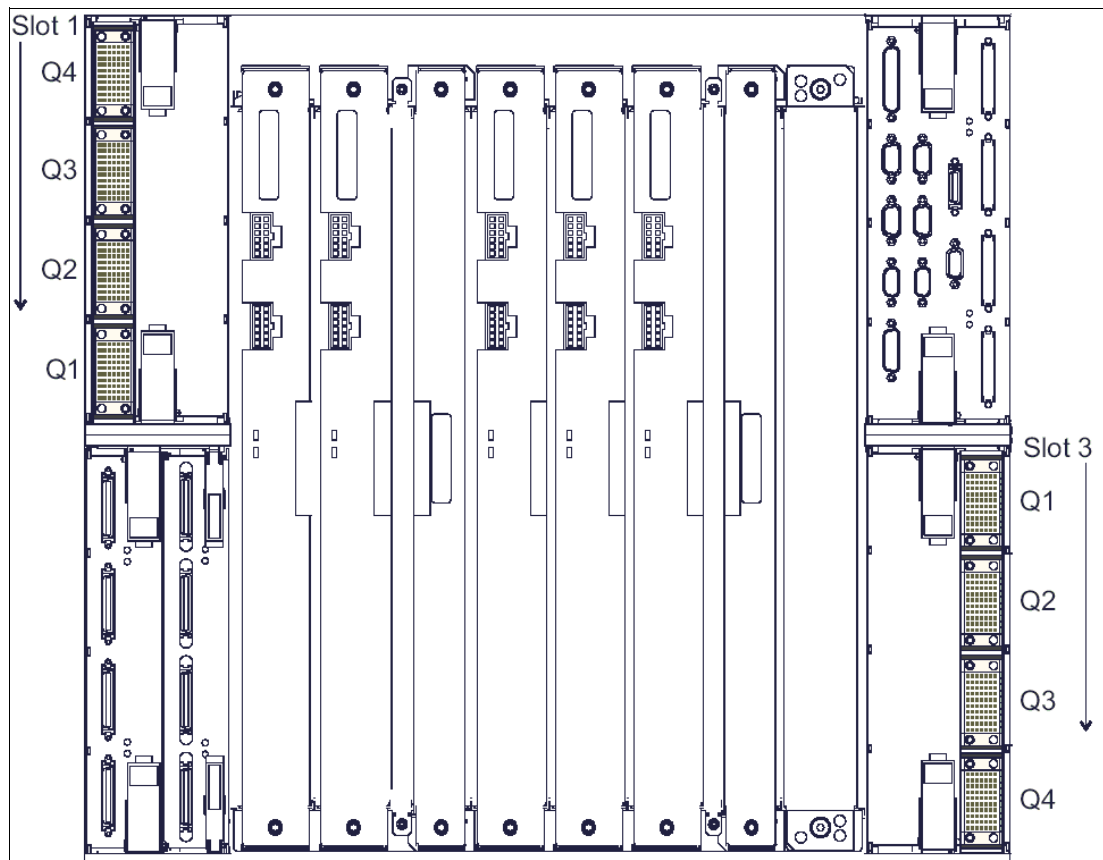
Figure 2-20 7040 CEC rear diagram
