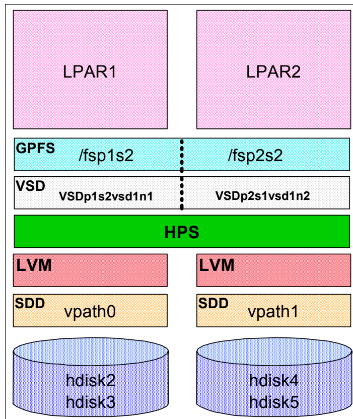
Figure 5-5 The GPFS scenario diagram
