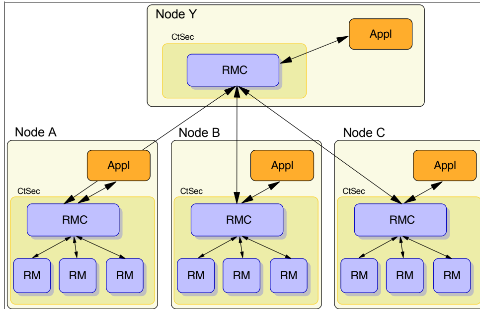
Figure 3-13 Management domain RMC
