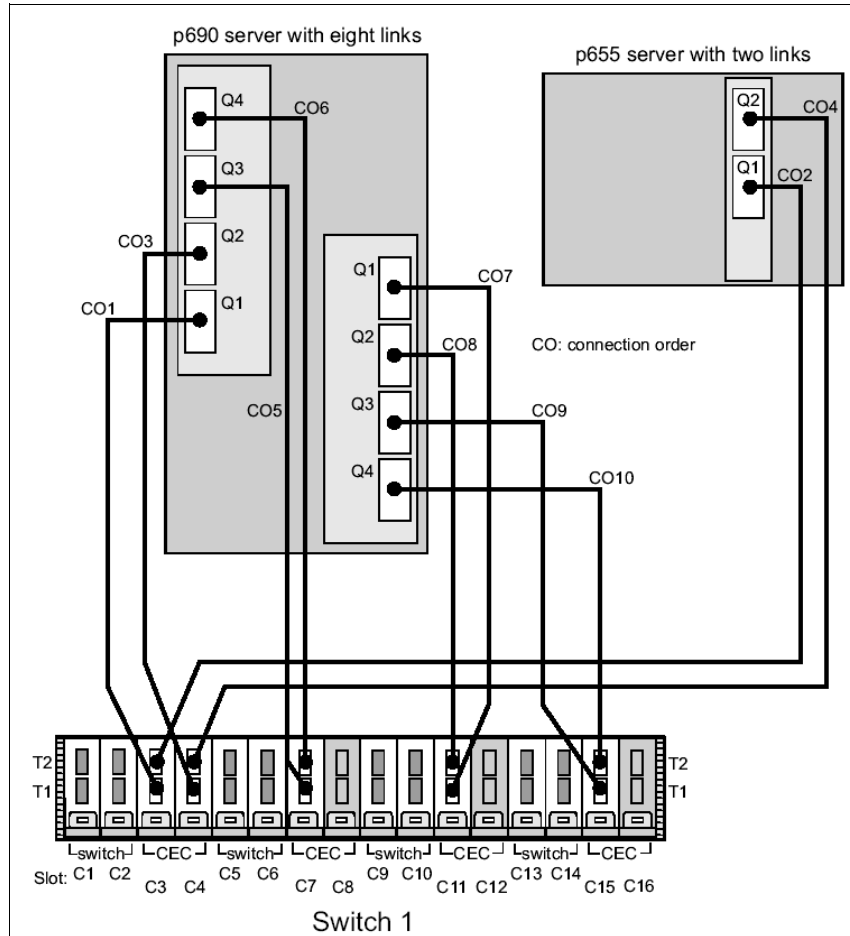
Figure 2-25 Sequentially cabled switch network
