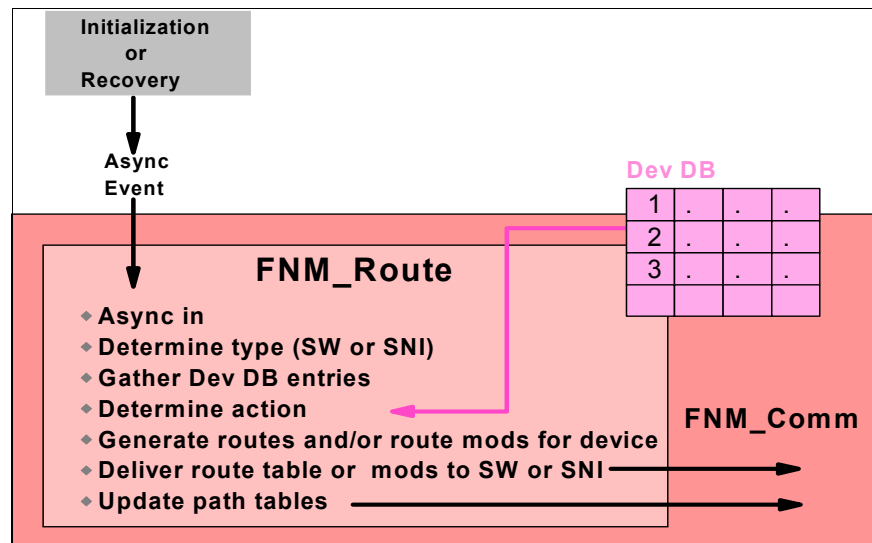
Figure 2-38 HPS routing overview
