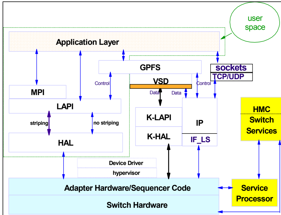
Figure 3-25 Message Passing Software Architecture
