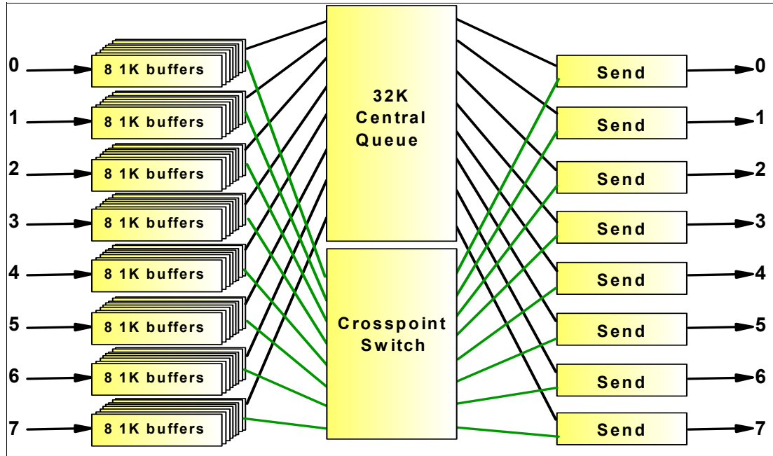
Figure 2-7 Internal diagram of the switch chip
