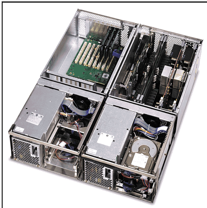
Figure 1-6 375 MHz wide node (Winterhawk II)
