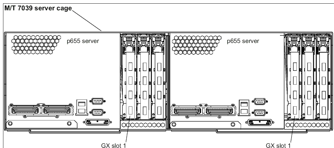
Figure 2-15 p655 physical rear diagram
