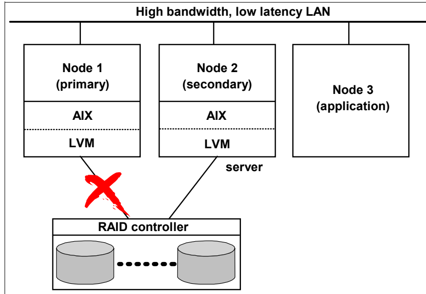
Figure 3-22 Backup node serving RAID device
