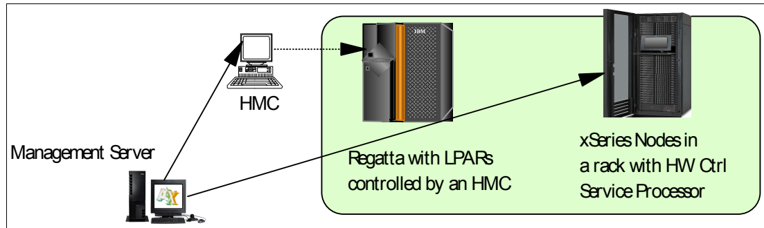
Figure 1-8 CSM Cluster 1600 example
