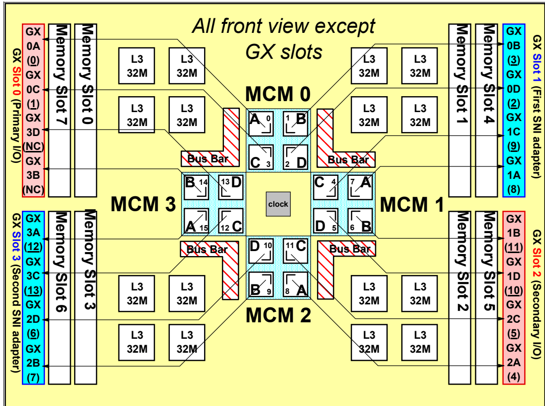
Figure 2-17 MCM to GX bus activation chart
