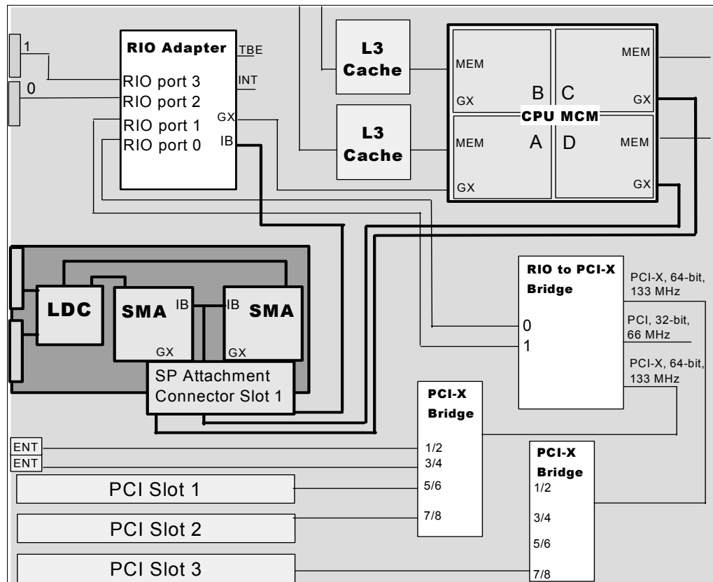
Figure 2-14 p655 logical bus architecture
