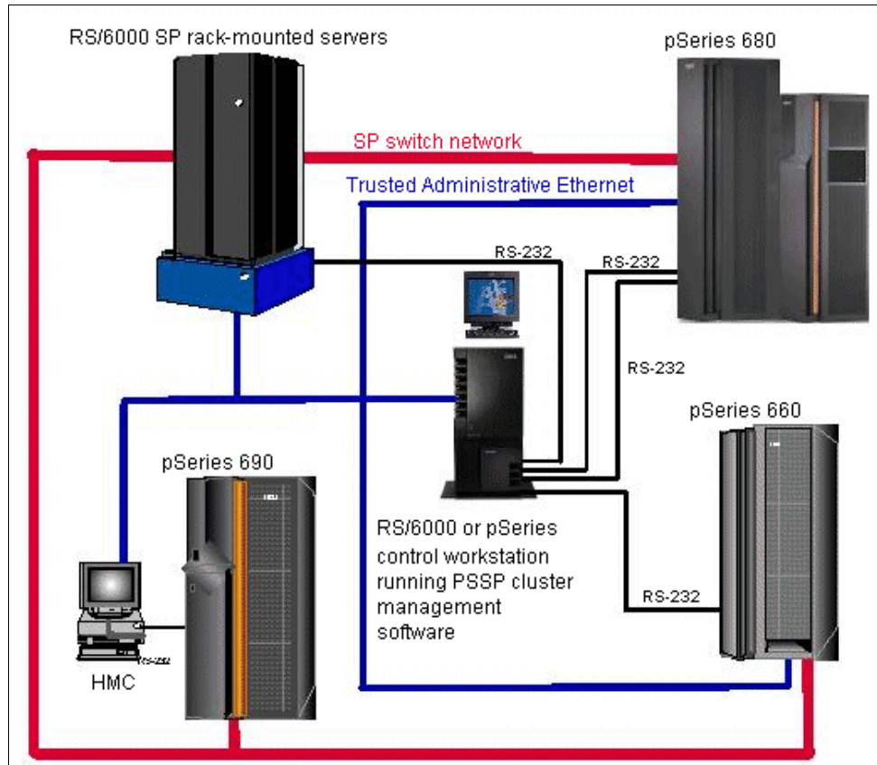
Figure 1-7 Cluster 1600 with PSSP and p690
