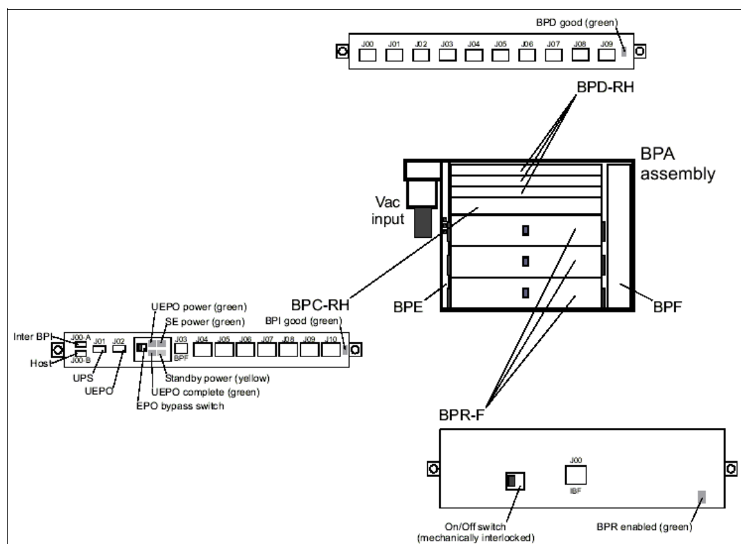
Figure 2-5 Components of a Bulk Power Assembly (BPA)
