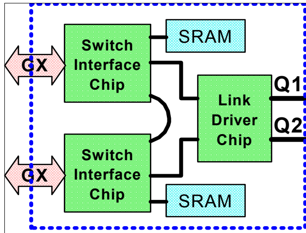
Figure 2-12 SNI logical view
