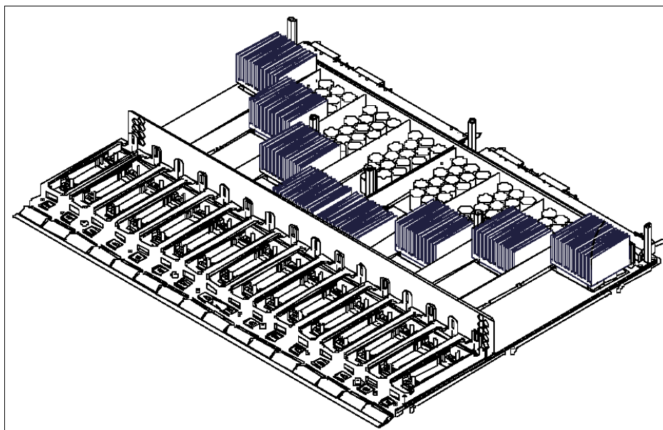
Figure 2-9 Physical diagram of an HPS switch board
