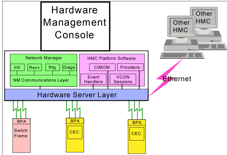
Figure 2-29 Hardware Server network
