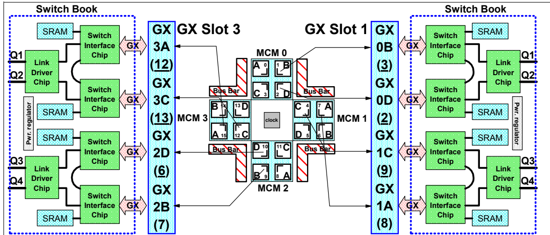
Figure 2-18 SNI-to-MCM relationship (front view)
