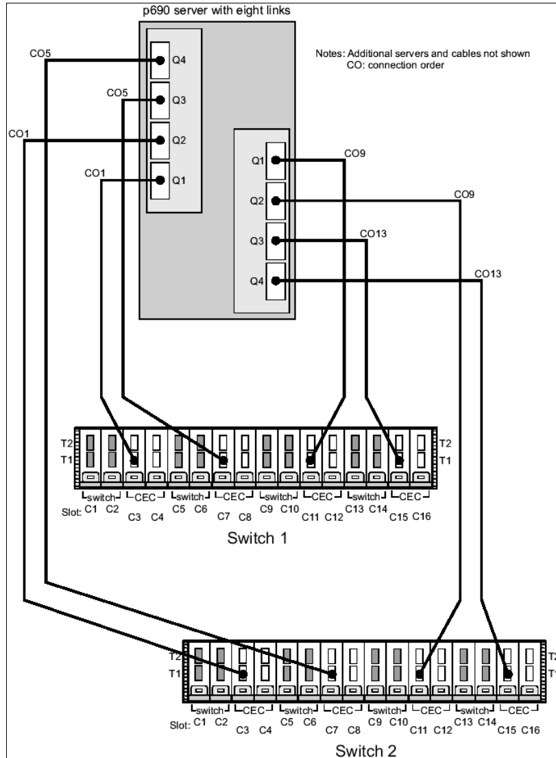
Figure 2-24 Dual-plane configuration
