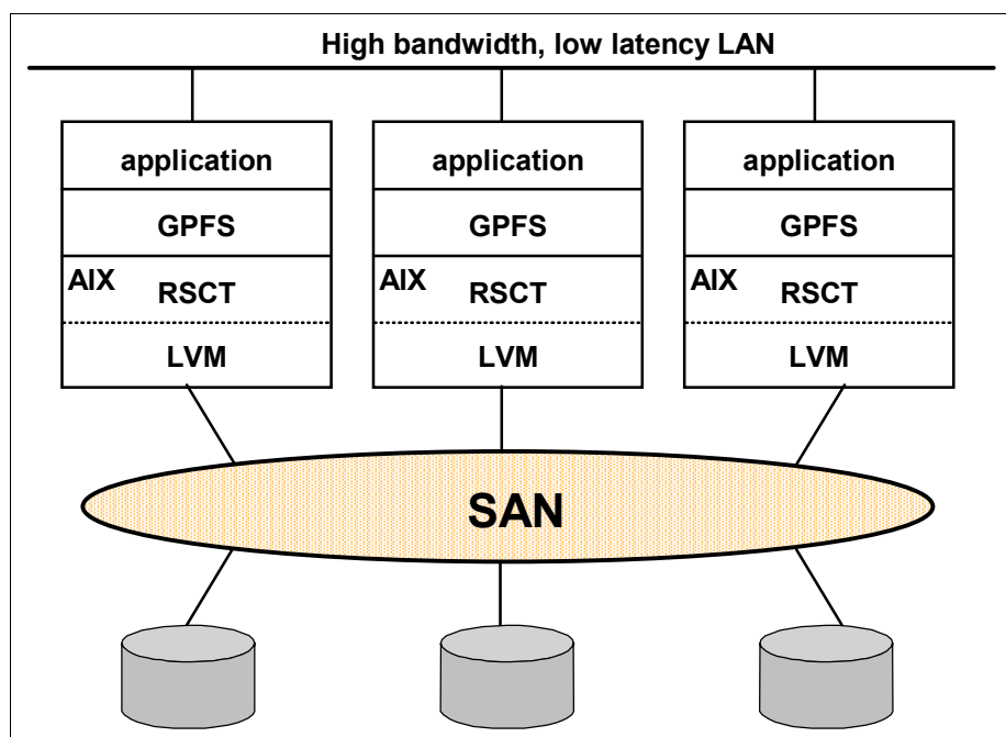
Figure 3-19 A GPFS cluster with SAN-attached disks
