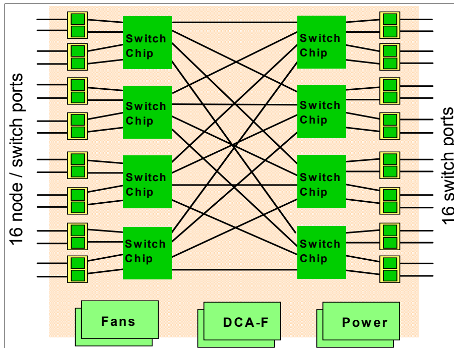
Figure 2-8 Logical view of HPS switch board
