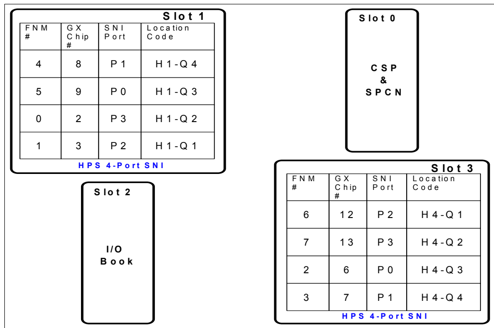
Figure 2-21 SNI to GX bus map
