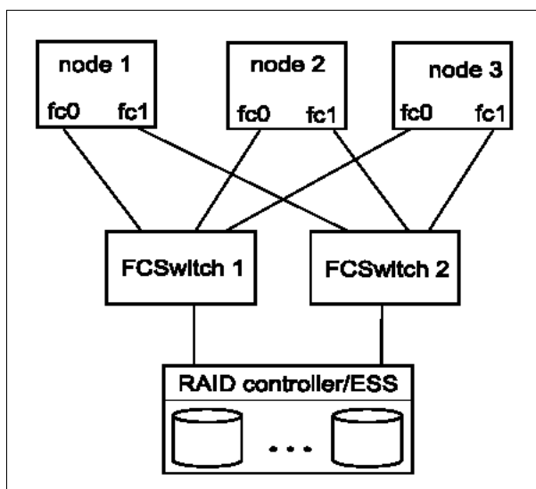
Figure 3-24 RAID/ESS Controller multi-tailed to each node
