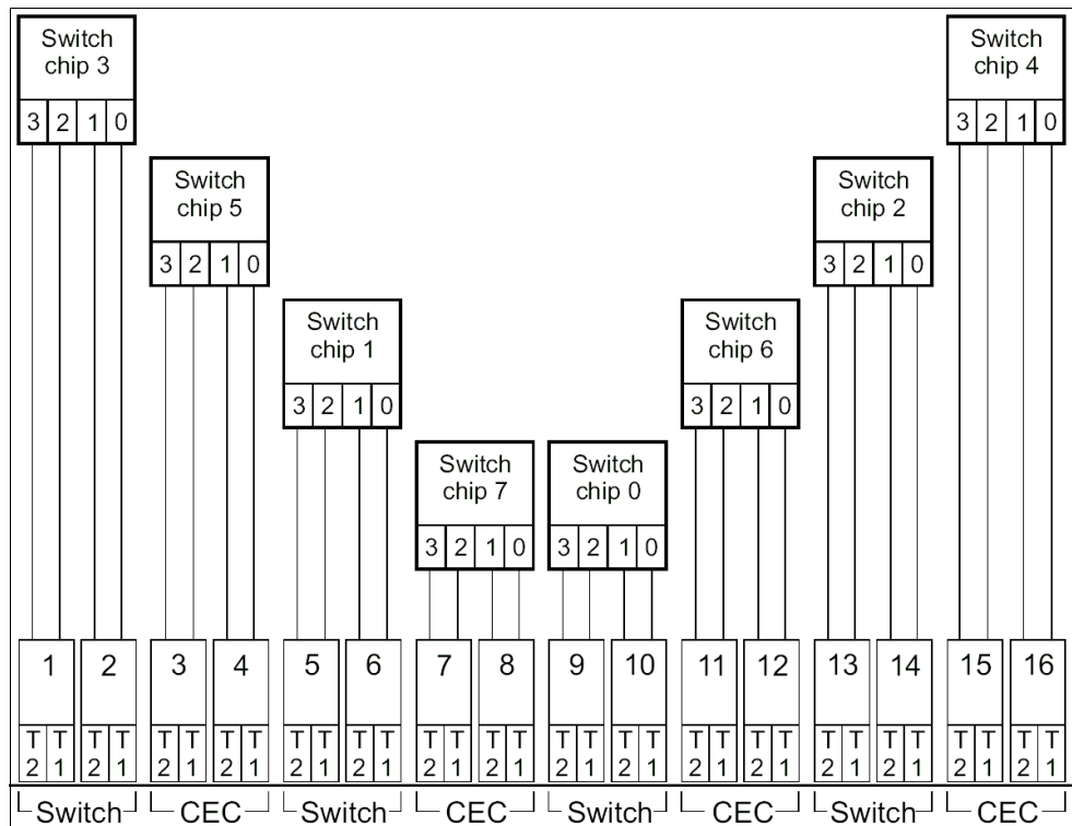
Figure 2-11 Switch port connector card numbering from front view
