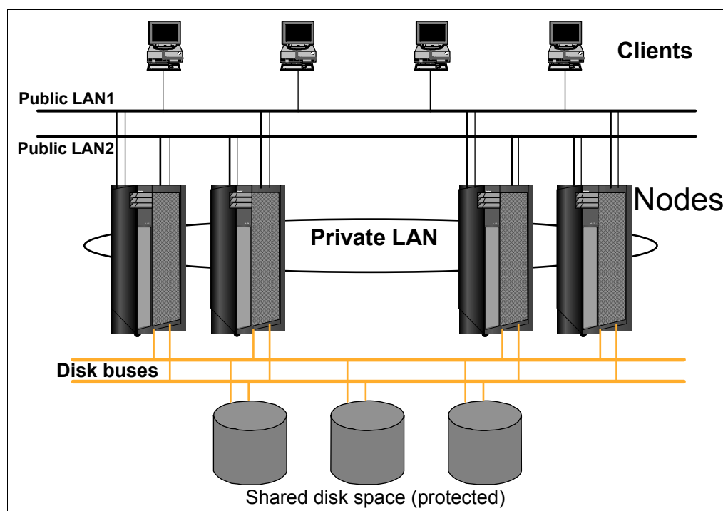
Figure 3-14 Example HACMP cluster scenario
