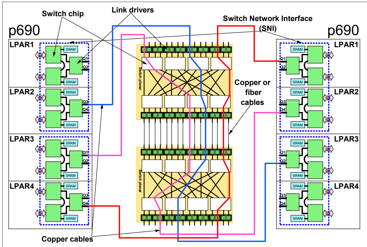
Figure 2-1 Switch hardware diagram
