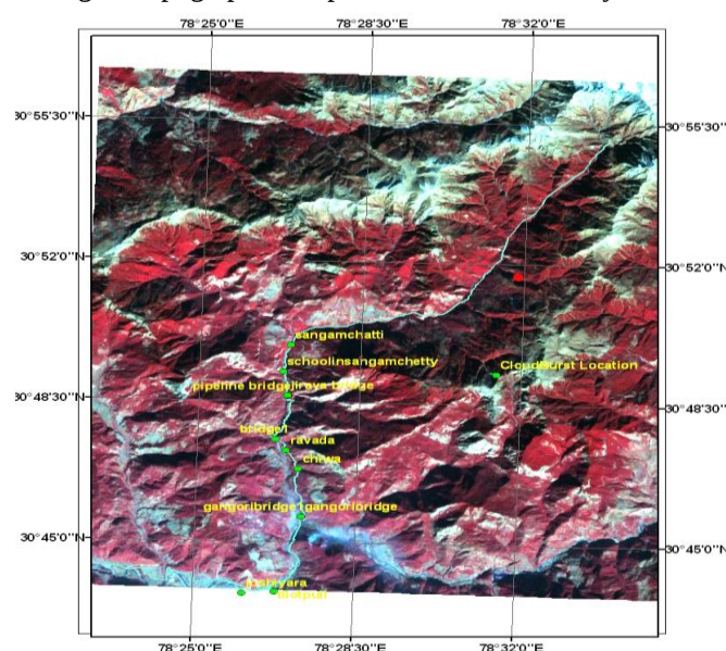
Fig.2. GPS data overlaid on Landsat ETM+ showing Cloudburst Location
