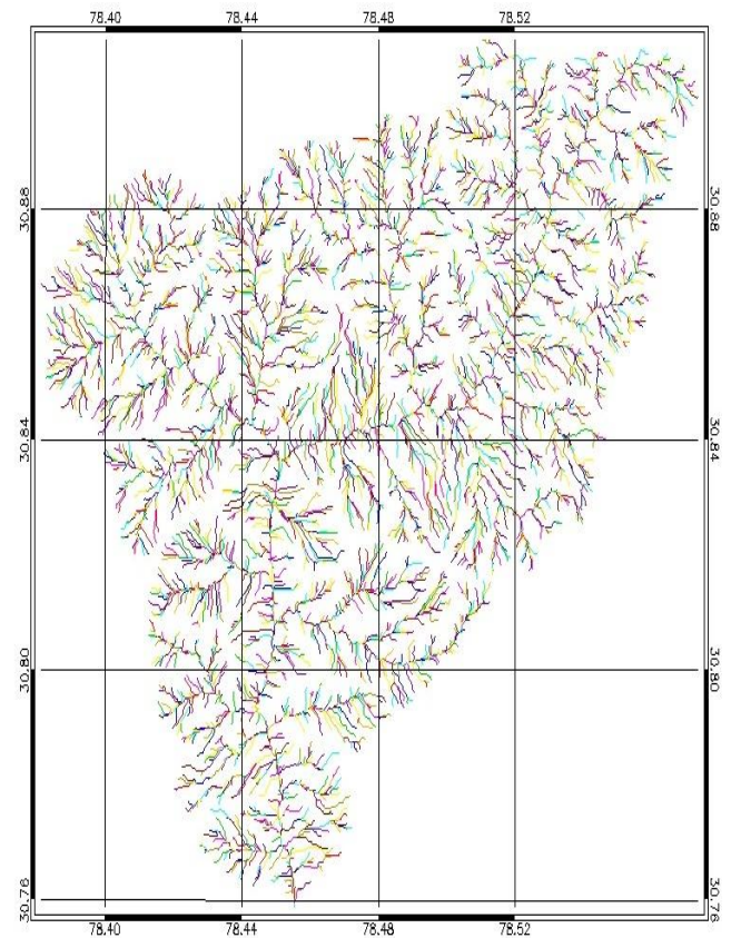
Fig.6 Evaluation of Stream order of study area in River tools
