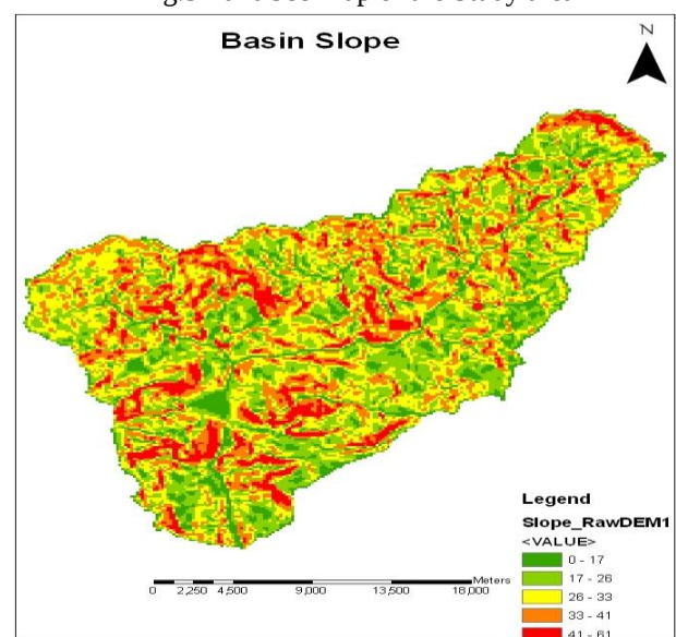
Fig.4 Slope angle map of the Study area
