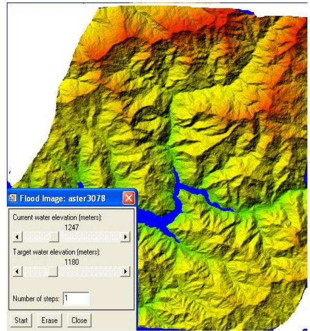
Fig.6 Visual representation of submerged area
