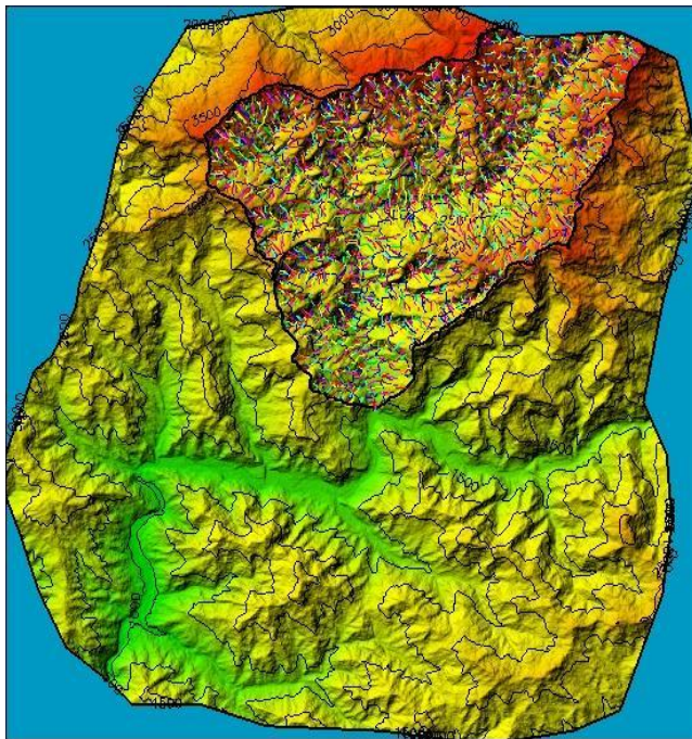
Fig.6 Elevation profile of the study area with contours
