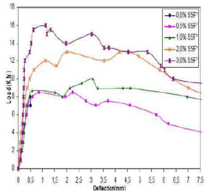
Fig.4. Load-deflection curves from deflection tests (various content of SSF*)
