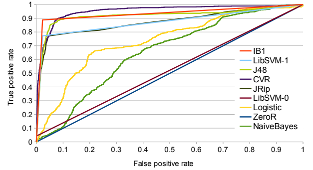
Figure 4: ROC curves for SeekingEngagement class
