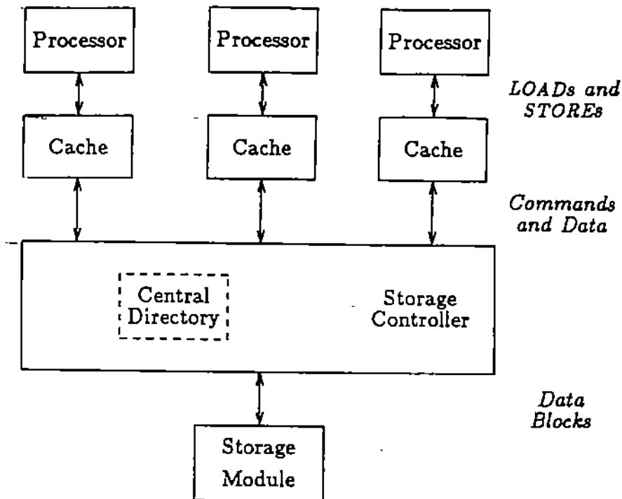
Figure 1.5 Tang's multiprocessor
