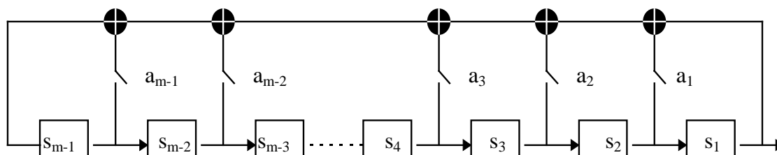
Figure 13. Linear Feedback Shift Registers ( a_i, s_i \in \{0,1\} ).
