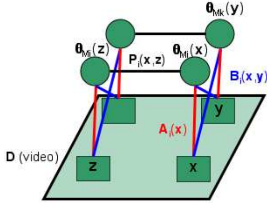
Figure 4: Contrast-dependent random field (CDRF) formulation of the energy of the layered representation containing two segments p_i and p_k . The appearance term \mathcal{A}_i(\mathbf{x}; \Theta, \mathbf{D}) , shown in red, connects the data \mathbf{D} (specifically the set of RGB values \mathcal{I}_i^j(\mathbf{x}) ) with the matte \Theta_{Mi}(\mathbf{x}) . The prior \mathcal{P}_i(\mathbf{x}, \mathbf{z}; \Theta) between two neighbouring points \mathbf{x} and \mathbf{z} , which encourages spatial continuity, connects \Theta_{Mi}(\mathbf{x}) and \Theta_{Mi}(\mathbf{z}) . The data dependent contrast term \mathcal{B}_i(\mathbf{x}, \mathbf{y}; \Theta, \mathbf{D}) , which cannot be included in the prior, is shown as the blue diagonal connections. Extending the formulation to more than two segments is trivial. Note that some of these diagonal connections are not shown, i.e. those connecting the other neighbouring points of \mathbf{x} and \mathbf{y} to \Theta_{Mk}(\mathbf{y}) and \Theta_{Mi}(\mathbf{x}) respectively, for the sake of clarity of the figure.
