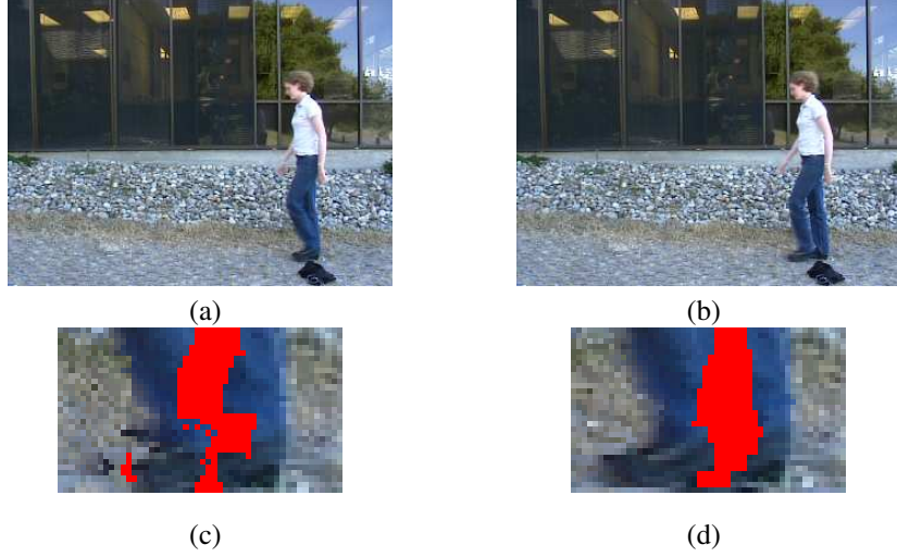
Figure 7: Effects of modelling motion blur. (a)-(b) Two consecutive frames from the video shown in Fig. 1. (c) The image motion computed without modelling motion blur. The reconstruction of the second frame, obtained by mapping the patches of the first frame according to the transformations obtained, indicates that incorrect transformations are found around the feet (see e.g. the shoes) where there is considerable motion blur. Note that the pixels marked red are those that are occluded in the first frame but present in the second frame. (d) Results after modelling motion blur. Accurate transformations for the patches belonging to the shoes are obtained by accounting for the change in appearance due to motion blur.
