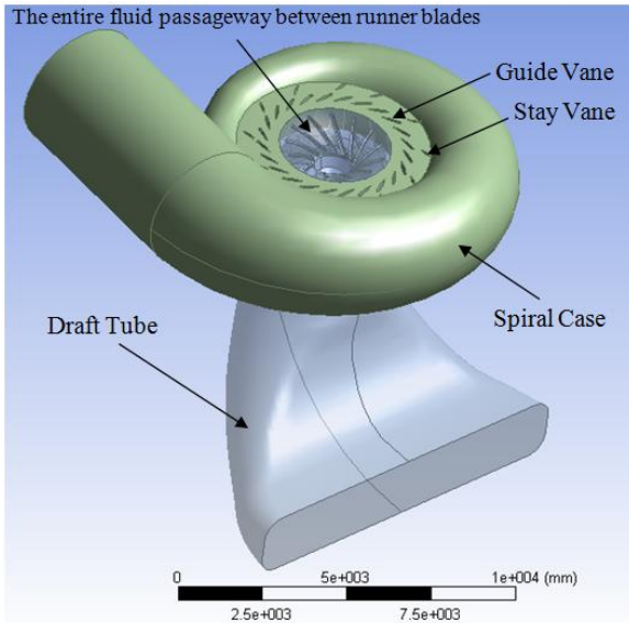
Fig 1: The geometrical model used in the simulation
