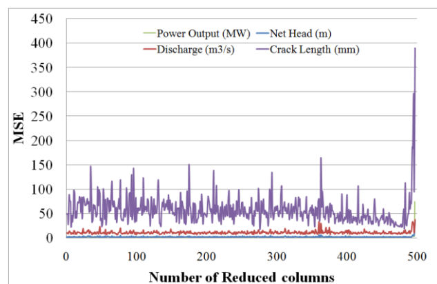
Fig 18: MSE for the estimated crack length and turbine operation conditions using amplitude of FRFs data sets along z-direction (500 spectral lines)
