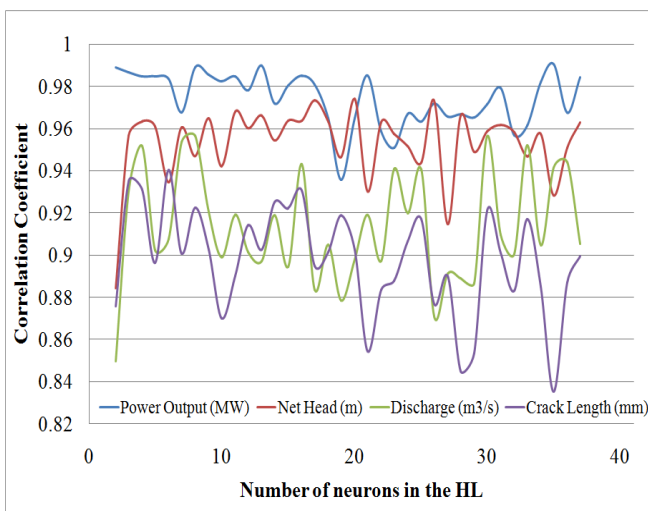
Fig 11: Correlation Coefficient for estimation of the turbine operation conditions and crack length by using amplitude of FRFs along x-direction (7 spectral lines)
