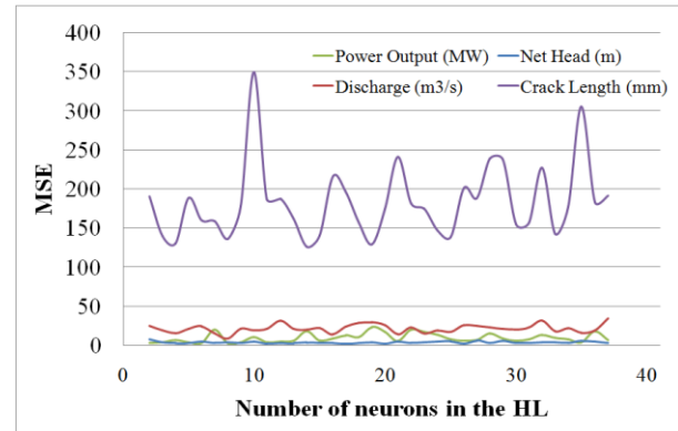
Fig 12: MSE for estimation of the turbine operation conditions and crack length by using amplitude of FRFs along x-direction (7 spectral lines)
