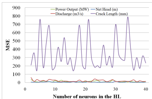
Fig 15 : MSE for the estimated crack length and turbine operation conditions using amplitude of FRFs data sets along z-direction (500 spectral lines)
