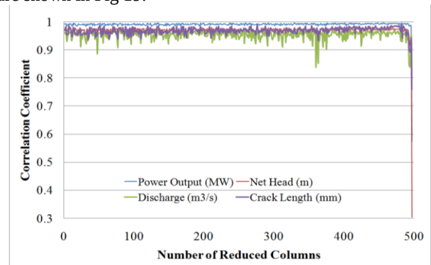
Fig 17: Correlation coefficients for the estimated crack length and turbine operation conditions using amplitude of FRFs data sets along z-direction (500 spectral lines)
