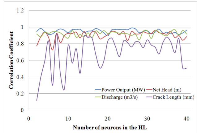
Fig 4: Correlation coefficient for estimation of the turbine operation conditions and crack length by using amplitude of FRFs along x -direction (500 spectral lines)
