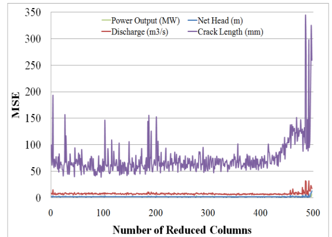
Fig 9: MSE for estimation crack length and turbine operation conditions using amplitude of FRFs data sets along x -direction (500 spectral lines)
