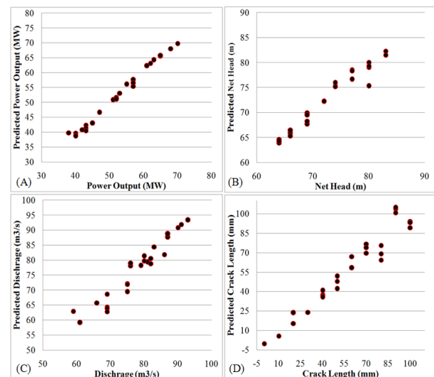
Fig 23: Identification of the power output (A) net head (B) discharge (C) and crack length(D) by using reduced amplitude of FRFs data sets along x and z -directions
