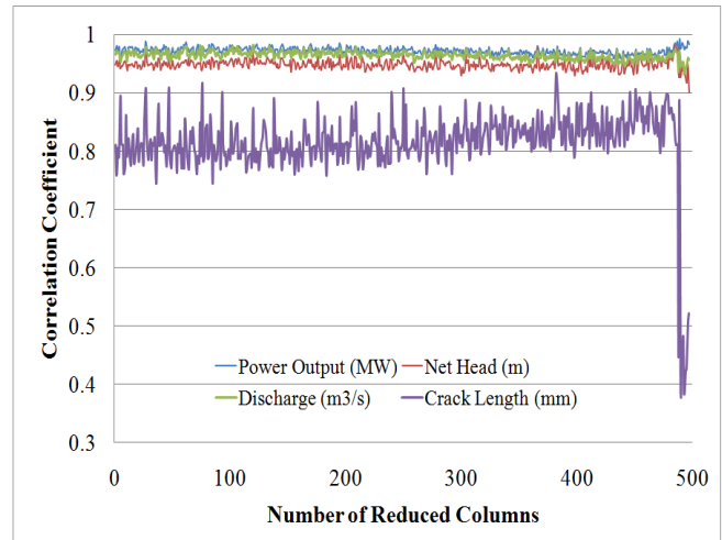
Fig 8: The correlation coefficients for estimated and actual crack length and turbine operation conditions using amplitude of FRFs data sets along x -direction (500 spectral lines)
