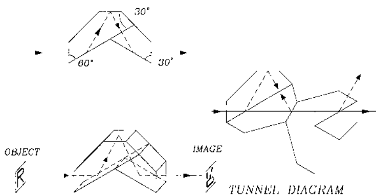
Figure 10.13 Reverting-inversing prism.
