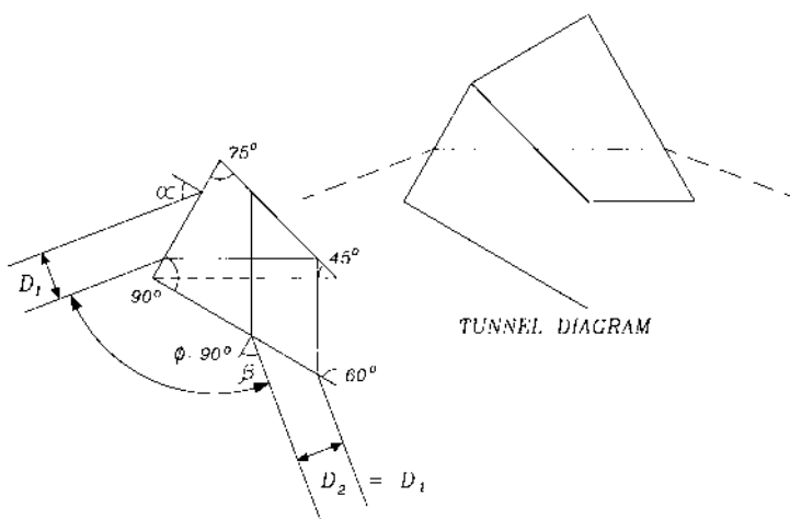
Figure 10.24 Constant deviation prism.
