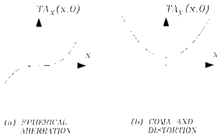
Figure 7.11 Sagittal plots for some aberrations: (a) spherical aberration; (b) coma and distortion.
