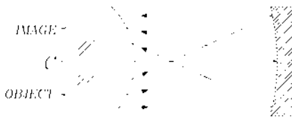
Figure 11.22 Dyson system.
