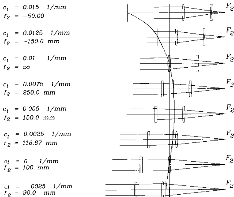
Figure 3.12 Position of the principal planes for a system of two separated thin lenses.
