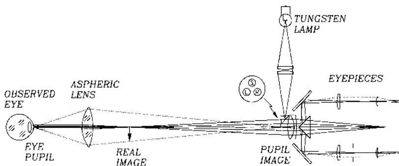
Figure 15.33 Indirect ophthalmoscope.
