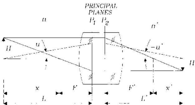
Figure 3.2 Image formation with a thick optical system.
