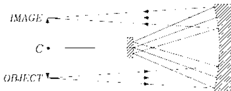
Figure 11.23 Offner system.
