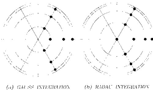
Figure 9.5 Distribution of rays in the pupil for Radau integration: (a) Gauss integration; (b) Radau integration.
