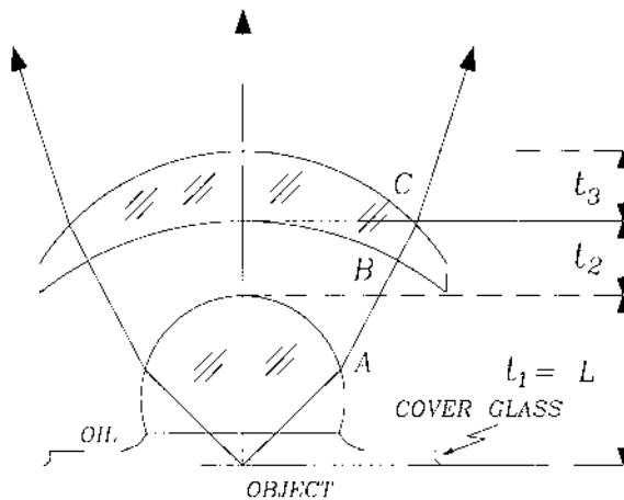
Figure 16.9 Duplex front of an oil immersion microscope objective.
