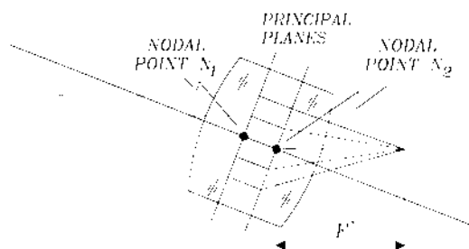
Figure 3.4 Measurement of the effective focal lens of a thick optical system.
