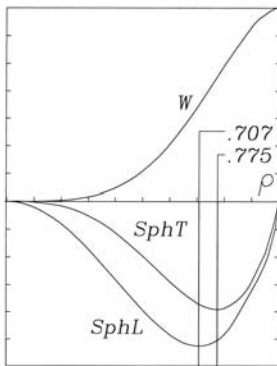
Figure 4.18 Transverse and longitudinal spherical aberration maxima when these aberrations are zero at the edge. The wavefront shape is also shown.
