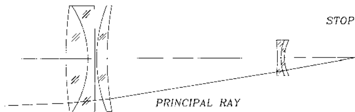
Figure 15.22 Galilean telescope.
