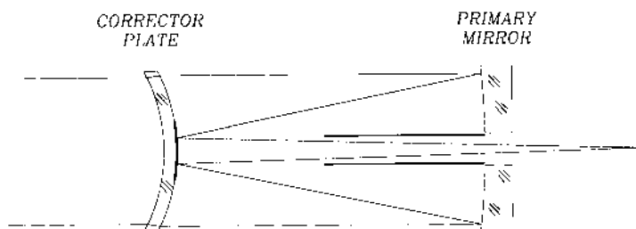
Figure 14.21 Maksutov–Cassegrain telescope.
