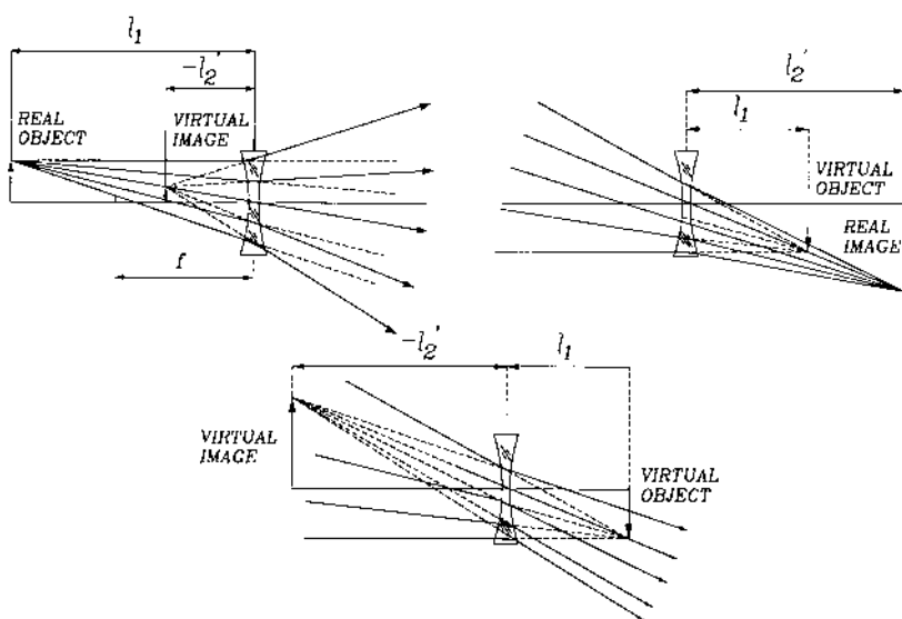
Figure 2.8 Image formation with thin divergent lenses.
