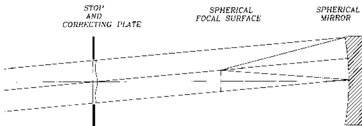
Figure 14.2 Schmidt camera.
