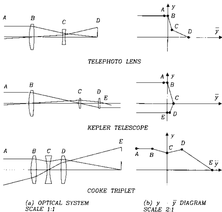
Figure 3.16 Three y - \bar{y} diagrams. (a) Optical system (scale 1:1); (b) y - \bar{y} diagram (scale 2:1).
