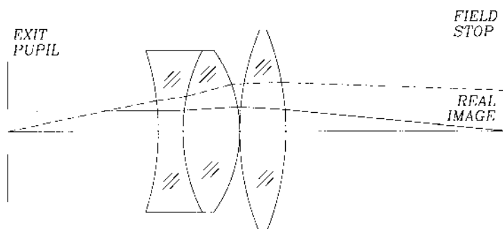
Figure 16.15 A 10 \times microscope wide-field eyepiece.
