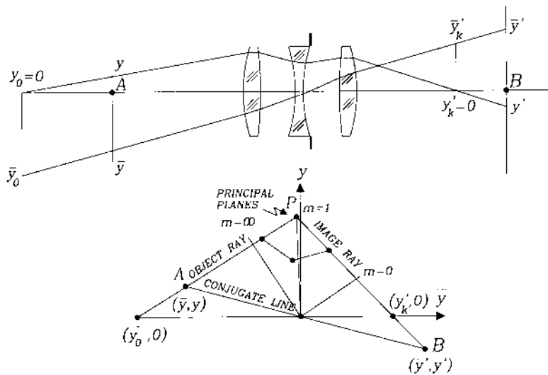
Figure 3.15 A y - \bar{y} diagram with the object and image rays and some conjugate lines.
