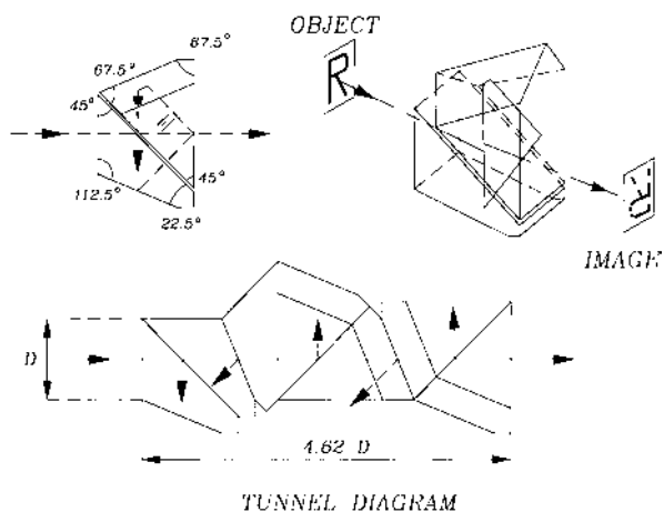
Figure 10.17 Schmidt-Pechan prism.
