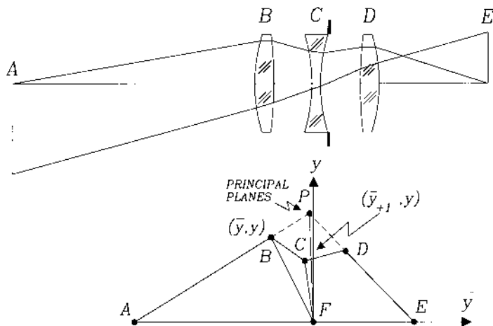
Figure 3.17 A y - \bar{y} diagram of a triplet, used to find the area of triangle ABC.
