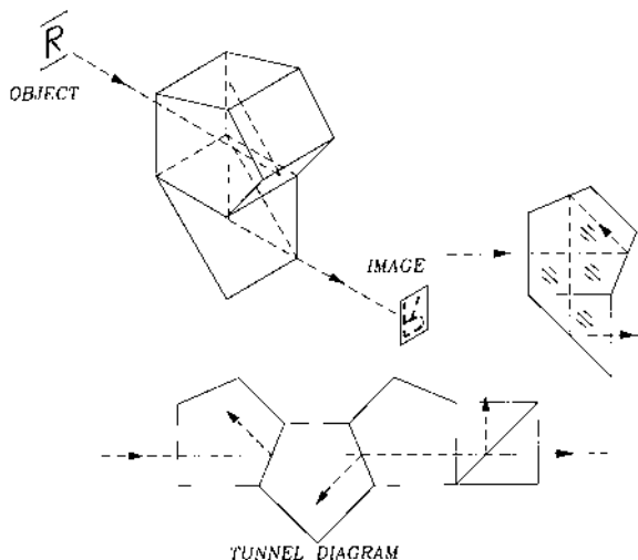
Figure 10.14 Reverting-inversing prism.
