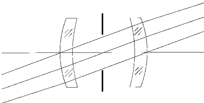
Figure 11.17 Periscopic lens.
