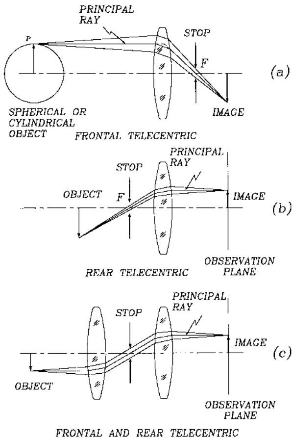
Figure 1.27 Telecentric lenses.
