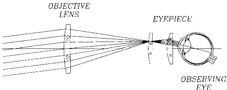
Figure 15.5 Telescope with an eyepiece having a field lens.
