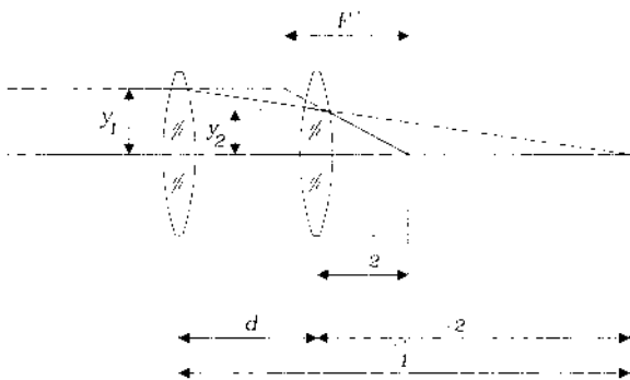
Figure 3.11 A system of two separated thin lenses.
