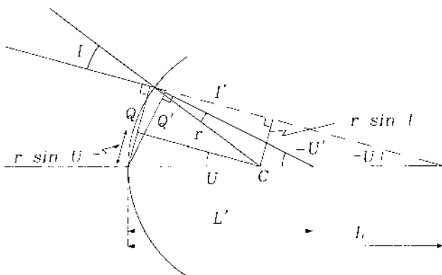
Figure 1.15 Meridional ray tracing by the Q - U method.
