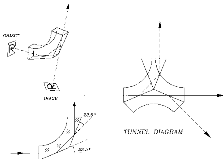
Figure 10.6 Wollaston prism.
