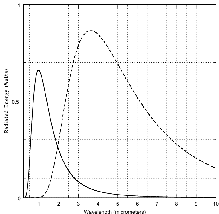
Figure 15.7: The energy vs. wavelength, the “spectra” (spectra is plural of spectrum), produced by two blackbodies with different temperatures.
