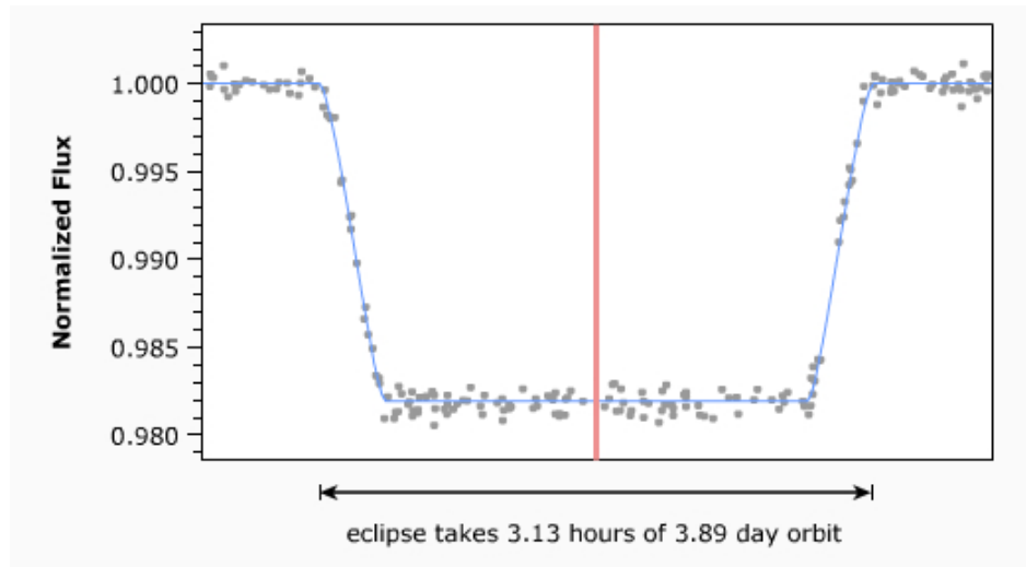
Figure 18.12: Transiting exoplanet #3.
