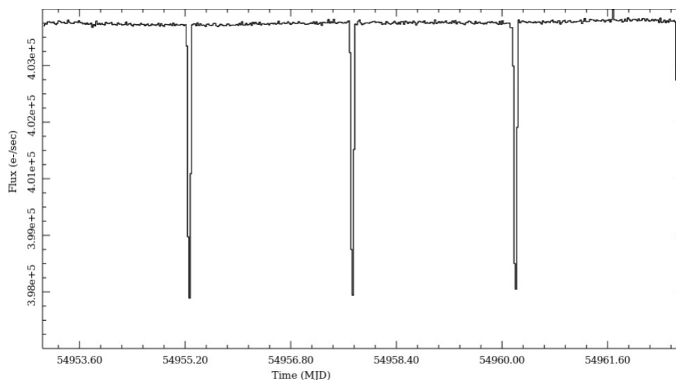
Figure 18.9: The light curve of Kepler 1b as measured by the Kepler satellite. The numbers on the y-axis are the total counts (how much light was measured), while the x-axis is “modified Julian days”. This is a system that simply makes it easy to figure out periods of astronomical events since it is a number that increases by 1 every day (instead of figuring out how many days there were between June 6 th and November 3 rd ). Thus, to get an orbital period you just subtract the MJD of one event from the MJD of the next event.
