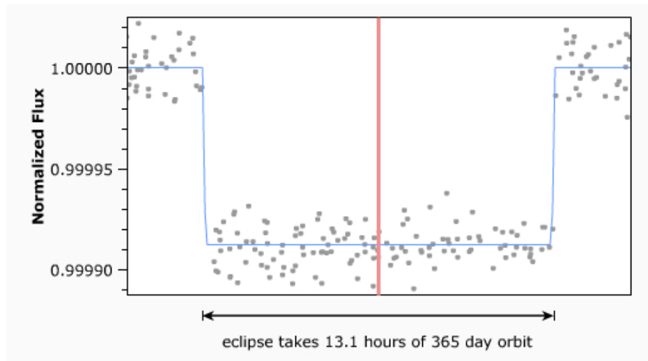
Figure 18.13: Transiting exoplanet #4.
