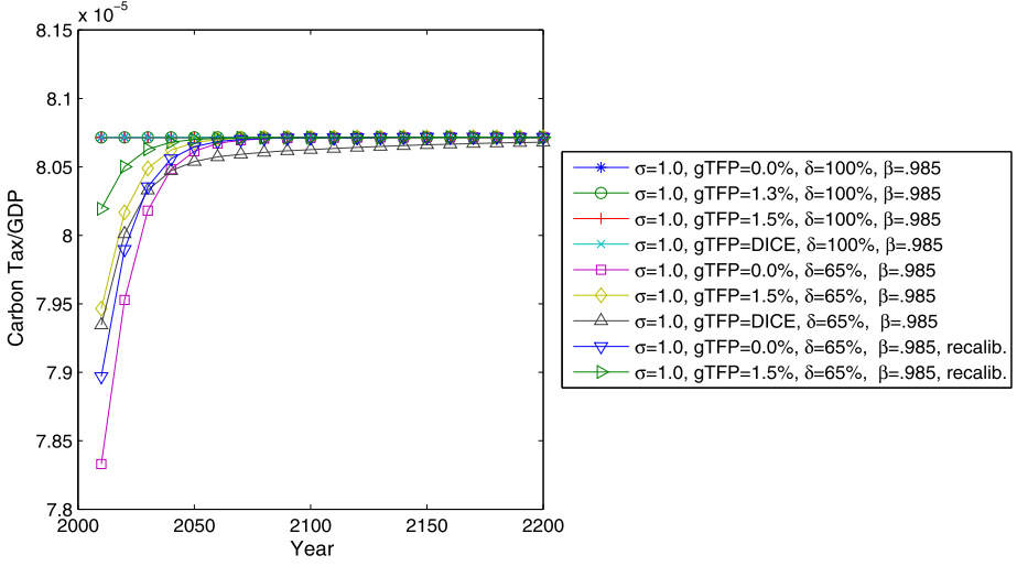
FIGURE S.4.—Carbon tax/GDP ratio, \sigma = 1 .
