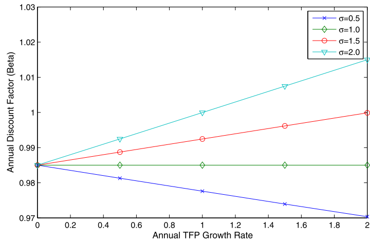
FIGURE S.15.—Annual discount factor for benchmark carbon tax/GDP approximation.
