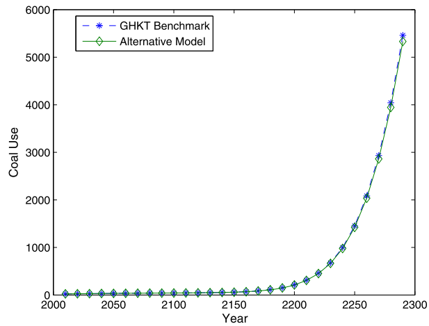
FIGURE S.18.—Coal use comparison: GHKT benchmark vs. alternative model.
