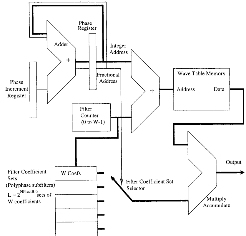
Figure 8.9 A sampling playback oscillator using high order interpolation. Every output sample is a vector dot product of W input samples and one of the filter coefficient vectors, stored re-ordered from the original prototype filter. The fractional phase address selects the filter coefficient vector used.
