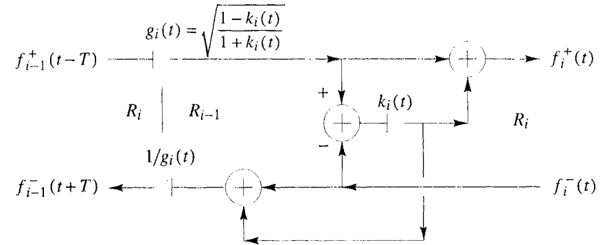
Figure 10.10 A three-multiply normalized scattering junction.
