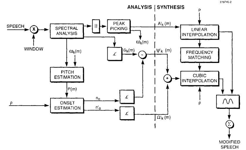
Figure 9.13 Analysis/synthesis for time-scale modification. (Reprinted with permission from [Quatieri and McAulay, 1992], © 1992, IEEE)
