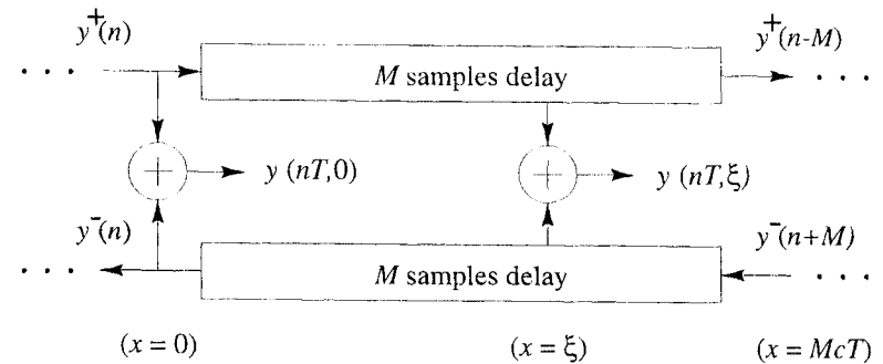
Figure 10.4 Conceptual diagram of interpolated digital waveguide simulation.
