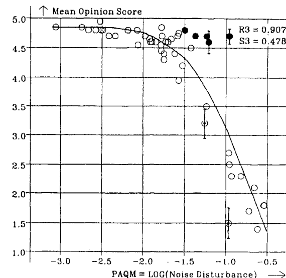
Figure 1.9 Relation between the mean opinion score (MOS) and the perceptual audio quality measure (PAQM) for the 50 items of the ISO/MPEG 1991 codec test [ISO91, 1991] in loudspeaker presentation. The filled circles are items whose quality was judged significantly lower by the model than by the subjects.
