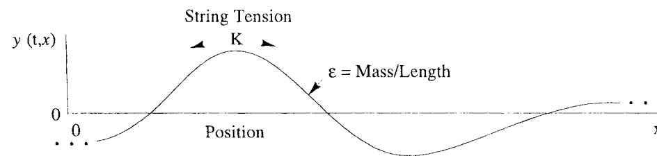
Figure 10.1 The ideal vibrating string.
