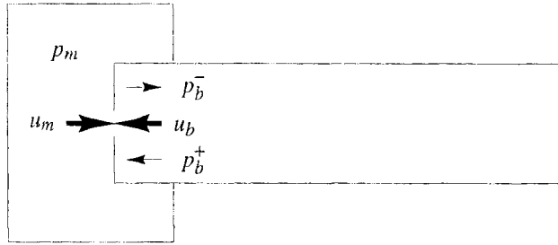
Figure 10.18 Schematic diagram of mouth cavity, reed aperture, and bore.
