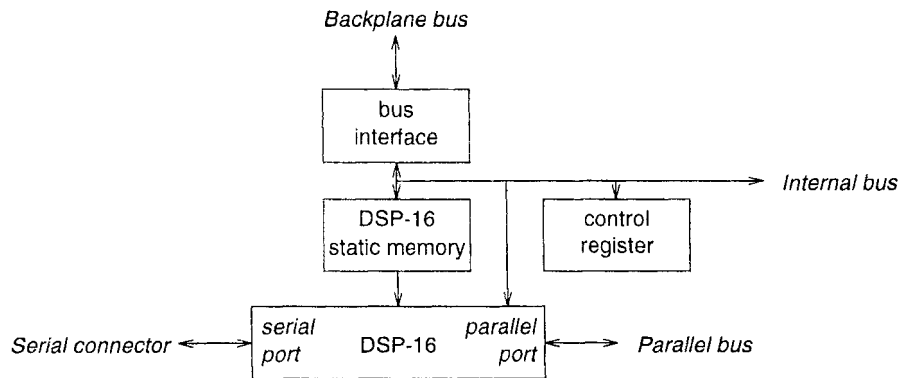
Figure 5.19 Gmusic core block diagram
