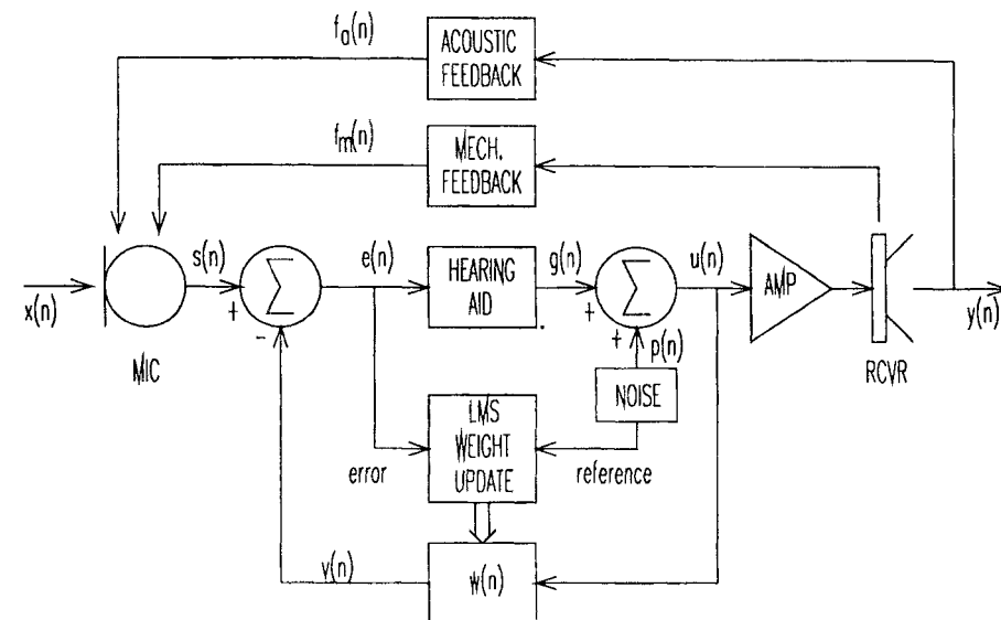
Figure 6.13 Block diagram of a hearing aid incorporating signal processing for feedback cancellation
