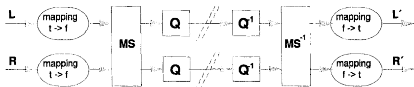
Figure 2.14 Basic block diagram of M/S stereo coding (Reprinted from [Herre, 1995] © 1995, courtesy of the author)
