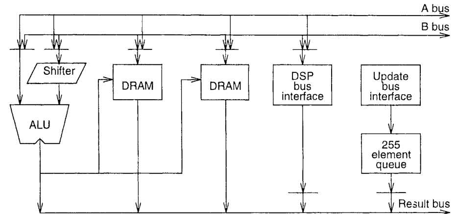
Figure 5.12 Lucasfilm ASP interconnect and memory diagram
