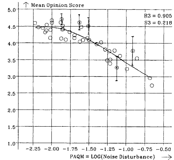
Figure 1.15 Relation between MOS and cognitive corrected PAQM ( PAQM_{C1.4} ) for the 43 ISO layer II tandeming conditions of the ITU-R TG10/2 1993 [ITURsg10cond9343, 1993] audio codec test.
