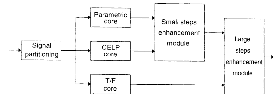
Figure 2.21 MPEG-4 audio scaleable configuration
