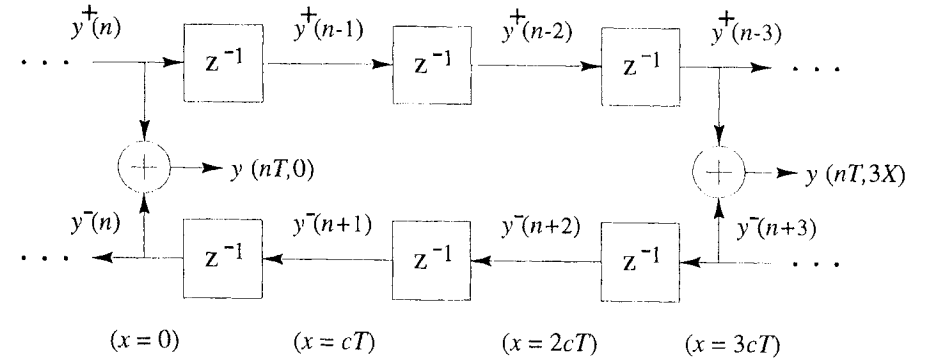
Figure 10.3 Digital simulation of the ideal, lossless waveguide with observation points at x = 0 and x = 3X = 3cT .
