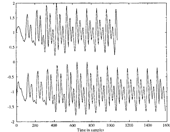
Figure 7.9 Time-domain representation of an original speech signal (top), and of its time-stretched version (bottom), showing shape invariance. Time-domain modification technique.
