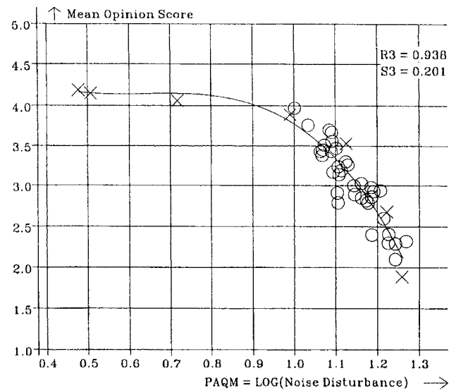
Figure 1.16 Relation between the MOS and the cognitive corrected PAQM ( PAQM_{C4.0, W0.1} ) for the ETSI GSM full rate speech database. Crosses represent data from the experiment based on the modulated noise reference unit, circles represent data from the speech codecs.
