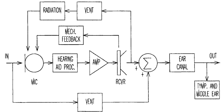
Figure 6.12 Block diagram of an ITE hearing aid inserted into the ear canal
