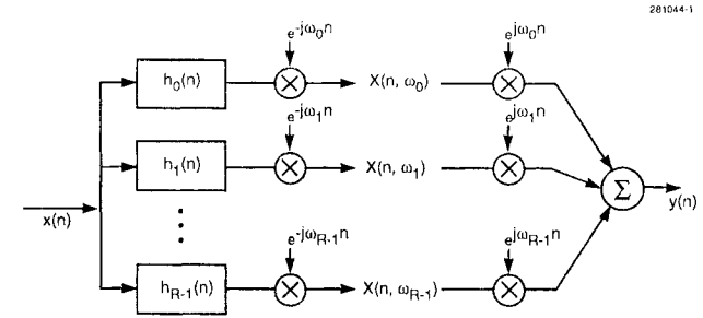
Figure 9.2 Phase vocoder based on filter bank analysis/synthesis.
