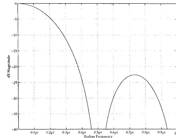
Figure 8.8 Frequency response of a linear interpolation sample rate converter with L = 4 showing better stopband rejection around 0.5\pi (or at the original Nyquist rate) but increased rolloff in the passband below 0.25\pi of almost -7 dB.
