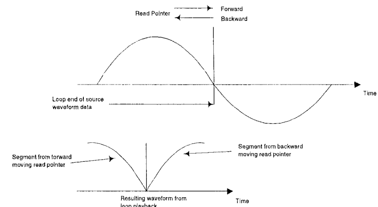
Figure 8.12 Backwards forwards loop at a loop point with odd symmetry.
