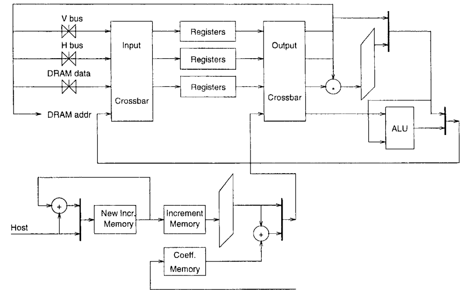
Figure 5.16 Sony OXF DSP block diagram
