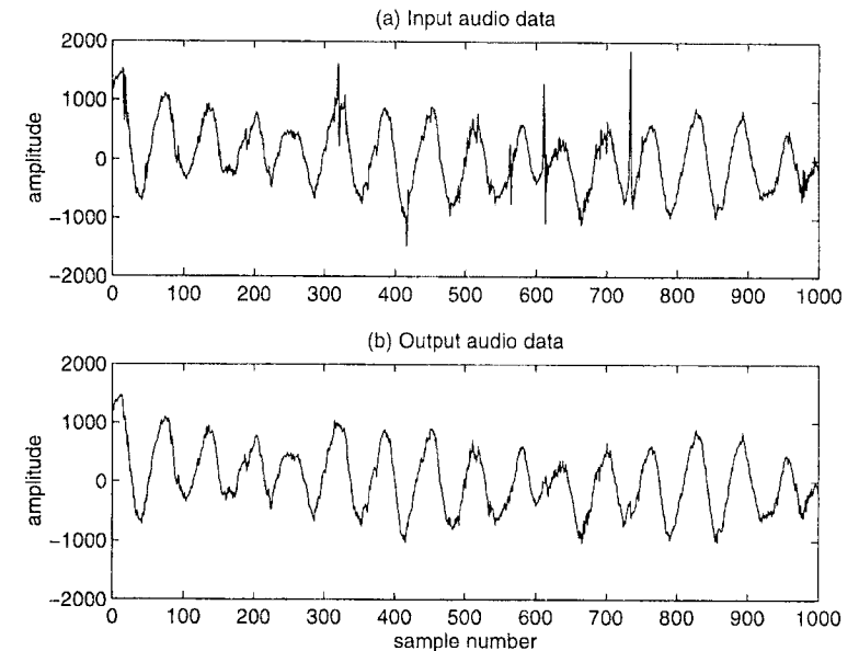
Figure 4.8 Restoration using Bayesian iterative methods
