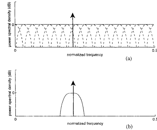
Figure 4.17 Restoration of a sinusoidal signal embedded in white noise (of power 0 dB). (a) The noisy signal (the dotted lines feature the filter bank characteristics); (b) The processed signal.
