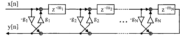
Figure 3.18 Lattice allpass structure.
