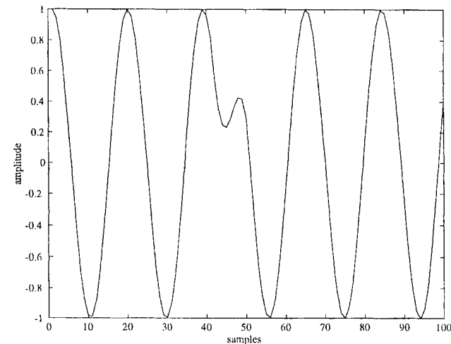
Figure 7.6 Time-scale modification of a sinusoid.
