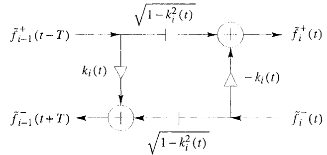
Figure 10.9 The normalized scattering junction.
