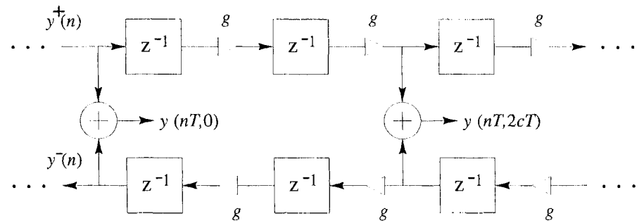
Figure 10.12 Discrete simulation of the ideal, lossy waveguide.
