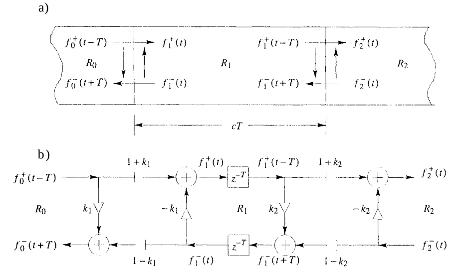
Figure 10.6 A waveguide section between two partial sections. a) Physical picture indicating traveling waves in a continuous medium whose wave impedance changes from R_0 to R_1 to R_2 . b) Digital simulation diagram for the same situation. The section propagation delay is denoted as z^{-T} . The behavior at an impedance discontinuity is characterized by a lossless splitting of an incoming wave into transmitted and reflected components.
