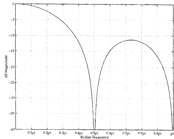
Figure 8.7 Digital Sinc function – the frequency response for a zero order hold interpolator sample rate converter with L = 4 , which puts the original Nyquist frequency at 0.25\pi . We can see rolloff in the passband of about -3.9 dB and very poor rejection of images outside of the passband, which result in artifacts perceived as pitch shifting distortion.
