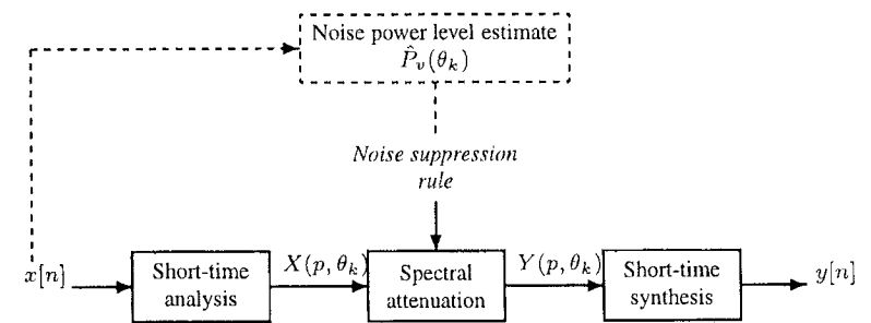
Figure 4.15 Background noise suppression by short-time spectral attenuation
