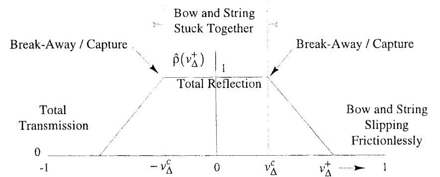
Figure 10.23 Simple, qualitatively chosen bow table for the digital waveguide violin.
