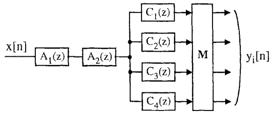
Figure 3.15 Mixing matrix \mathbf{M} used to form uncorrelated outputs from parallel comb filters [Schroeder, 1962]. A_i(z) are allpass filters, and C_i(z) are comb filters.
