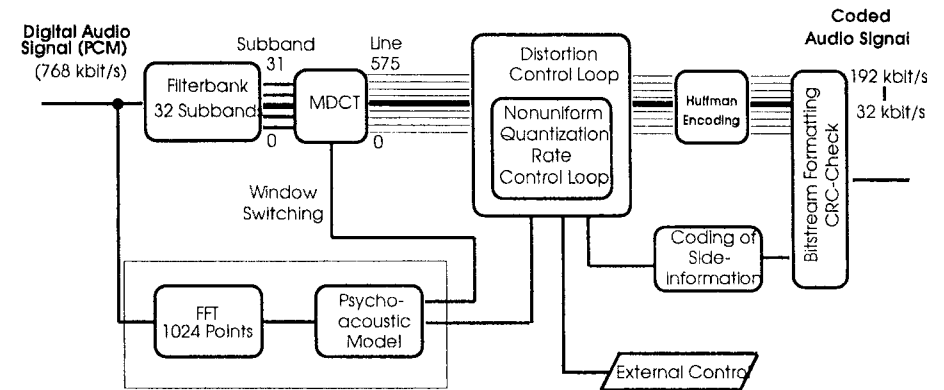
Figure 2.18 Block diagram of an MPEG-1 Layer 3 encode
