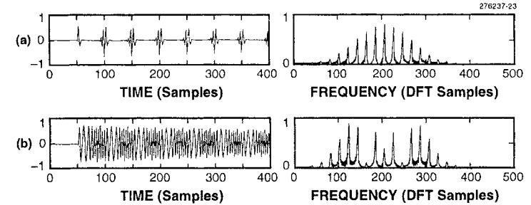
Figure 9.30 Comparison of Equation (9.82) and (9.86) for parameter settings \omega_c = 2000 , \omega_m = 200 , and I = 5.0 : (a) Equation (9.86); (b) Equation (9.82). (Both waveforms and spectra are illustrated.)
