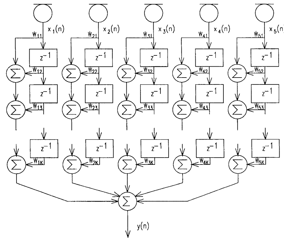
Figure 6.20 Block diagram of a time-domain five-microphone adaptive array.
