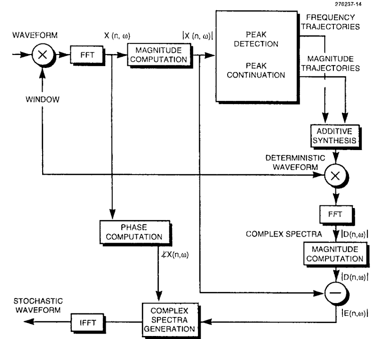
Figure 9.20 Block diagram of the deterministic plus stochastic system.
