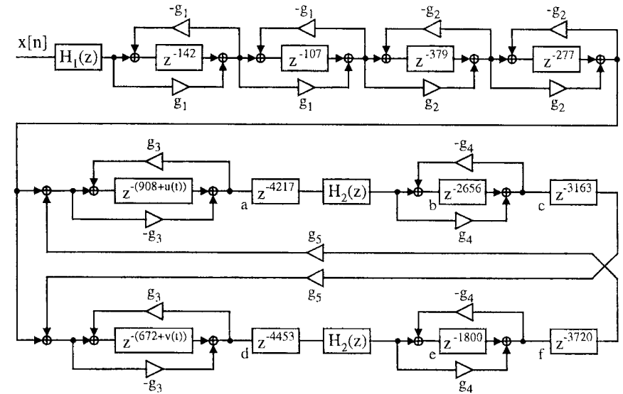
Figure 3.21 Dattorro's plate reverberator based on an allpass feedback loop, intended for 29.8 kHz sampling rate [Dattorro, 1997]. H_1(z) and H_2(z) are lowpass filters described in figure 3.11; H_1(z) controls the bandwidth of signals entering the reverberator, and H_2(z) controls the frequency dependent decay. Stereo outputs y_L and y_R are formed from taps taken from labelled delays as follows: y_L = a[266] + a[2974] - b[1913] + c[1996] - d[1990] - e[187] - f[1066] , y_R = d[353] + d[3627] - e[1228] + f[2673] - a[2111] - b[335] - c[121] . In practice, the input is also mixed with each output to achieve a desired reverberation level. The time varying functions u(t) and v(t) are low frequency ( \approx 1 Hz) sinusoids that span 16 samples peak to peak. Typical coefficients values are g_1 = 0.75 , g_2 = 0.625 , g_3 = 0.7 , g_4 = 0.5 , g_5 = 0.9 .
