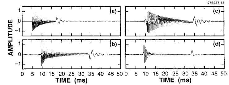
Figure 9.18 Time-scale expansion ( \times 2 ) using subband phase correction; (a) Original; (b) Expansion with phase correction at 5ms; (c) with phase correction in clustered subbands; (d) without phase correction. (Reprinted with permission from [Quatieri et al., 1995], © 1995, IEEE)
