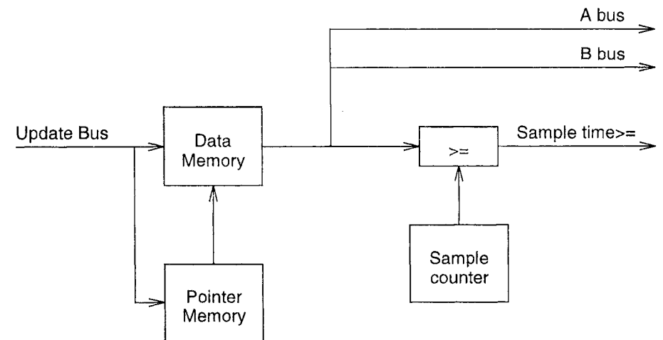
Figure 5.13 Moorer's update queue data path
