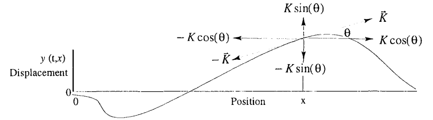
Figure 10.5 Transverse force propagation in the ideal string.
