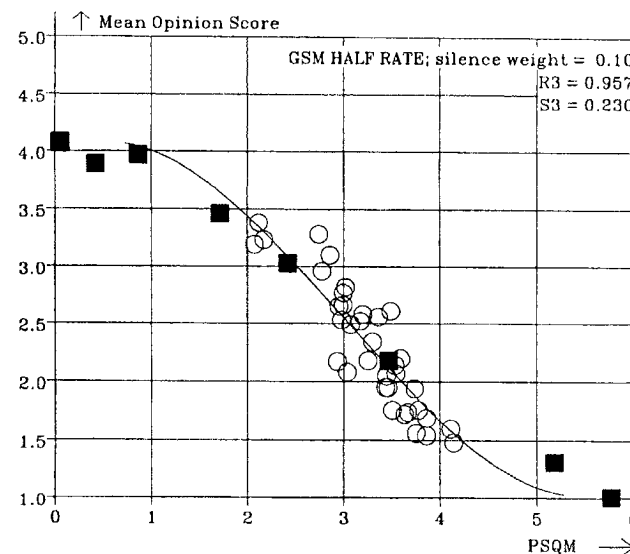
Figure 1.19 The same as Fig. 1.18 but for the ETSI GSM half rate speech database using the PSQM.
