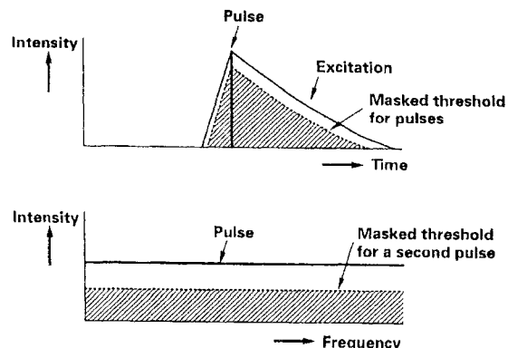
Figure 1.3 From the masking pattern it can be seen that the excitation produced by a click is smeared out in the time domain.
