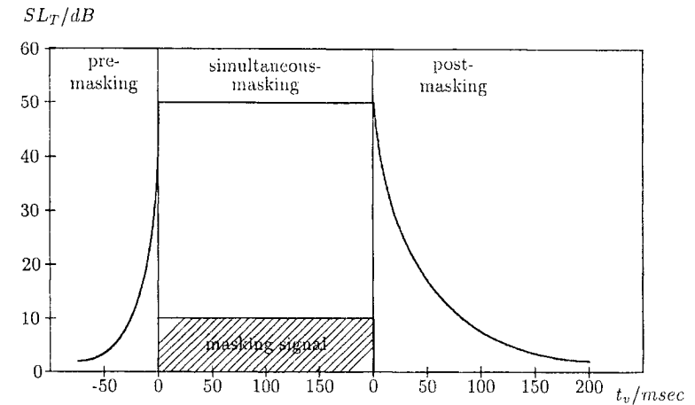
Figure 2.2 Example of pre-masking and post-masking (according to [Zwicker, 1982]) (Reprinted from [Sporer, 1998] ©1998, courtesy of the author)
