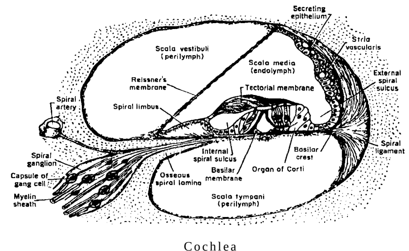
Figure 6.2 Features of the cochlea: transverse cross-section of the cochlea (Reprinted with permission from [Rasmussen, 1943], ©1943, McGraw-Hill)
