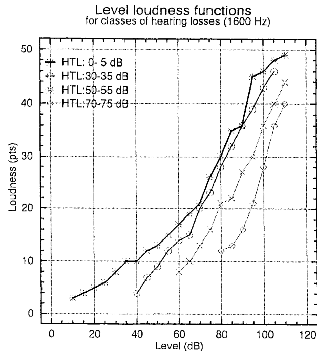
Figure 6.6 Loudness level functions on a 50-point rating scale for different classes of hearing loss.
