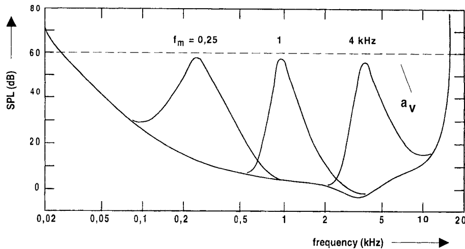
Figure 2.1 Masked thresholds: Masker: narrow band noise at 250 Hz, 1 kHz, 4 kHz (Reprinted from [Herre, 1995] ©1995, courtesy of the author)
