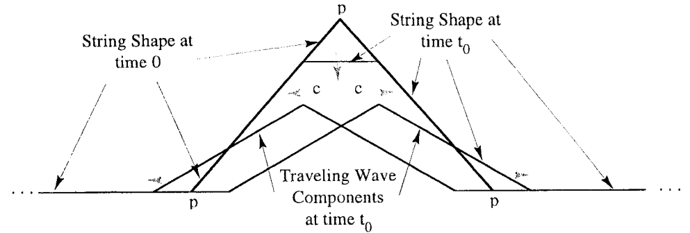
Figure 10.2 An infinitely long string, “plucked” simultaneously at three points, labeled “p” in the figure, so as to produce an initial triangular displacement. The initial displacement is modeled as the sum of two identical triangular pulses which are exactly on top of each other at time 0. At time t_0 shortly after time 0, the traveling waves centers are separated by 2ct_0 meters, and their sum gives the trapezoidal physical string displacement at time t_0 which is also shown. Note that only three short string segments are in motion at that time: the flat top segment which is heading to zero where it will halt forever, and two short pieces on the left and right which are the leading edges of the left- and right-going traveling waves. The string is not moving where the traveling waves overlap at the same slope. When the traveling waves fully separate, the string will be at rest everywhere but for two half-amplitude triangular pulses heading off to plus and minus infinity at speed c .
