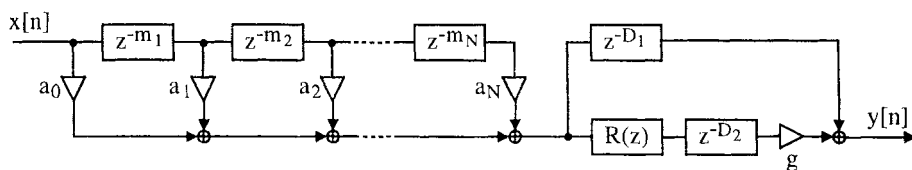
Figure 3.7 FIR filter cascaded with reverberator R(z) [Moorer, 1979].
