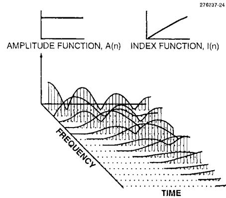
Figure 9.29 Spectral dynamics of FM synthesis with linearly changing modulation index I(n) . (Reprinted with permission from [Moorer, 1977], © 1977, IEEE)
