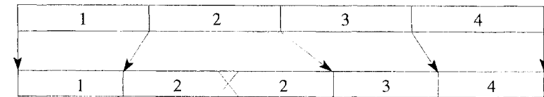
Figure 7.4 Pitch modification with the sampling technique. The segments are resampled (here to a lower sampling rate) and possibly repeated (as segment 2), giving the output signal the same duration as the input signal.
