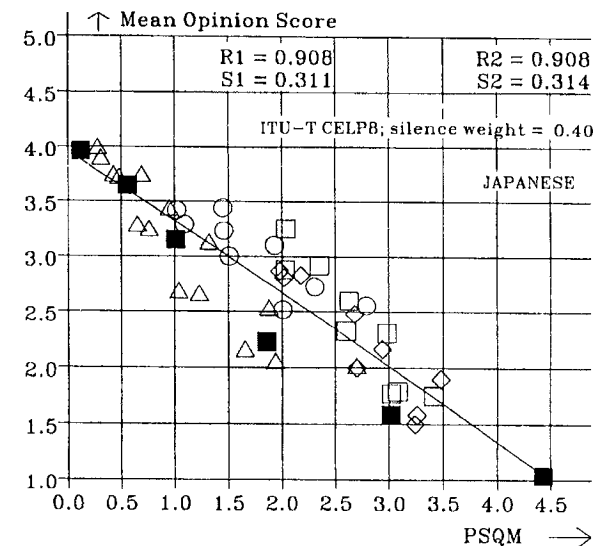
Figure 1.21 The same as Fig. 1.20 but for the Japanese language.
