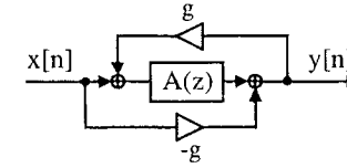
Figure 3.19 Generalization of figure 3.18.
