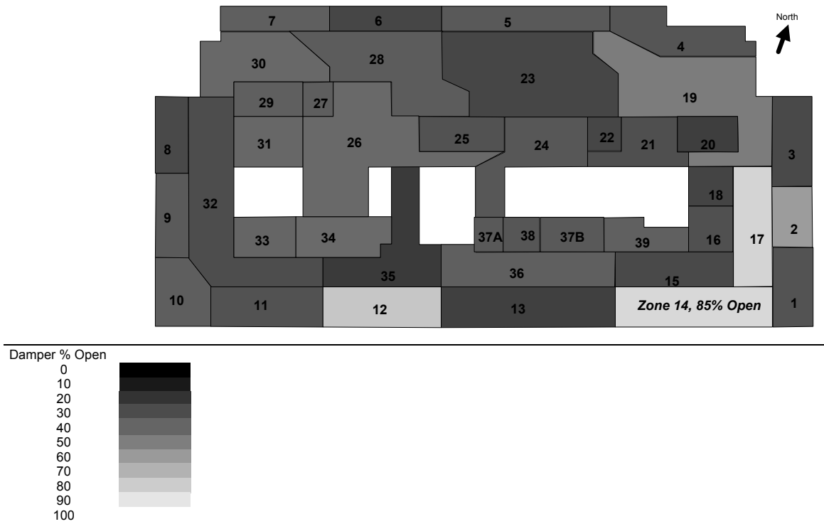
Figure 24. Site 3 VAV Box Demand, 7am Monday August 5, 2002
