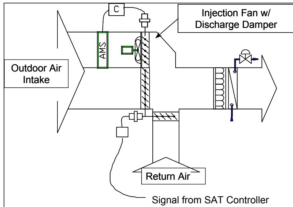
Figure 93. Injection Fan with Dedicated Minimum outdoor air Damper
