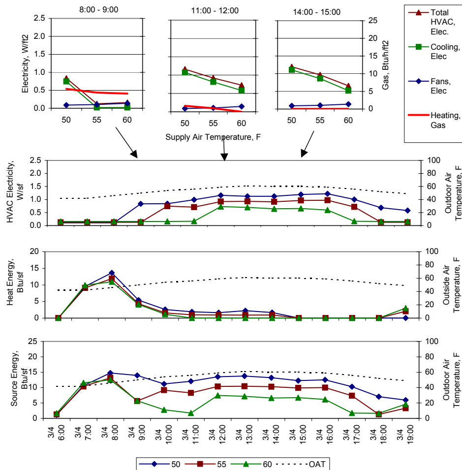
Figure 39 – Comparison of Mild Day Simulation Results for Three Supply Air Temperature Setpoints: 50°F, 55°F, and 60°F. March 4, Sacramento Climate.
