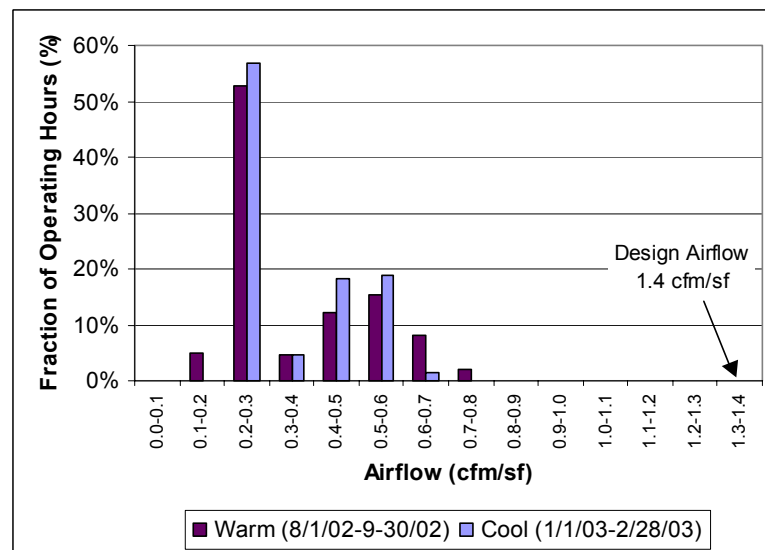
Figure 123. Total System Airflow, Site 1
