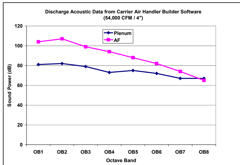
Figure 66. Case Study A – Carrier Acoustic Data (With Casing)
