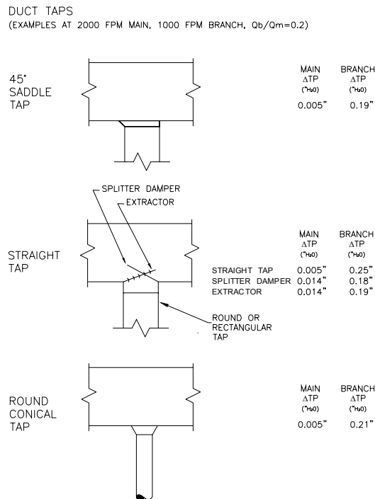
Figure 34. Pressure Drop Through Duct Taps
