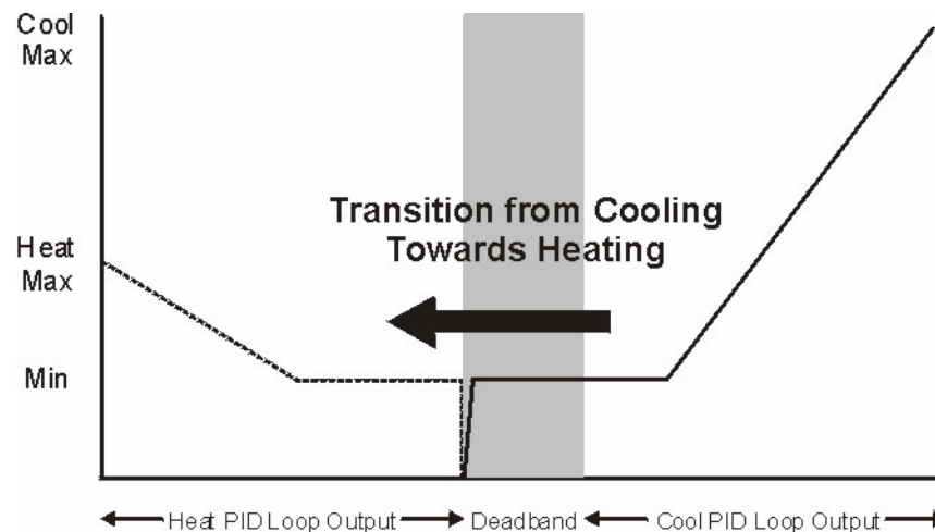
Figure 27. Dual Duct - From Cooling to Heating
