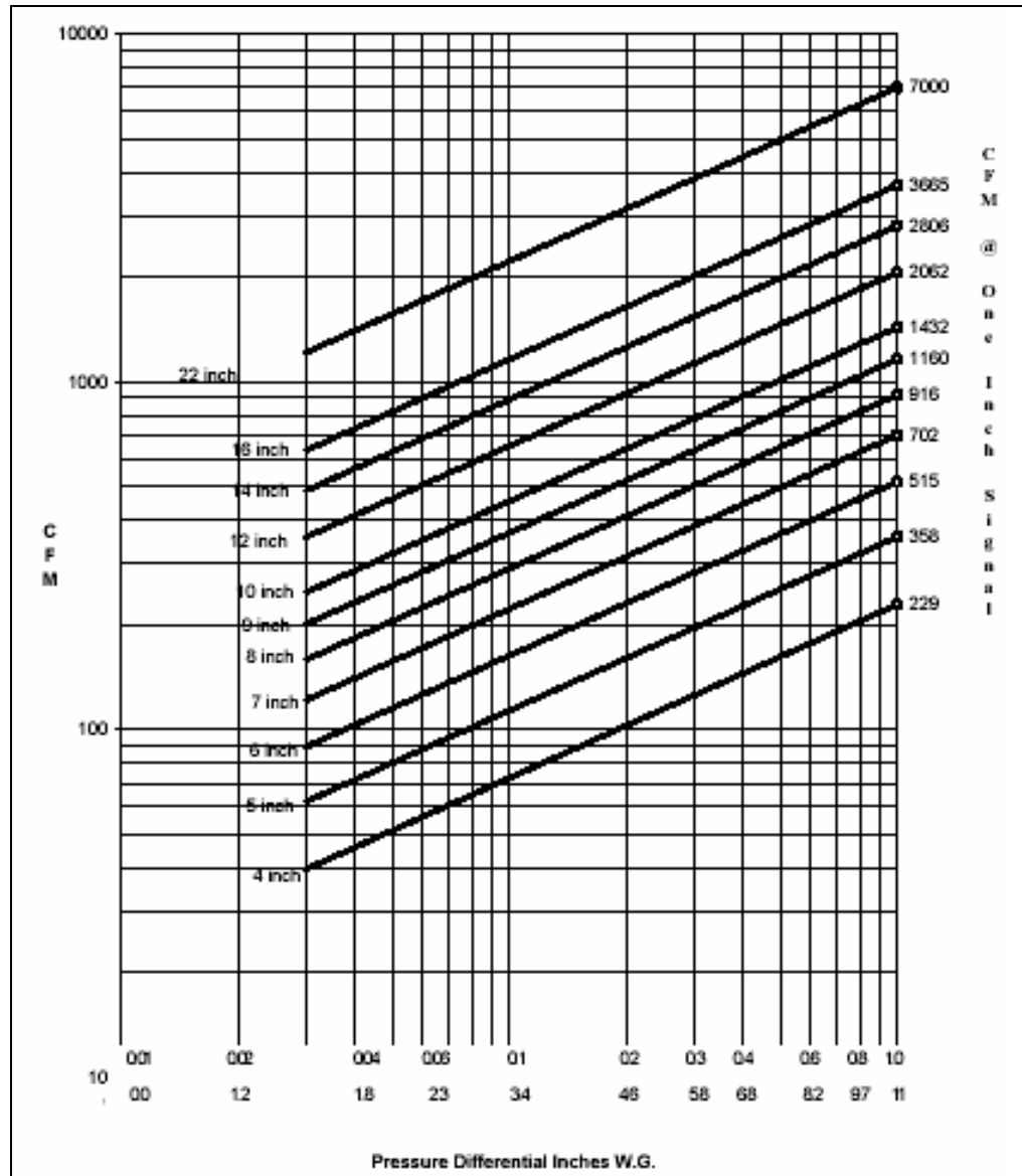
Figure 23. Sample VAV Box Inlet Sensor Performance Chart, CFM vs. Velocity Pressure Signal
