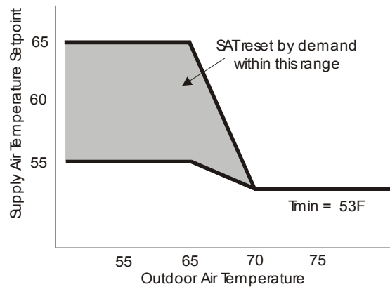
Figure 40. Recommended Supply Air Temperature Reset Method
