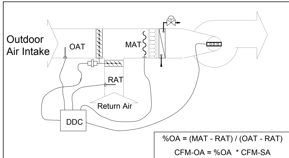
Figure 90. Energy Balance Method of Controlling Minimum outdoor air
