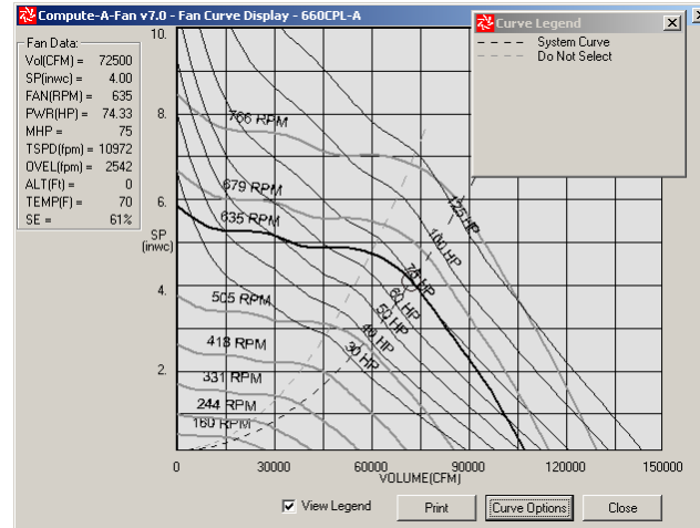
Figure 70. Case Study B – 66” Plenum Fan Curve
