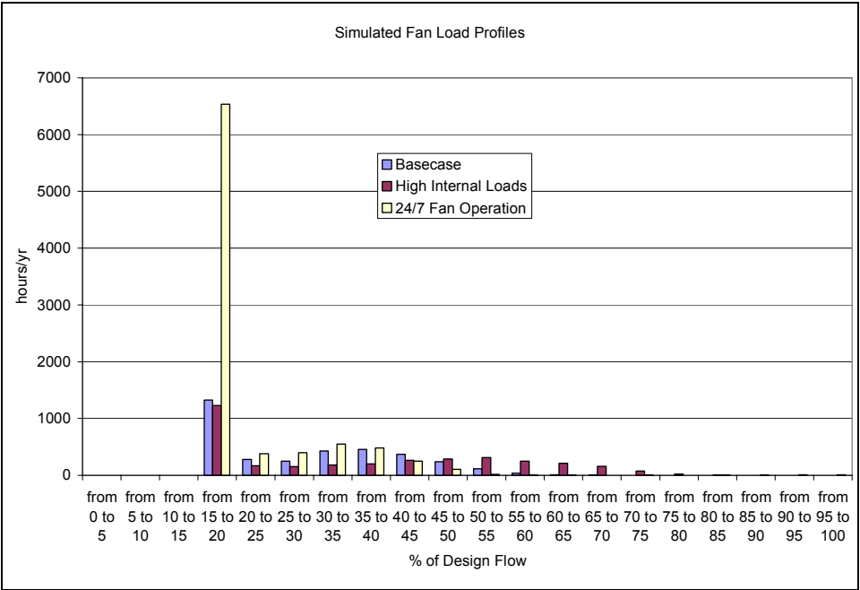
Figure 62. Case Study A - Load Profiles
