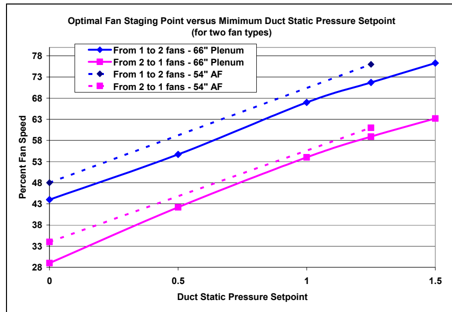
Figure 85. Optimal Staging Point for Two Fan Types
