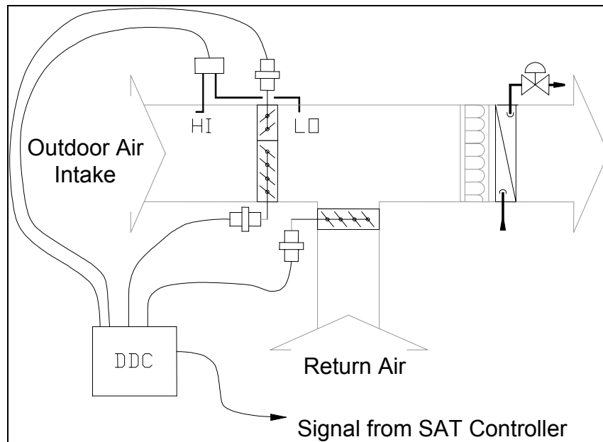
Figure 94. Minimum outdoor air Damper With Pressure Control
