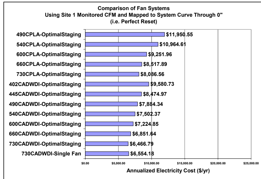
Figure 75. Case Study B Simulation Results - Perfect Static Pressure Reset
