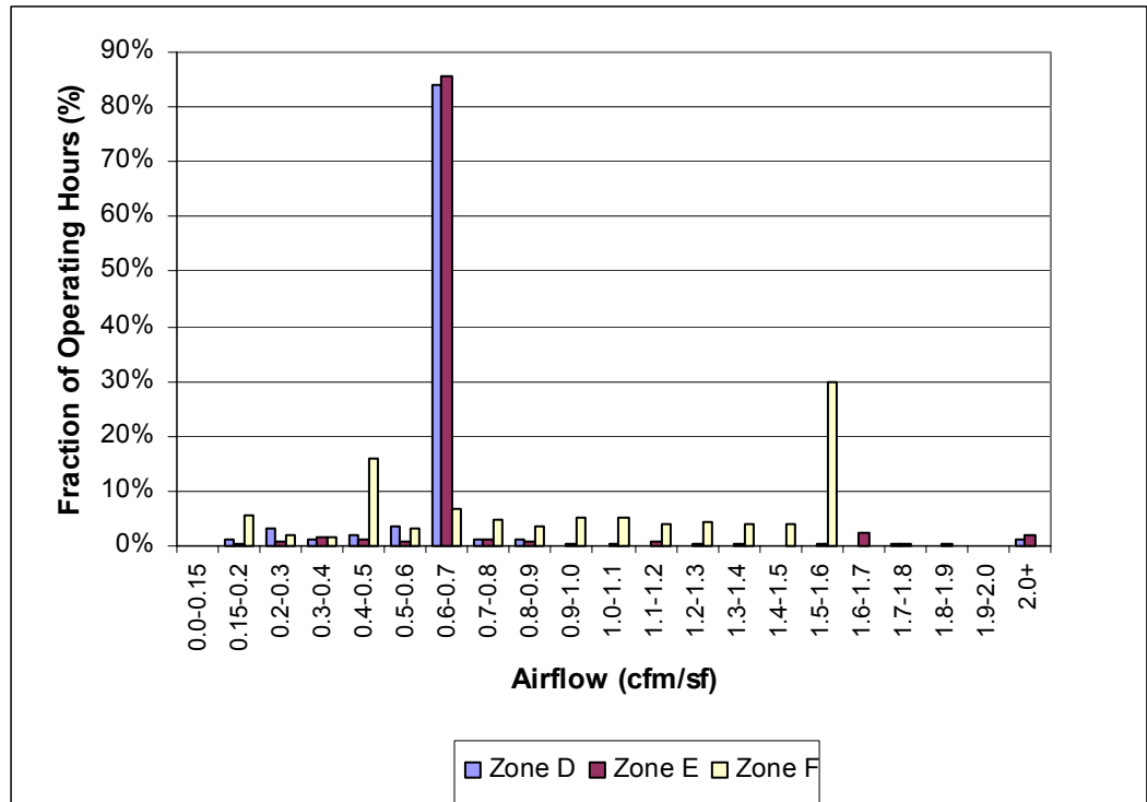
Figure 120. Site 3, Sample of Perimeter Zones, Warm Period (8/8/02 - 9/7/02)
