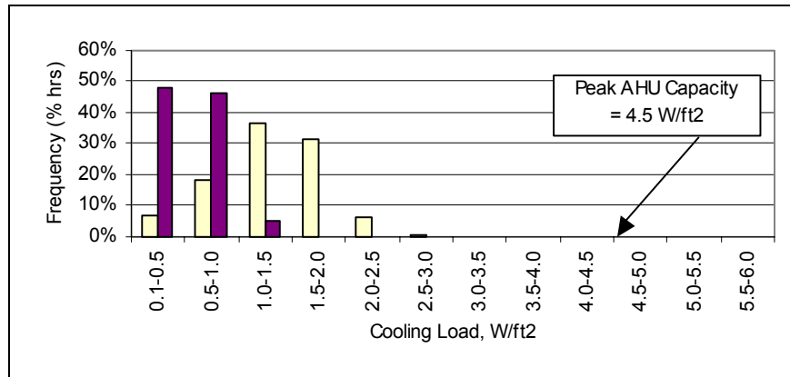
Figure 129. Site 3 (Light bar includes Aug-Oct 2002, dark bar covers Nov 2002 – Jan 2003)
