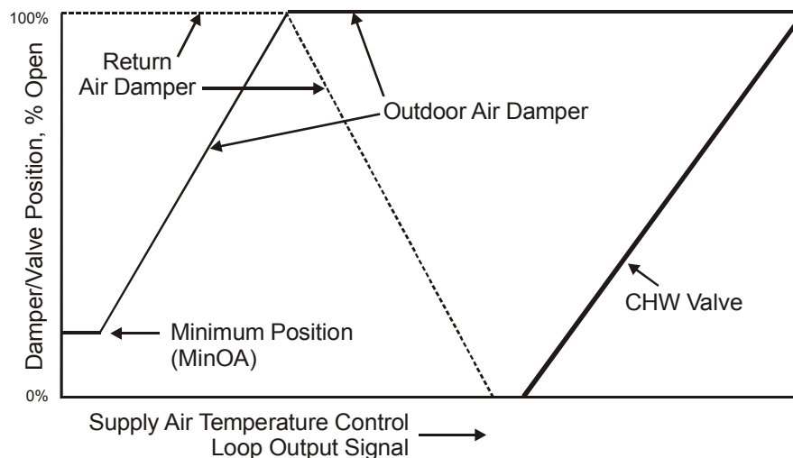
Figure 98. Airside Economizer Control Staging from ASHRAE Guideline 16-2003
