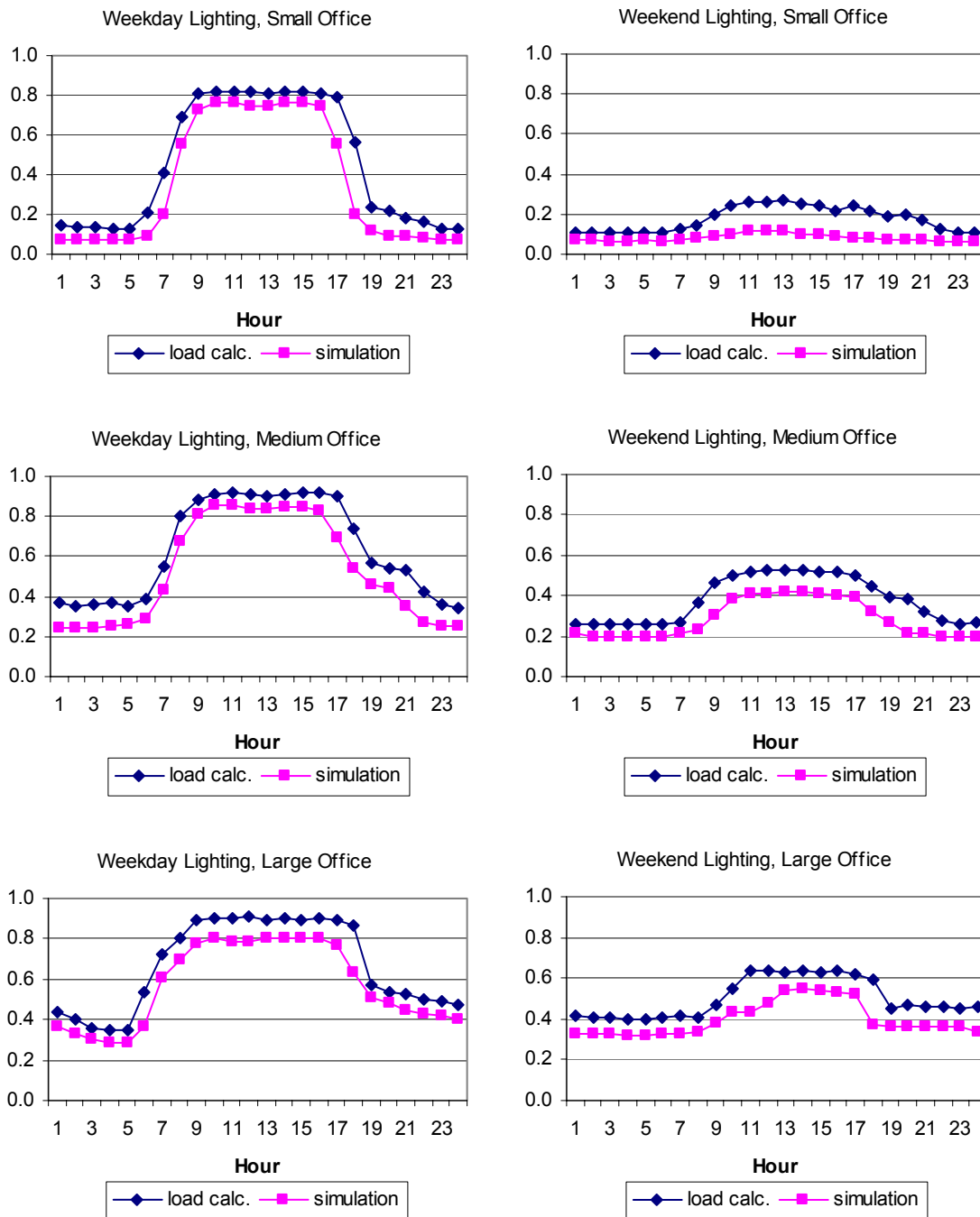
Figure 10. Measured Lighting Schedules (90 th percentile for design load calculation and 50 th percentile for energy simulations) for Small, Medium and Large Office Buildings – ASHRAE 1093-RP.
