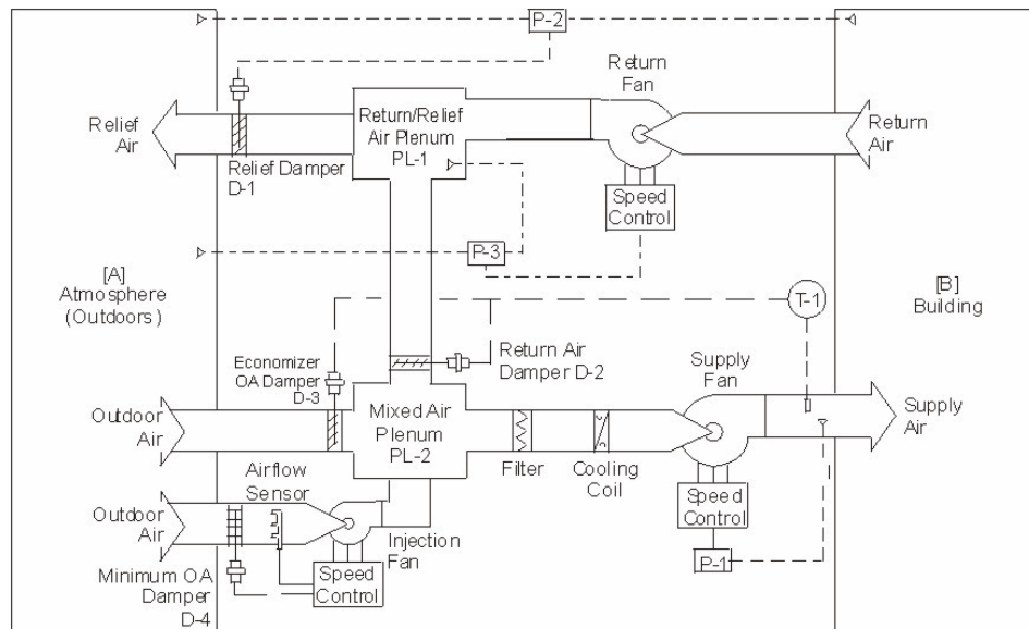
Figure 97. Airside Economizer Configuration with Return Fan from ASHRAE Guideline 16-2003
