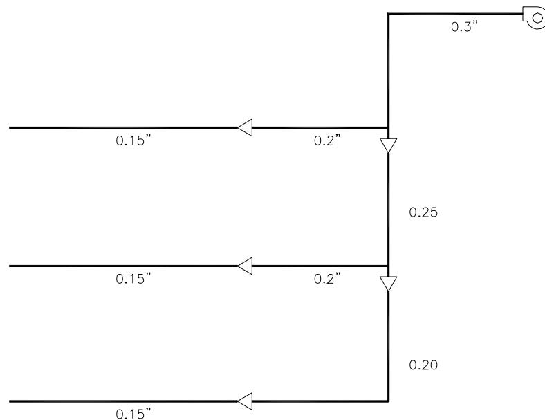
Figure 35. Example of Duct Sizing Using the Friction Rate Reduction Method
