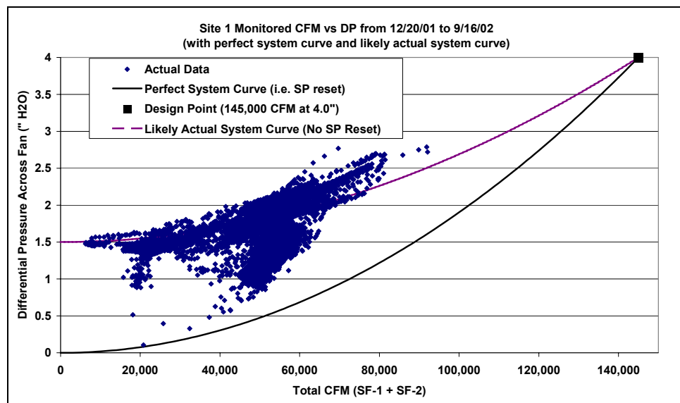
Figure 71. Case Study B - Monitored Data
