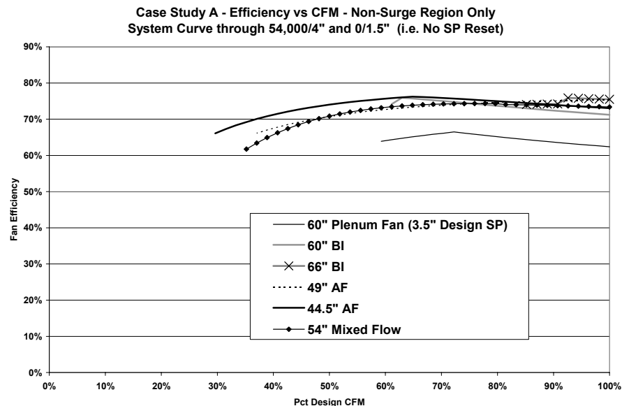
Figure 59. Case Study A - Part Load Efficiency (Non-surge Region Only)
