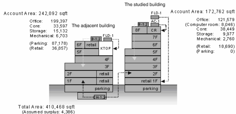
Figure 111. Buildings Summary (Source: Naoya Motegi, LBNL)
