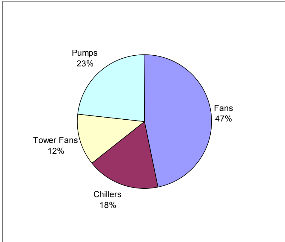
Figure 102. Site 1, Monitored HVAC Electricity End Uses
