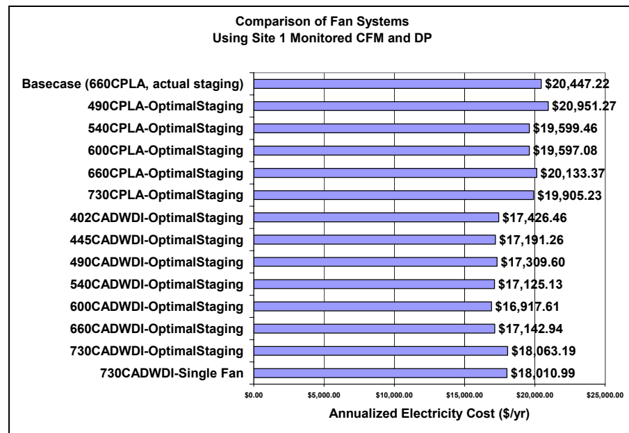
Figure 74. Case Study B Simulation Results - No Static Pressure Reset
