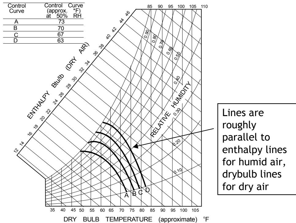
Figure 99. Electronic Enthalpy High Limit Controller.
