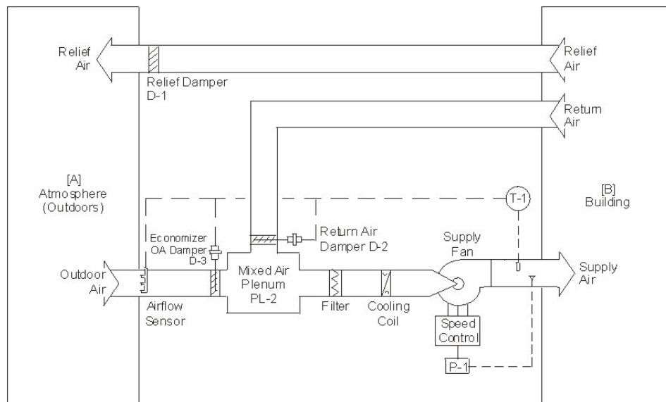
Figure 95. Airside Economizer Configuration with Barometric Relief from ASHRAE Guideline 16-2003
