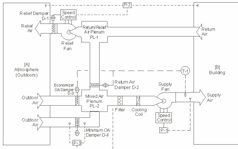
Figure 96. Airside Economizer Configuration with Relief Fan from ASHRAE Guideline 16-2003
