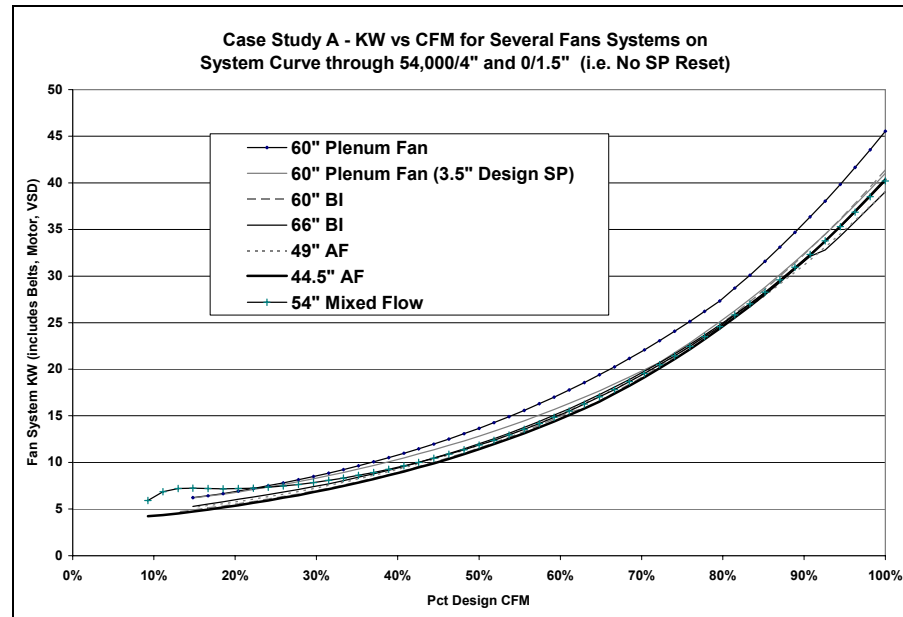
Figure 60. Case Study A - kW versus CFM
