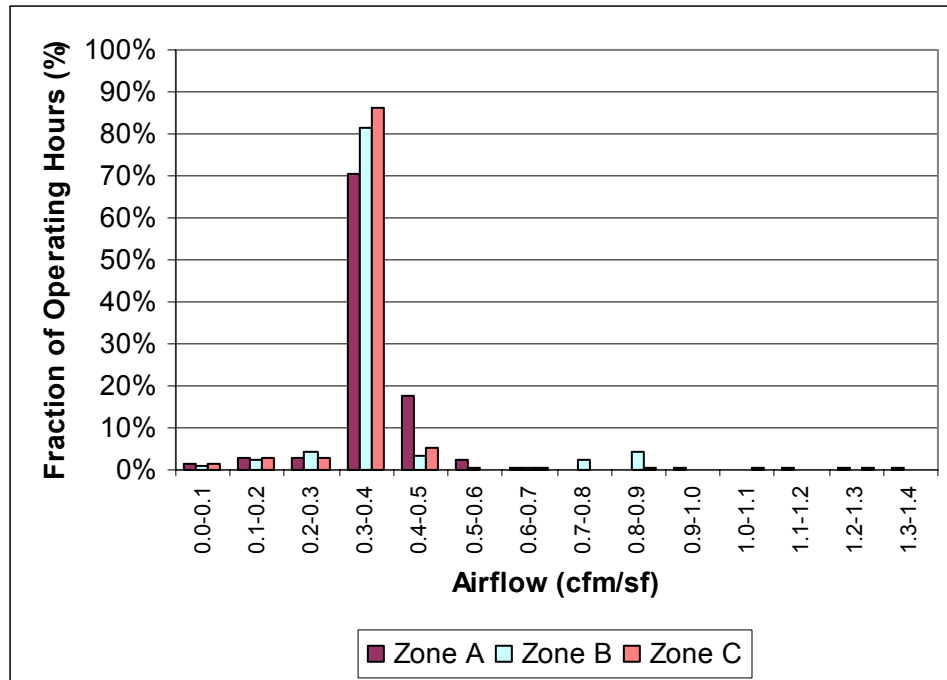
Figure 117. Site 3, Sample of Interior Zones, Warm Period (8/8/02 - 9/7/02)
