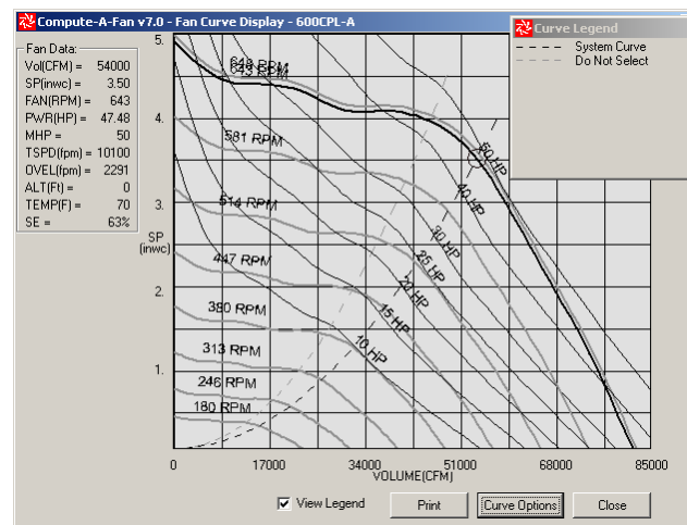
Figure 41. A Typical Manufacturer's Fan Curve (60" Plenum Fan)
