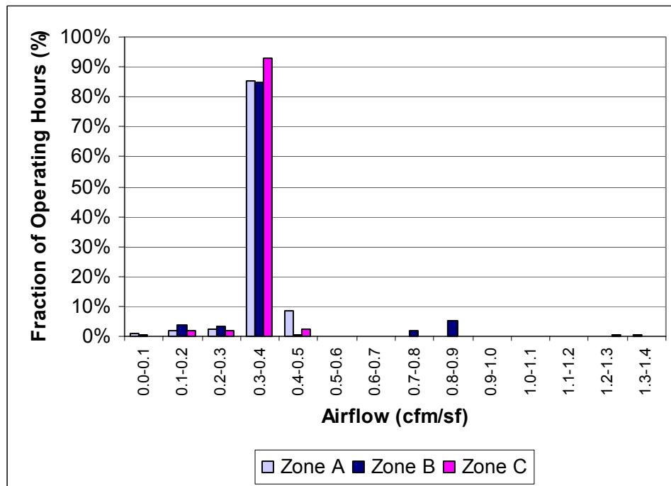
Figure 118. Site 3, Sample of Interior Zones, Cool Period (12/12/02-1/11/03)
