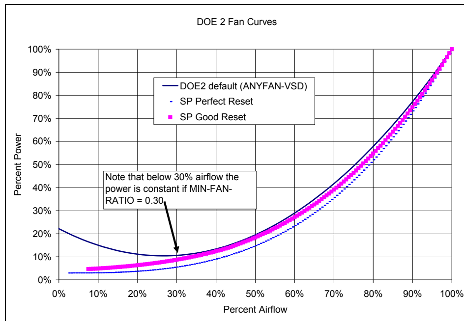
Figure 132. Fan Performance Curves for Simulation
