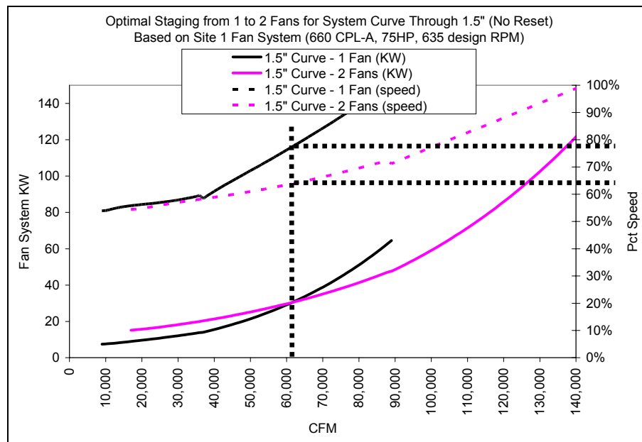
Figure 82. Optimal Staging (No Static Pressure Reset)
