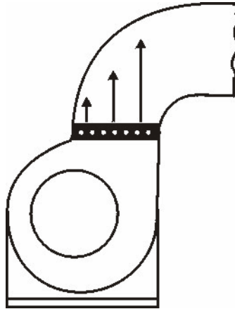
Figure 36. Poor Discharge Configuration Resulting in Significant Fan System Effect
