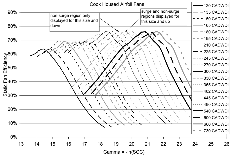
Figure 47. Gamma Curves for All Cook Housed Airfoil Fans
