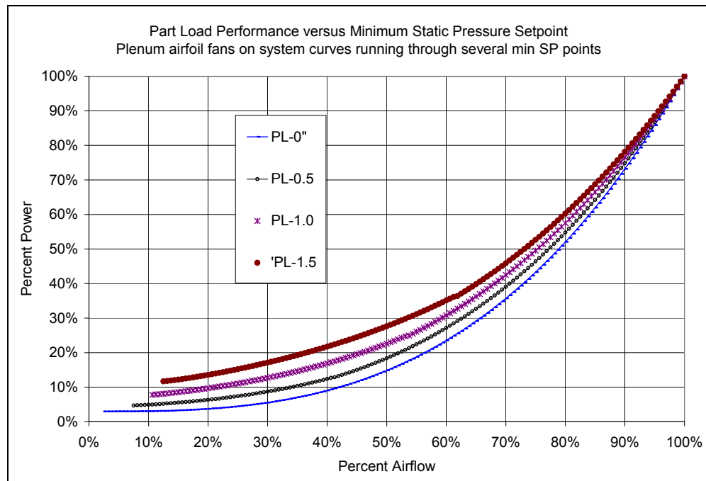
Figure 80. SP Setpoint vs Fan System Energy
