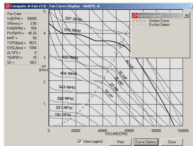
Figure 54. Case Study A - 66" Plenum Fan Design Point
