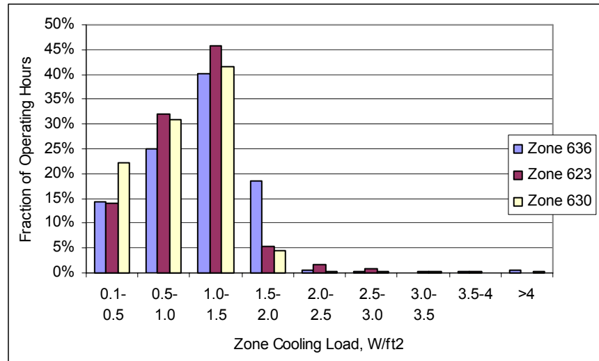
Figure 108 – Monitored Cooling Loads for a Sample of Three Interior Zones, Site 3 (Office)
