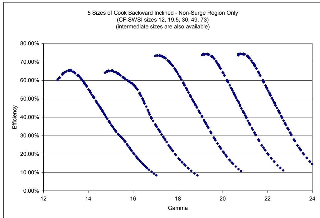
Figure 49. Gamma Curves for Some Cook Backward Inclined Fans
