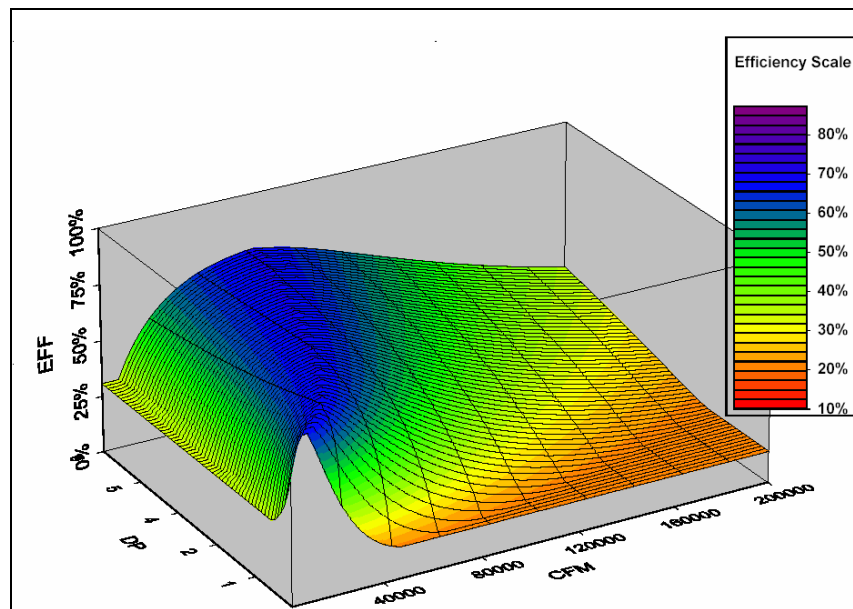
Figure 43. Three-Dimensional Fan Curve for 49" Housed Airfoil Fan
