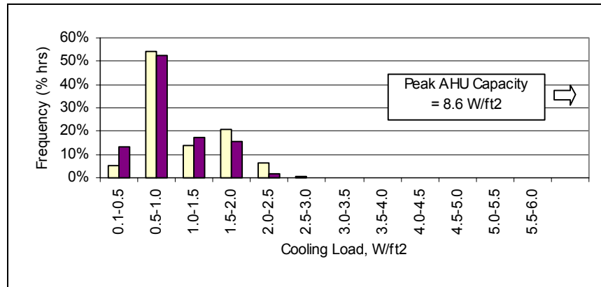
Figure 127. Site 1 (Dark bar includes Jan-May 2002 and Nov-Dec 2002, light bar covers Jun-Oct 2002)
