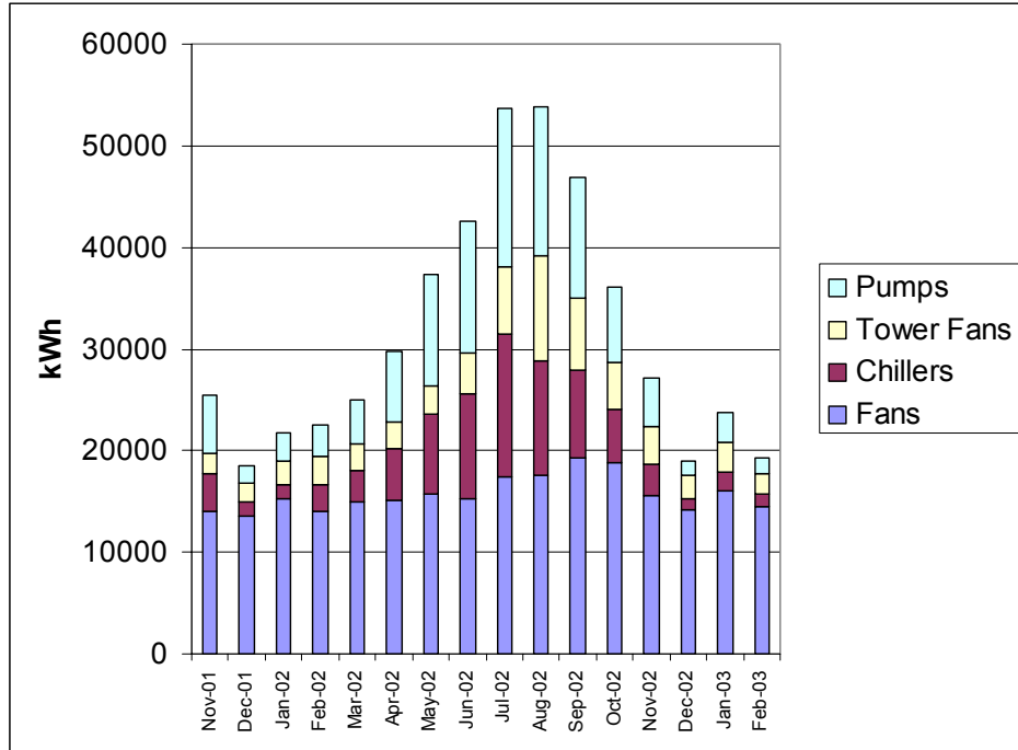
Figure 101. Site 1, Monitored HVAC Electricity End Uses
