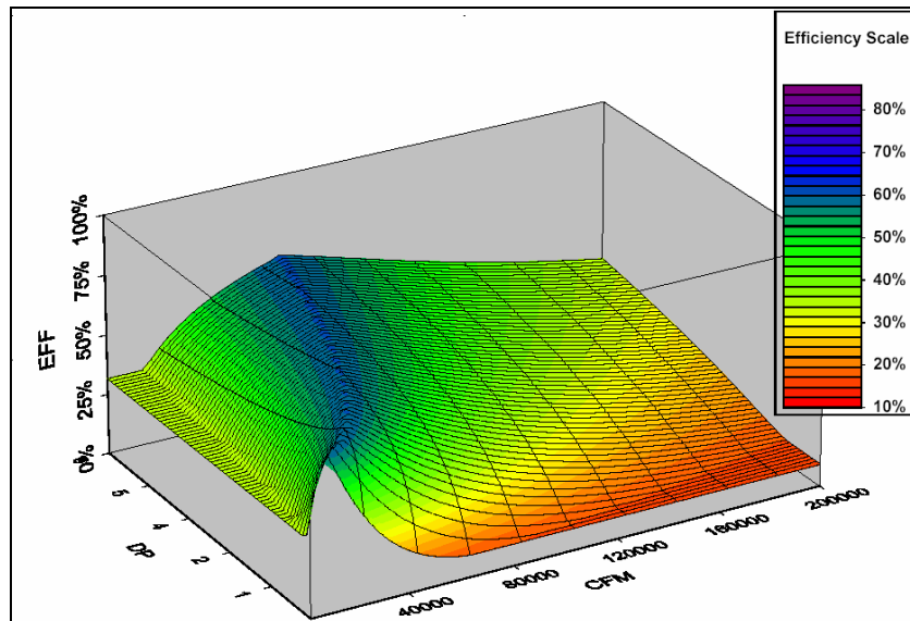
Figure 42. Three-Dimensional Fan Curve for 66" Plenum Airfoil Fan
