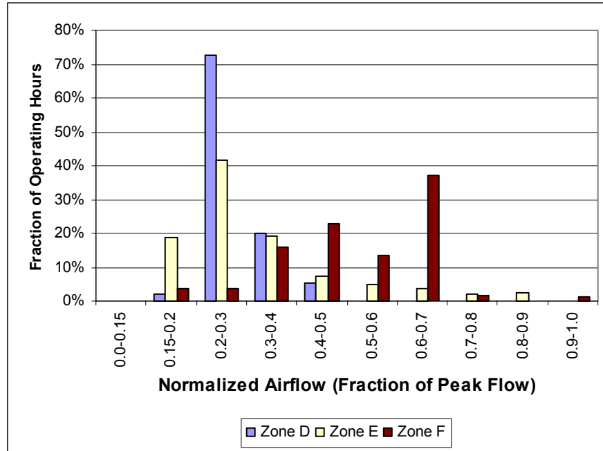
Figure 122. Site 4, Sample of Perimeter Zones (10/18/02-2/24/03)
