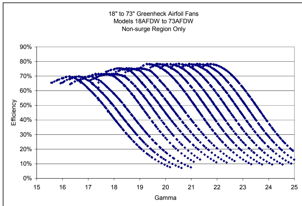
Figure 48. Gamma Curves for All Greenheck Housed Airfoil Fans (Non-Surge Region Only)
