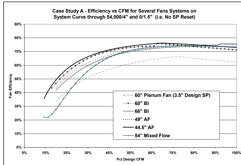
Figure 58. Case Study A - Part Load Fan Efficiency
