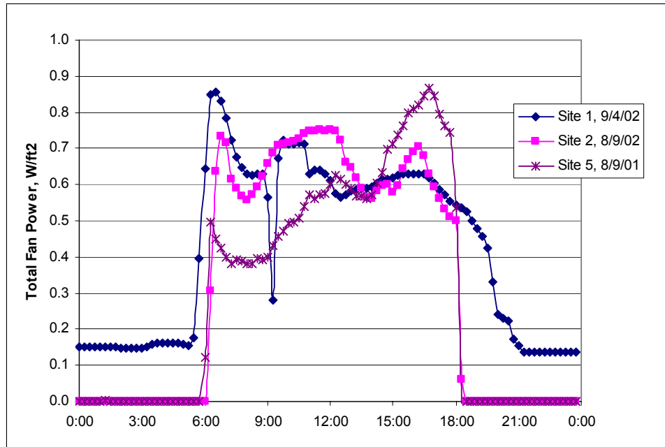
Figure 112. Peak Day Fan Electric Demand, Three Sites
