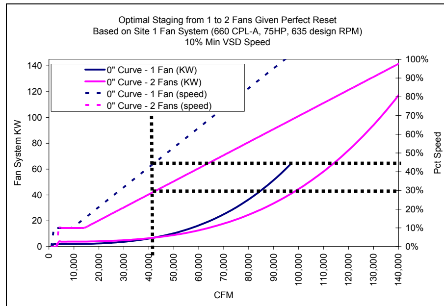
Figure 83. Optimal Staging (Perfect Static Pressure Reset)
