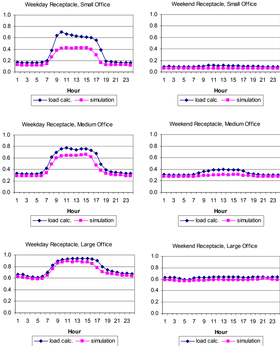
Figure 14. Measured Equipment Schedules (90 th percentile for design load calculations and 50 th percentile for energy simulations) for Small, Medium and Large Office Buildings – ASHRAE 1093-RP
