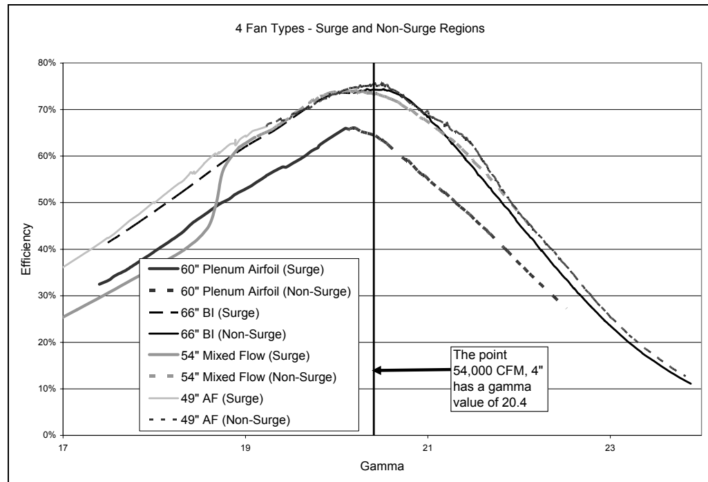
Figure 45. Gamma Curves for Four Fan Types
