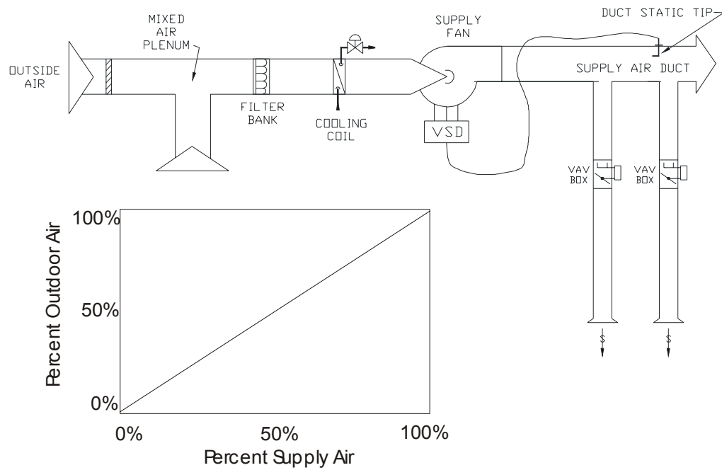
Figure 89. VAV Reheat System with a Fixed Minimum outdoor air Damper Setpoint
