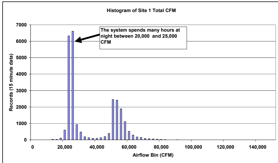
Figure 72. Case Study B - Histogram of CFM
