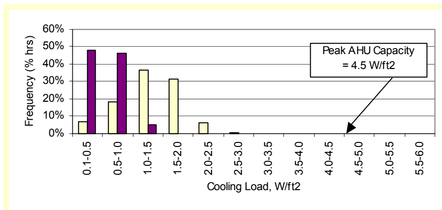
Figure 7. Measured Cooling Delivered by Air Handler, Site 3 (Light bar includes Aug-Oct 2002, dark bar covers Nov 2002 – Jan 2003)
