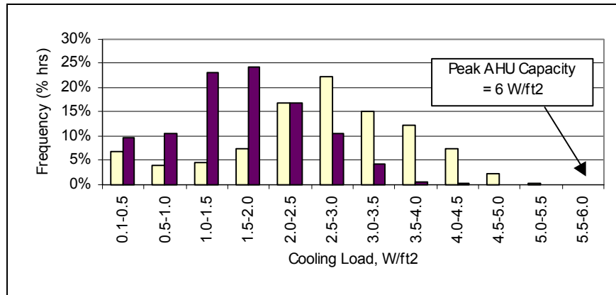
Figure 128. Site 2 (Light bar includes Jun-Oct 2002, dark bar covers Nov 2002 – Jan 2003)
