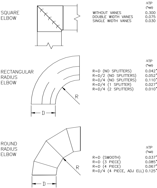
Figure 32. Pressure Drop Through Elbows
