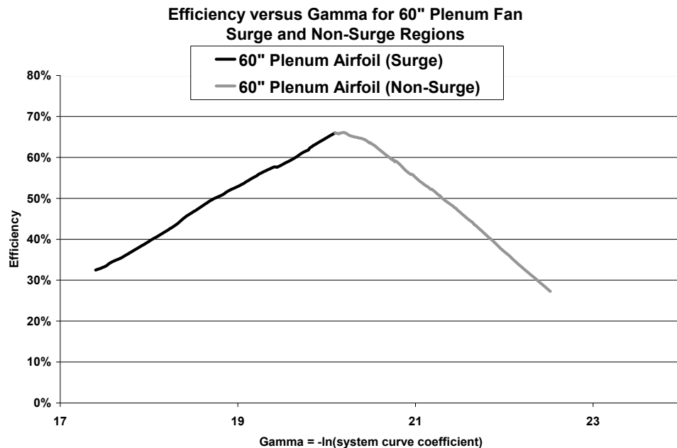
Figure 44. Gamma Curve
