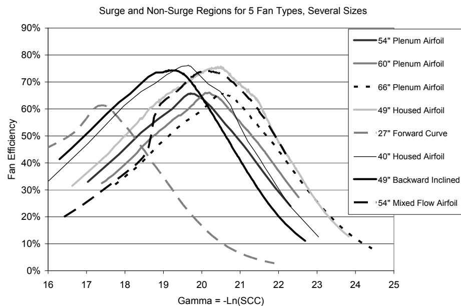
Figure 46. Gamma Curves for Several Fan Types and Sizes
