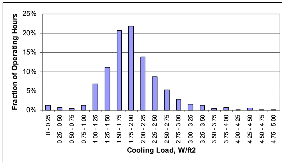
Figure 131. Monitored Sensible Cooling Load for an Air Handler Serving 19 Interior Zones, Site 4
