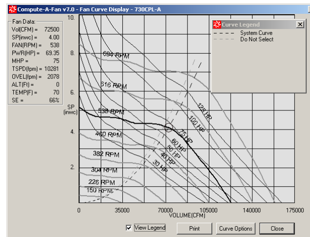
Figure 69. Case Study B - 73" Plenum Fan Curve
