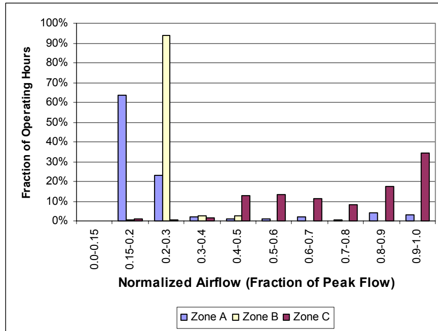
Figure 119. Site 4, Sample of Interior Zones (10/18/02-2/24/03)
