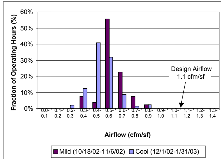
Figure 126. Total System Airflow, Site 4
