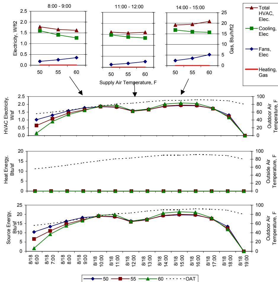
Figure 38. Comparison of Hot Day Simulation Results for Three Supply Air Temperature Setpoints: 50°F, 55°F, and 60°F. August 18, Sacramento Climate.
