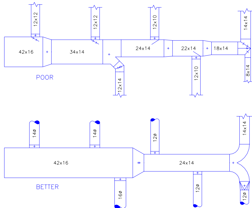
Figure 31. Examples of Poor and Better Duct Design
