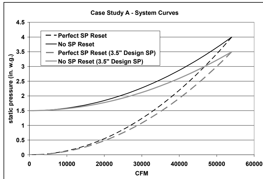
Figure 56. Case Study A - System Curves
