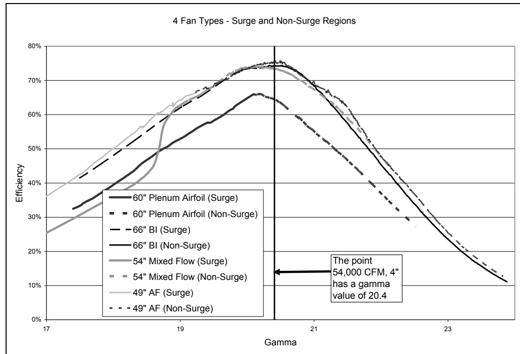
Figure 61. Case Study A - Gamma Curves
