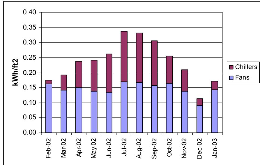
Figure 116. Comparison of Fan and Chiller Energy at Site 2 (Cumulative Graph, e.g. Combined Total is 0.34 kWh/ft²-yr in July)
