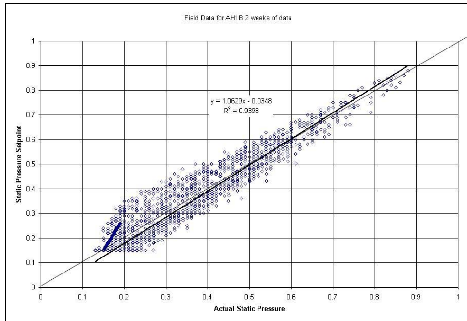
Figure 81. Monitored Data Illustrating Static Pressure Reset
