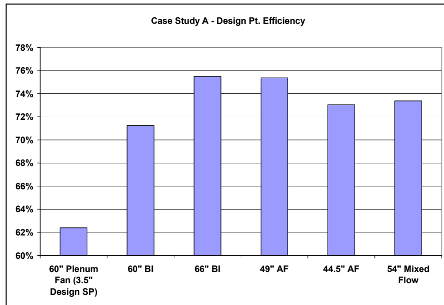
Figure 57. Case Study A - Design Point Efficiency
