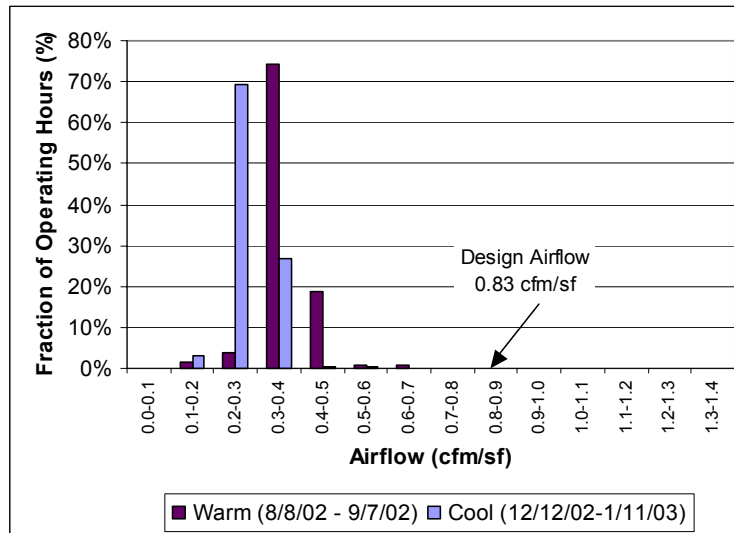
Figure 125. Total System Airflow, Site 3
