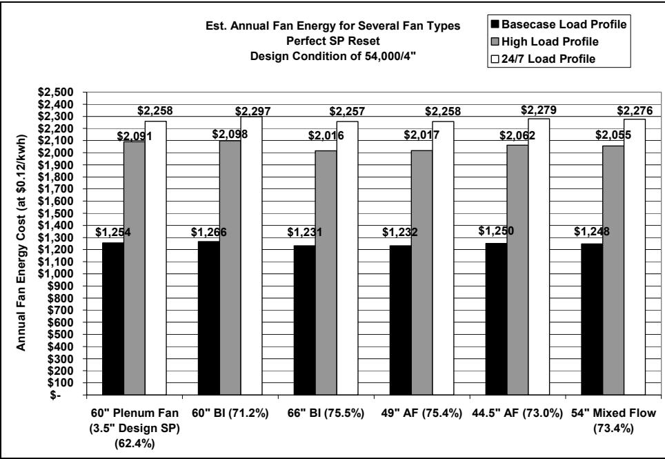
Figure 63. Case Study A Results - Perfect Static Pressure Reset
