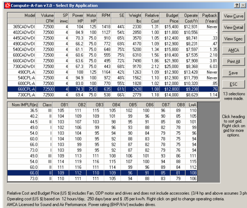
Figure 68. Case Study B - Selection Software Airfoil and Plenum Fans
