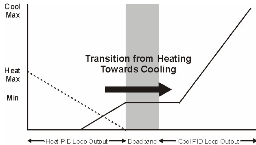
Figure 30. Dual Duct Mixing - From Heating to Cooling
