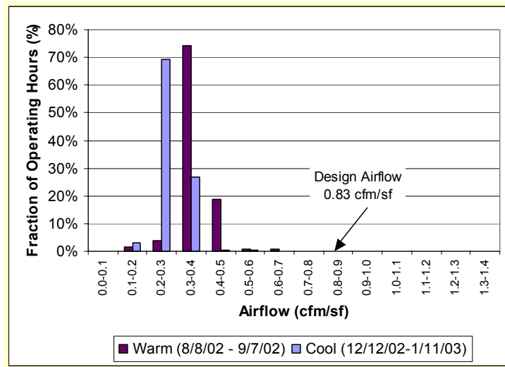
Figure 6. Measured System Airflow, Site 3
