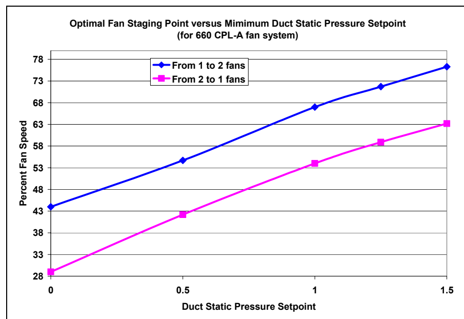
Figure 84. Optimal Staging Point vs. Minimum Duct Static Pressure Setpoint
