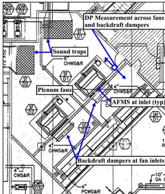
Figure 76. Plan View of Site 1 Air Handler
