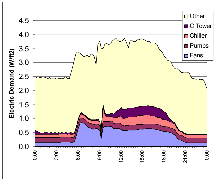
Figure 113. Peak Day Electric Demand, Site 1, 9/3/2002 (Cumulative Graph; Total Peak is 3.9 W/ft²)
