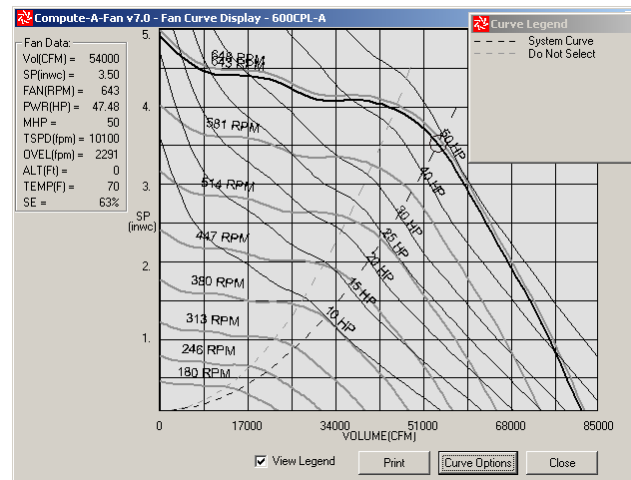
Figure 55. Case Study A - 60" Plenum Fan Design Point
