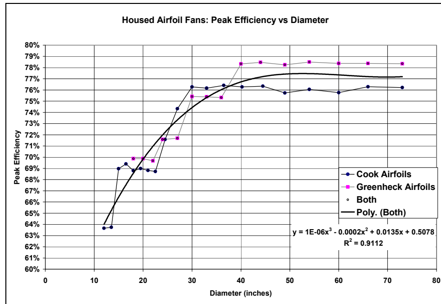
Figure 79. Peak Efficiency of Cook vs Greenheck Housed Airfoil Fans
