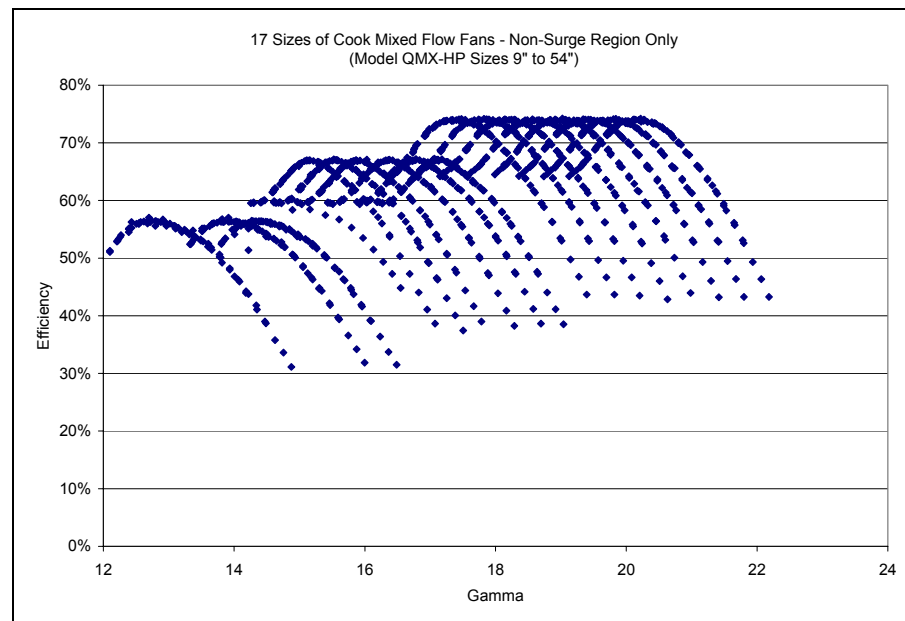
Figure 50. Gamma Curves for All Cook Airfoil Mixed Flow Fans
