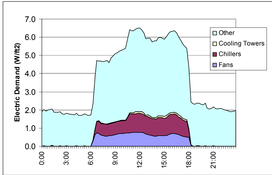
Figure 114. Peak Day Electric Demand, Site 2, 8/9/2002 (Cumulative Graph; Total Peak is 6.4 W/ft 2 )
