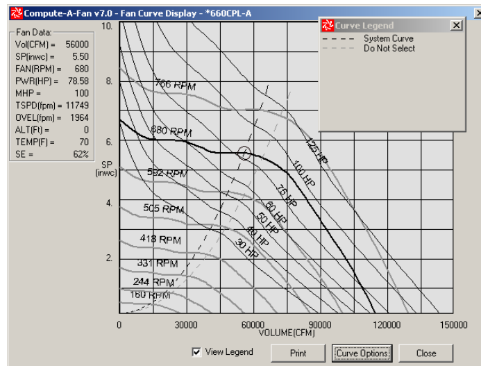
Figure 87. "Paralleling" - High Flow
