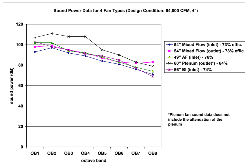
Figure 65. Case Study A - Acoustic Data (No Casing)
