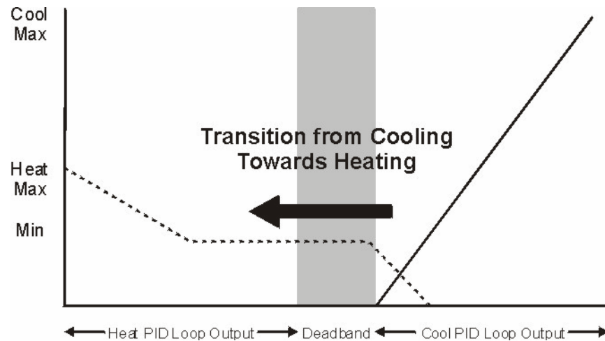
Figure 29. Dual Duct Mixing - From Cooling to Heating
