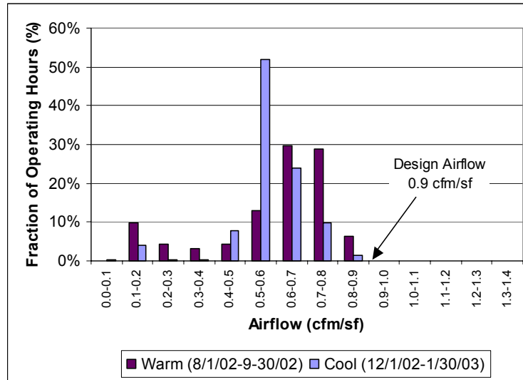
Figure 124. Total System Airflow, Site 2
