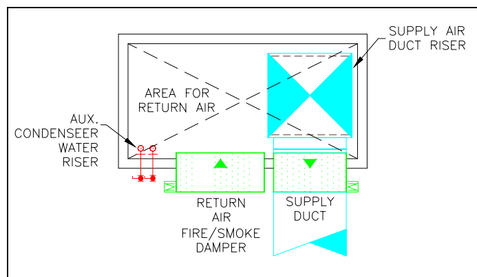
Figure 8. Typical Duct Shaft with Unducted Return
