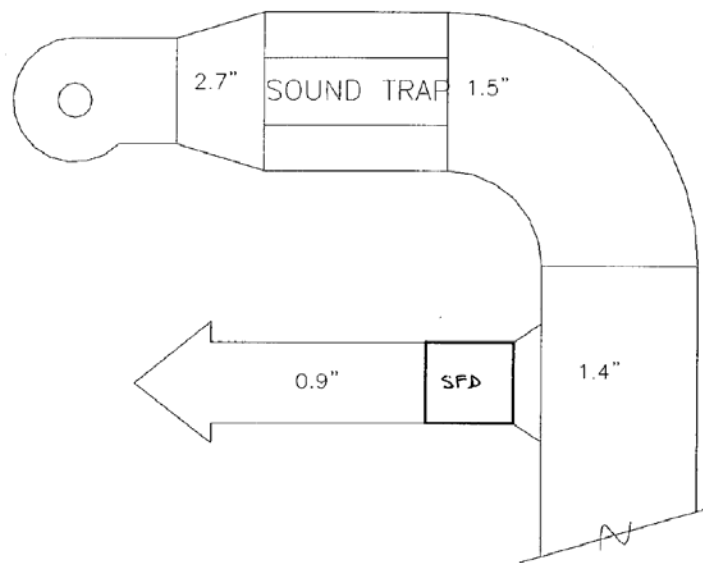
Figure 37. Measured Pressure in a System with Significant Fan and Duct System Effect
