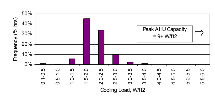
Figure 130. Site 4 (Dark bar includes Nov. 25, 2002 - Feb. 24, 2003)
