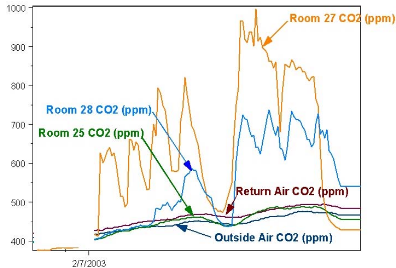
Figure 20. Measured CO 2 Levels At Site #4 on February 7 th , 2003
