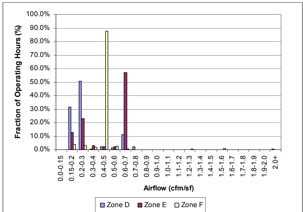
Figure 121. Site 3, Sample of Perimeter Zones, Cool Period (12/12/02 - 1/11/03)
