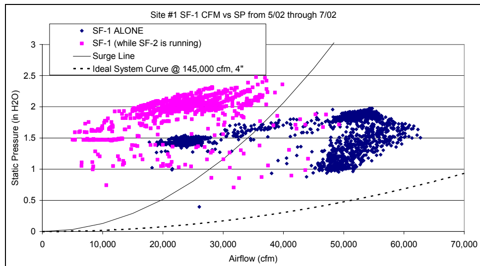
Figure 86. Parallel Fans in Surge
