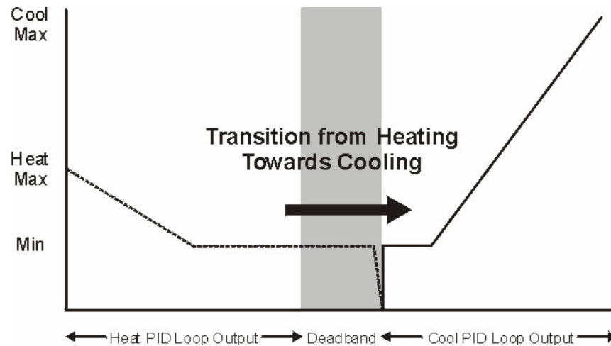
Figure 28. Dual Duct - From Heating to Cooling
