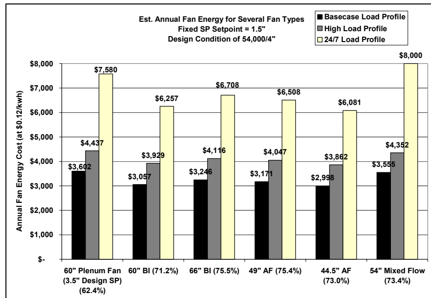
Figure 64. Case Study A Results – No Static Pressure Reset
