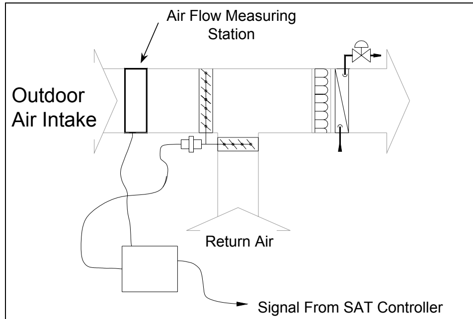
Figure 92. Airflow Measurement of 100% outdoor air
