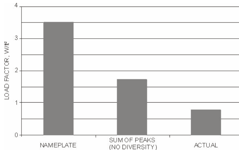
Figure 13. Office Equipment Load Factor Comparison – Wilkins, C.K. and N. McGaffin. ASHRAE Journal 1994 - Measuring computer equipment loads in office buildings
