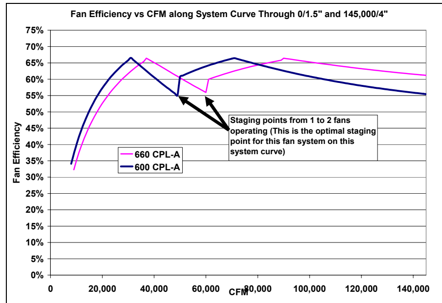
Figure 73. Case Study B – Part Load Fan Efficiency
