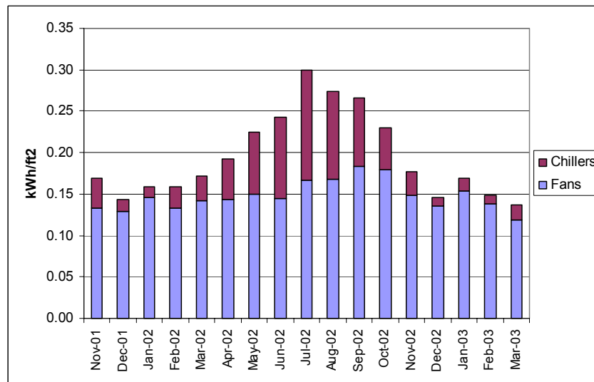
Figure 115. Comparison of Fan and Chiller Energy at Site 1 (Cumulative Graph, e.g. Combined Total is 0.30 kWh/ft 2 -yr in July)
