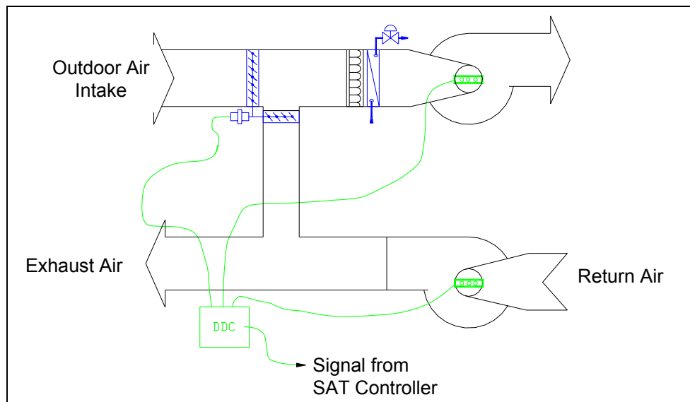
Figure 91. Return Fan Tracking
