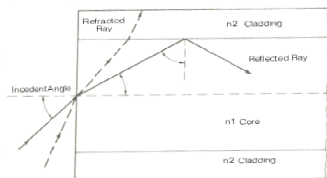
Fig. 2: Total internal reflection between 2 dielectric mediums
