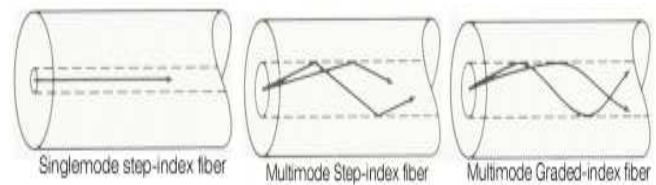
Fig. 3: Optical Fibre
