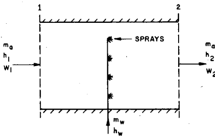
Fig. A6.11 Typical Spray Chamber
