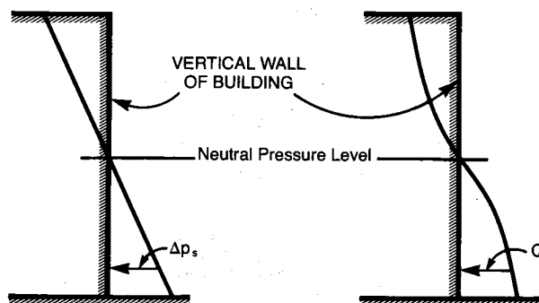
Fig. A5.3 Diagram Showing Linear Distribution of \Delta p_s and Non-Linear Distribution of Q for Winter Conditions
