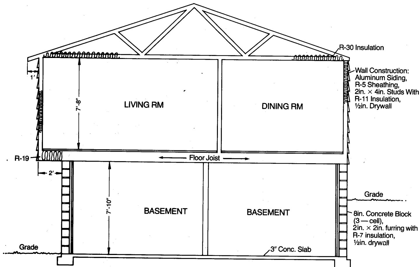
Fig. 7.5 Elevation for Residence of Example 7.4.
