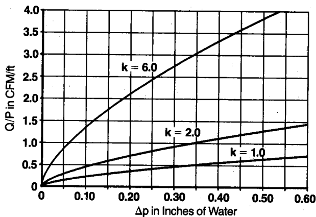
Fig. 5.11 Window and Residential Type Door Infiltration Characteristics
