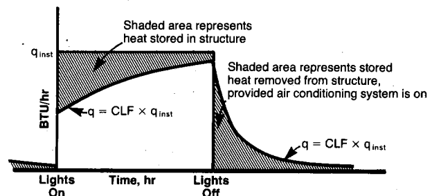
Fig. A4.1 The Effect of Thermal Storage on the Cooling Load Due to Lights
