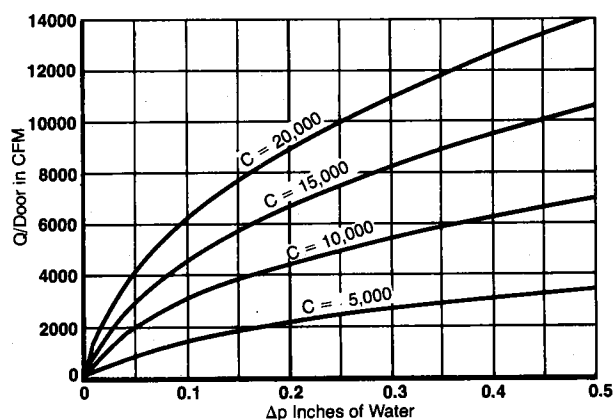
Figure 5.14 Swinging Door Infiltration Characteristics with Traffic
