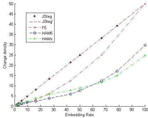
Fig. 3. A comparison between HAM algorithm and DEA, Jsteg and F5 algorithm
