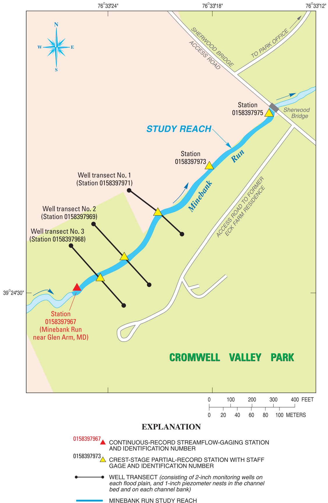
Figure 12b. General layout of the Minebank Run study reach for hydrologic data collection.
