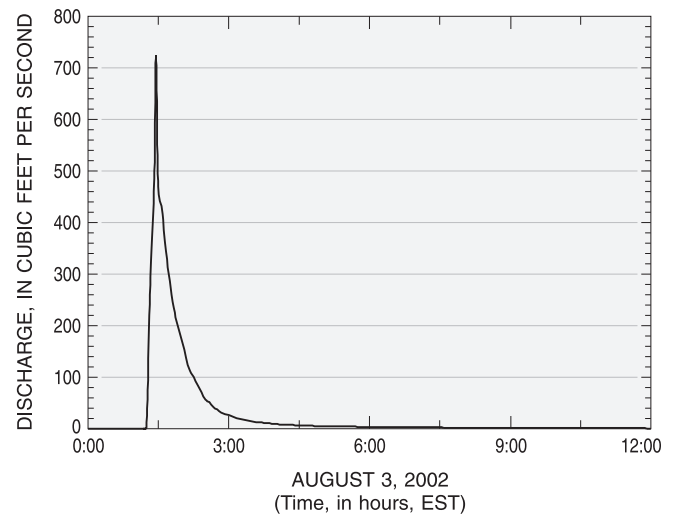
Figure 19. Discharge hydrograph for U.S. Geological Survey station 0158397967, Minebank Run near Glen Arm, Maryland, for the storm of August 3, 2002.
