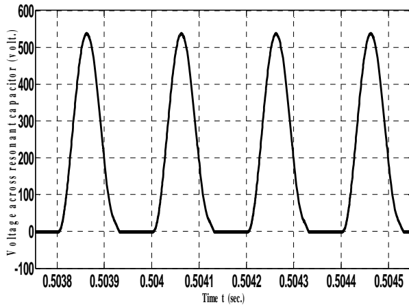
Figure: (b) Voltage across resonant capacitor (Cr).
