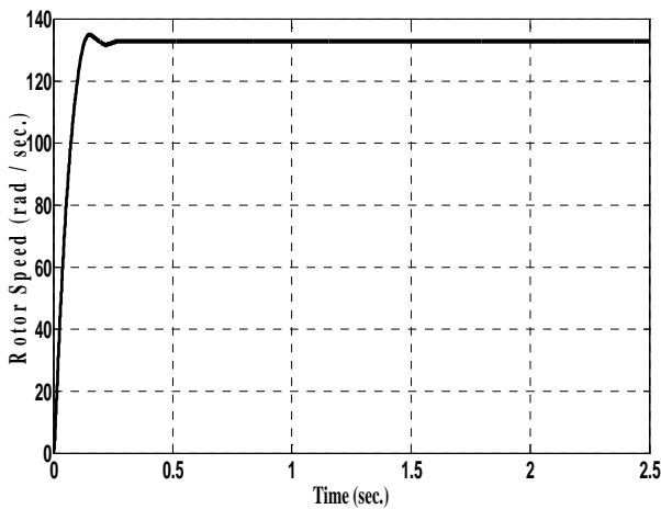
Figure: (c) Rotor speed \omega_m (rad / sec.)
