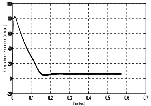
Figure: (e) Armature current I_a (Amp.).
