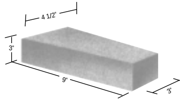
9 Inch No. 3 Key 9 X (4½ – 3) X 3
