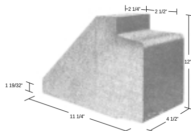
Shape No. 60-12-C For Arch 12 Inches Thick
