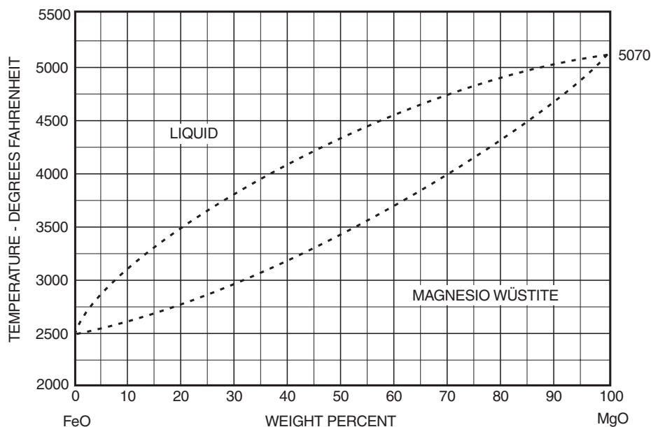
Figure 5 Equilibrium Diagram of the system FeO•MgO
