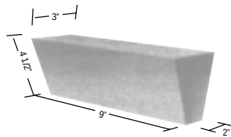
9 Inch No. 3 Arch 9 X 4½ X (3 – 2)
