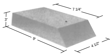
9 Inch – 60° End Skew (9 – 7¼) X 4½ X 3
