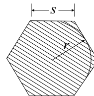
REGULAR POLYGON
