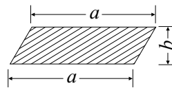
PARALLELOGRAM
