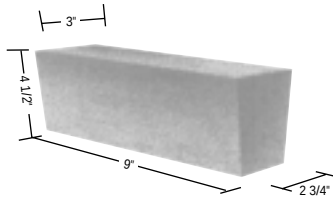
9 Inch No. 1 Arch 9 X 4½ X (3 – 2¾)
