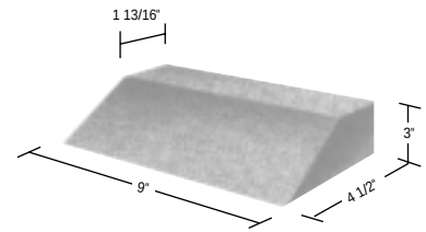
9 Inch – 48° Side Skew 9 X (4½ – 1⅓) X 3
