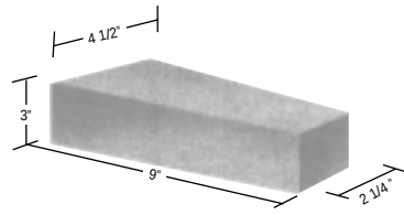
9 Inch No. 4 Key 9 X (4½ – 2¼) X 3
