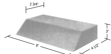
9 Inch – 60° Side Skew 9 X (4½ – 2¾) X 3
