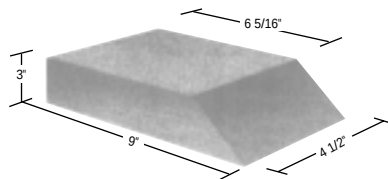
9 Inch – 48° End Skew (9 – 6⅝) X 4½ X 3
