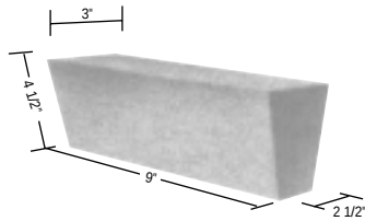
9 Inch No. 2 Arch 9 X 4½ X (3 – 2½)
