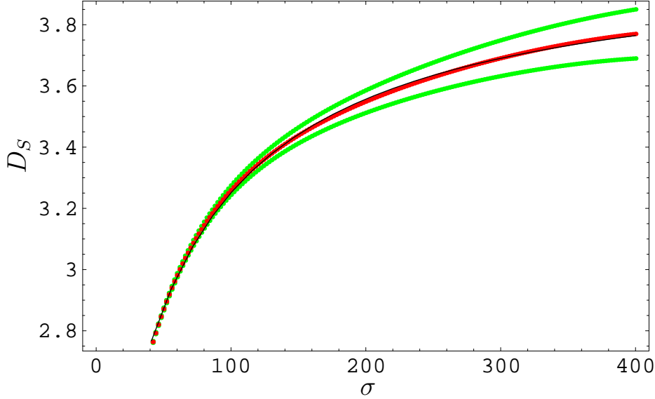
Figure 4: The spectral dimension D_S of the universe as function of the diffusion time \sigma , measured for \kappa_0 = 2.2 , \Delta = 0.6 and t = 80 , and a spacetime volume N_4 = 181k . The averaged measurements lie along the central curve, together with a superimposed best fit D_S(\sigma) = 4.02 - 119/(54 + \sigma) (thin black curve). The two outer curves represent error bars.
