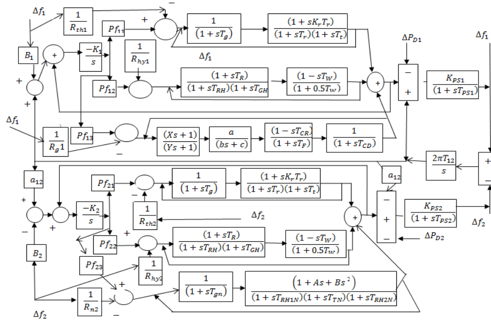
Figure 5. Complete Transfer function Block Diagram of Multi Generating Interconnected Power System.
