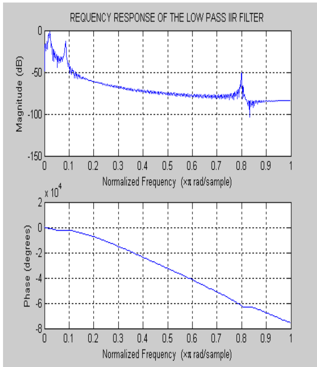
Figure 4: Frequency response (magnitude and phase ) of filter
